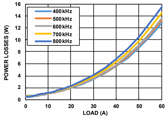
FIGURE 11. ISL99227, ISL99227B POWER DISSIPATION ( V_{IN} = 12V ; V_{OUT} = 1.8V ; L_{OUT} = 0.18\mu H/0.17m\Omega/FP1008-180-R )
