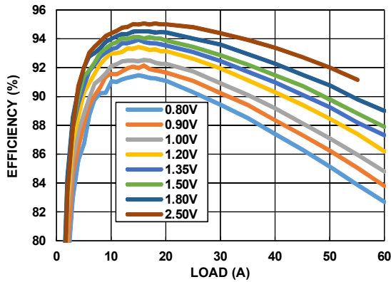
FIGURE 8. POWER STAGE EFFICIENCY ( V_{IN} = 12V ; f_{SW} = 500kHz ; L_{OUT} = 0.18\mu H/0.17m\Omega/FP1008-180-R ; INCLUDE INDUCTOR AND ISL99227, ISL99227B LOSSES)
