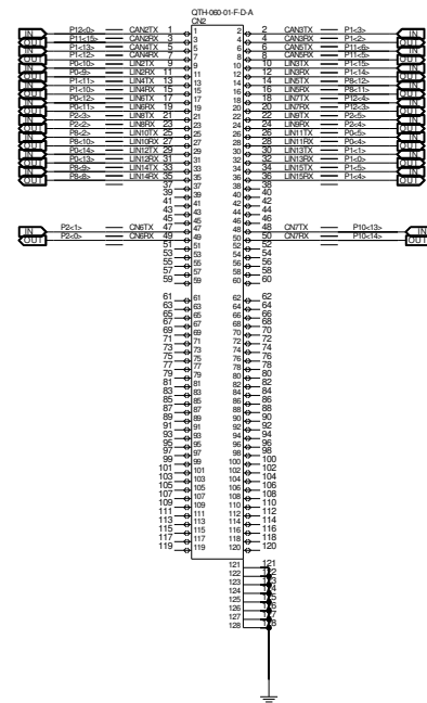
CONNECTOR2
