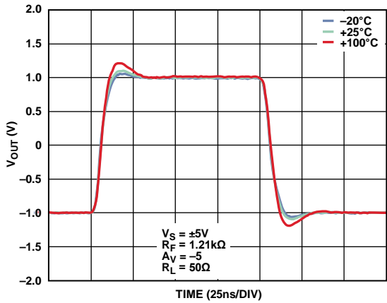
Figure 41. Small Signal Pulse Response vs. Case Temperature, A_V = -5 , V_S = \pm 5\text{ V} , V_{OUT} = 2\text{ V p-p} , R_F = 1.21\text{ k}\Omega , R_L = 50\ \Omega
