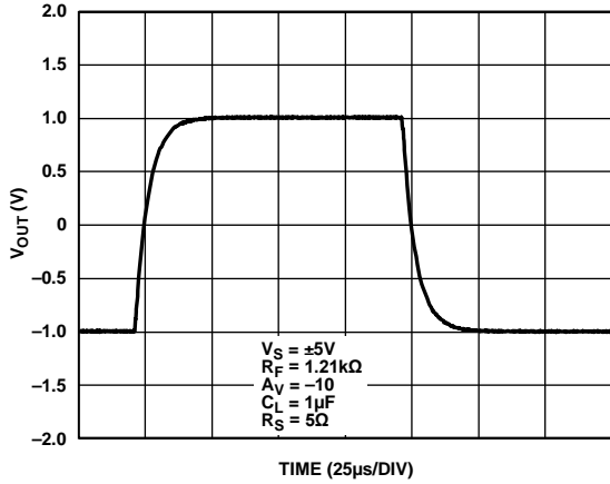
Figure 40. Small Signal Pulse Response, A_V = -10 , V_S = \pm 5\text{ V} , V_{OUT} = 2\text{ V p-p} , R_F = 1.21\text{ k}\Omega , C_L = 1\ \mu\text{F} , R_S = 5\ \Omega
