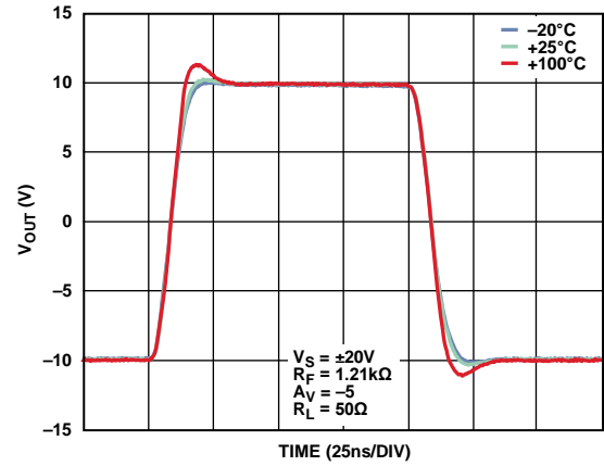
Figure 44. Large Signal Pulse Response vs. Case Temperature, A_V = -5 , V_S = \pm 20\text{ V} , V_{OUT} = 20\text{ V p-p} , R_F = 1.21\text{ k}\Omega , R_L = 50\ \Omega
