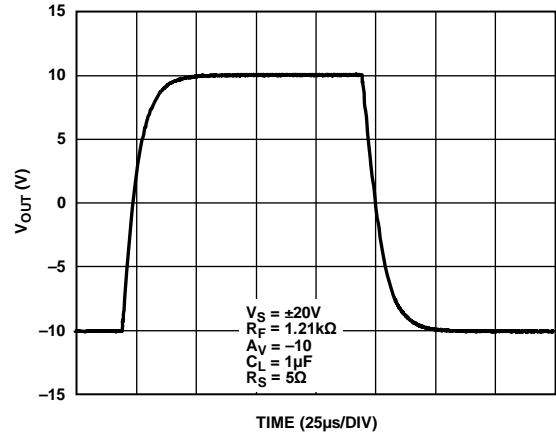
Figure 43. Large Signal Pulse Response, A_V = -10 , V_S = \pm 20\text{ V} , V_{OUT} = 20\text{ V p-p} , R_F = 1.21\text{ k}\Omega , C_L = 1\ \mu\text{F} , R_S = 5\ \Omega
