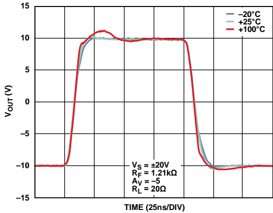
Figure 42. Large Signal Pulse Response vs. Case Temperature, A_V = -5 , V_S = \pm 20\text{ V} , V_{OUT} = 20\text{ V p-p} , R_F = 1.21\text{ k}\Omega , R_L = 20\ \Omega
