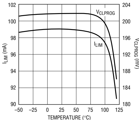
Input Current Limit vs Temperature (Low Power)
