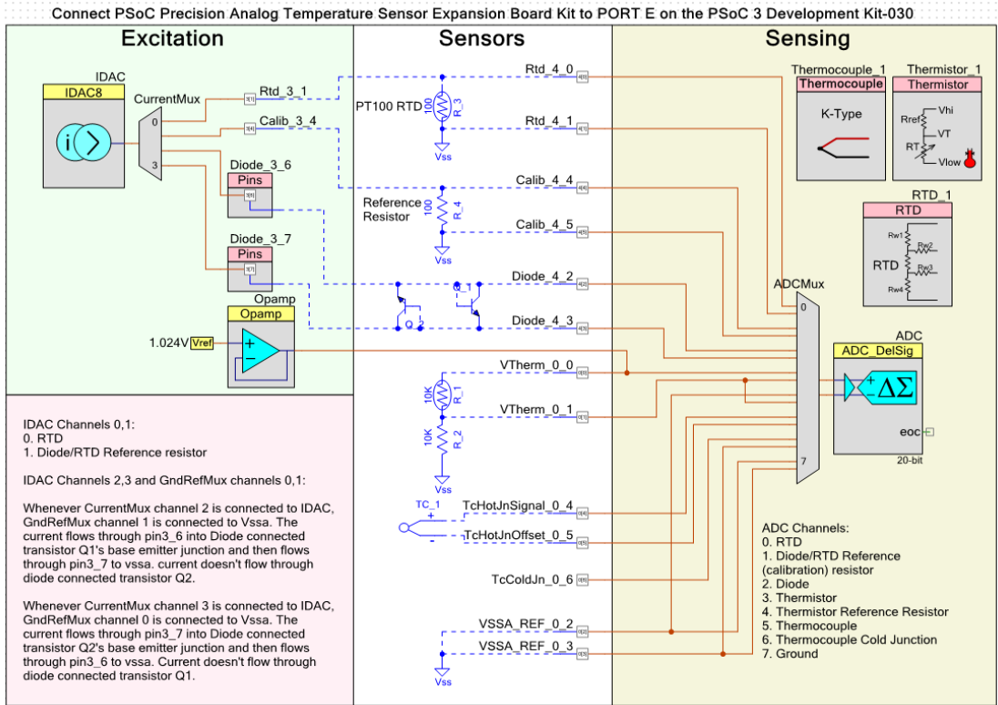
Figure 5-5. PSoC Creator Top Design
