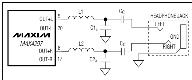
Figure 7. Headphone Application Circuit
