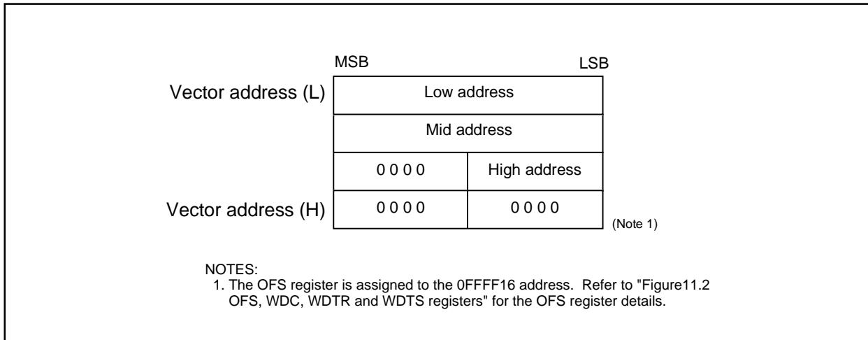
Figure 10.2 Interrupt Vector
