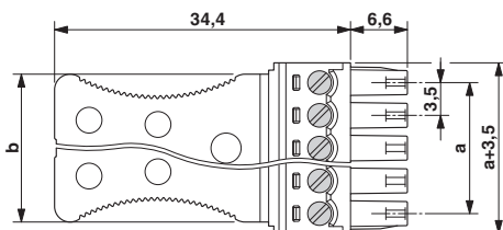
Dimensioned drawing
