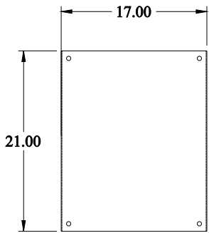
INNER PANEL
