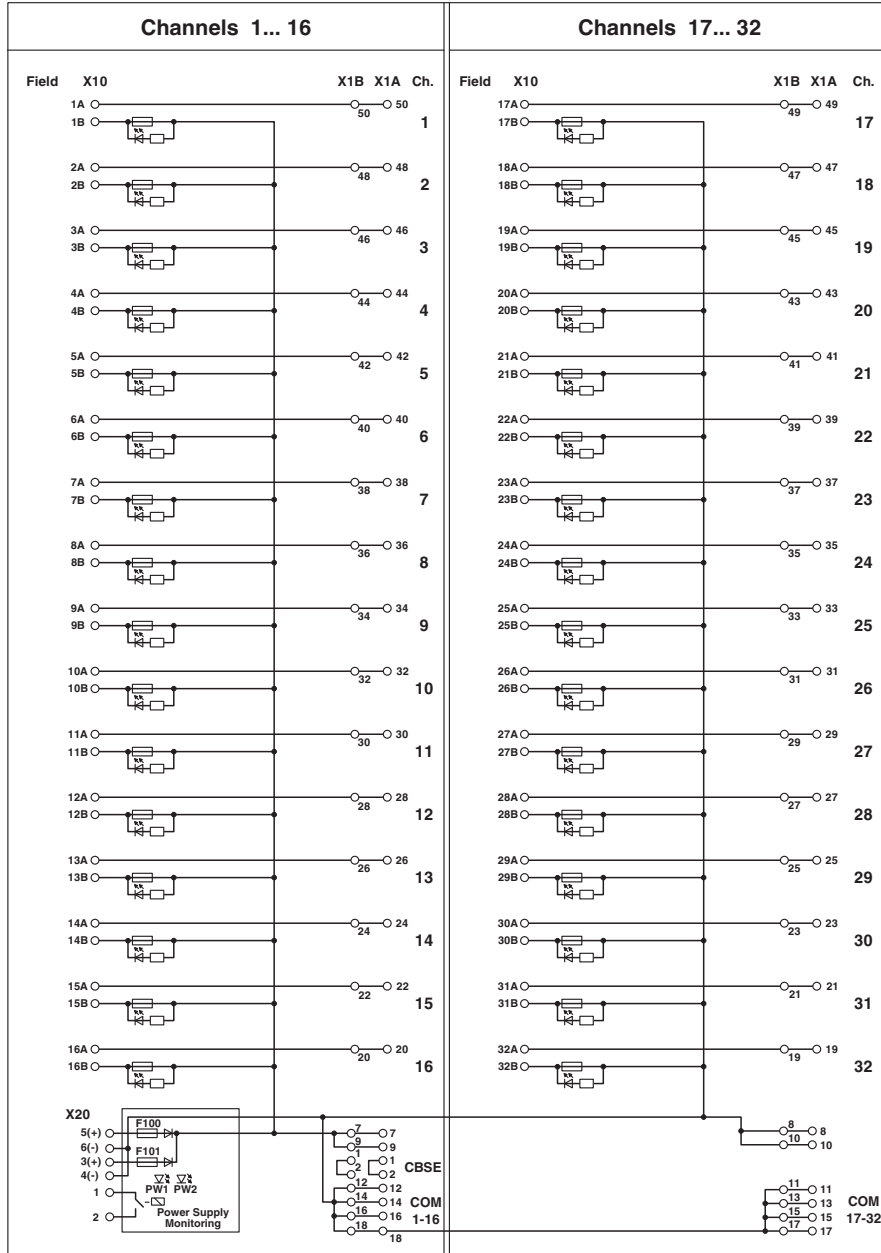
Circuit diagram
