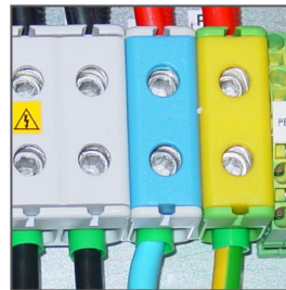
Motor Drive
