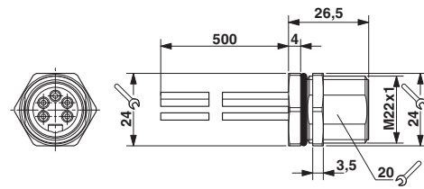
7/8" flush-type plug
