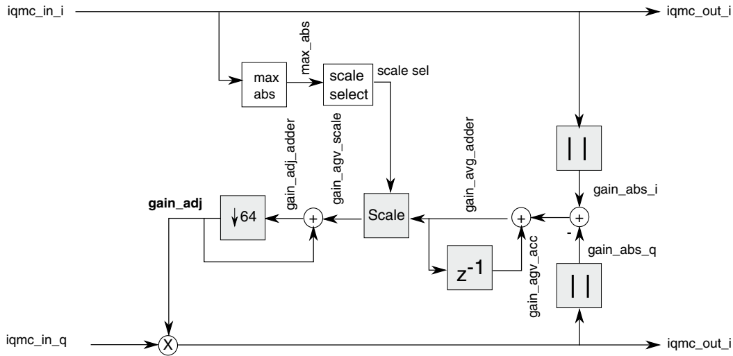
Figure 45-29. I/Q Gain Mismatch Calibration Block Diagram
