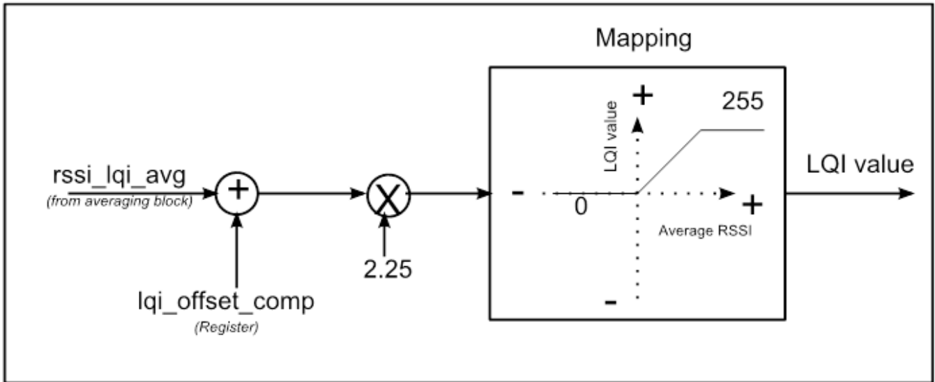
Figure 45-85. LQI Computation
