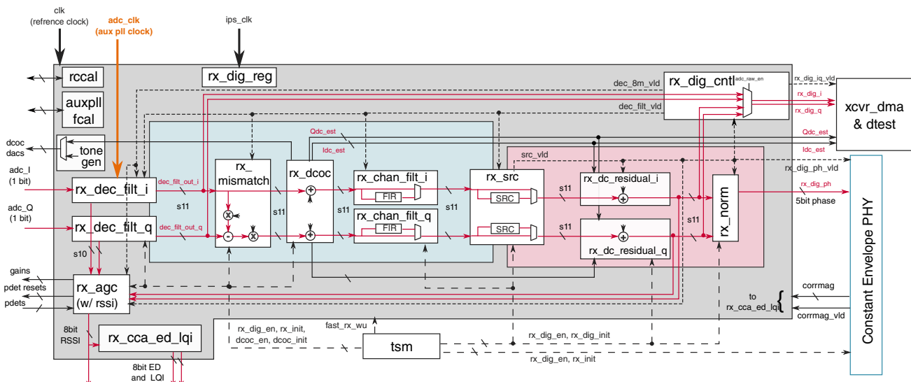
Figure 45-20. RX DIG Block diagram
