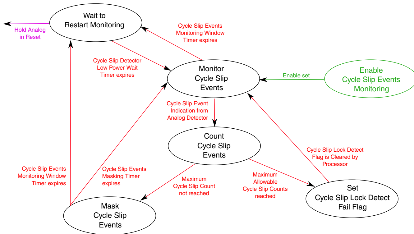
Figure 45-17. PLL Lock Detect State Machine
