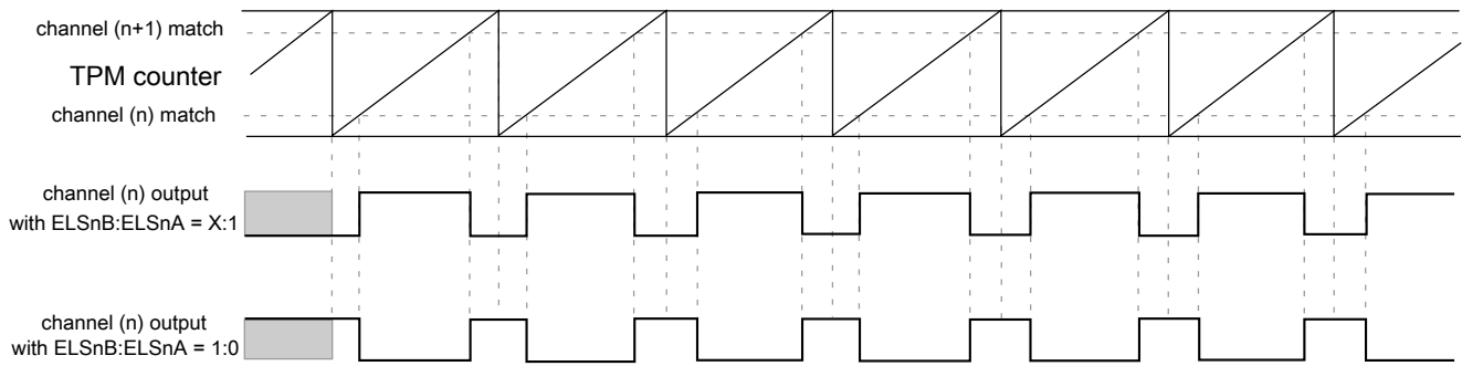
Figure 33-15. Combine mode
