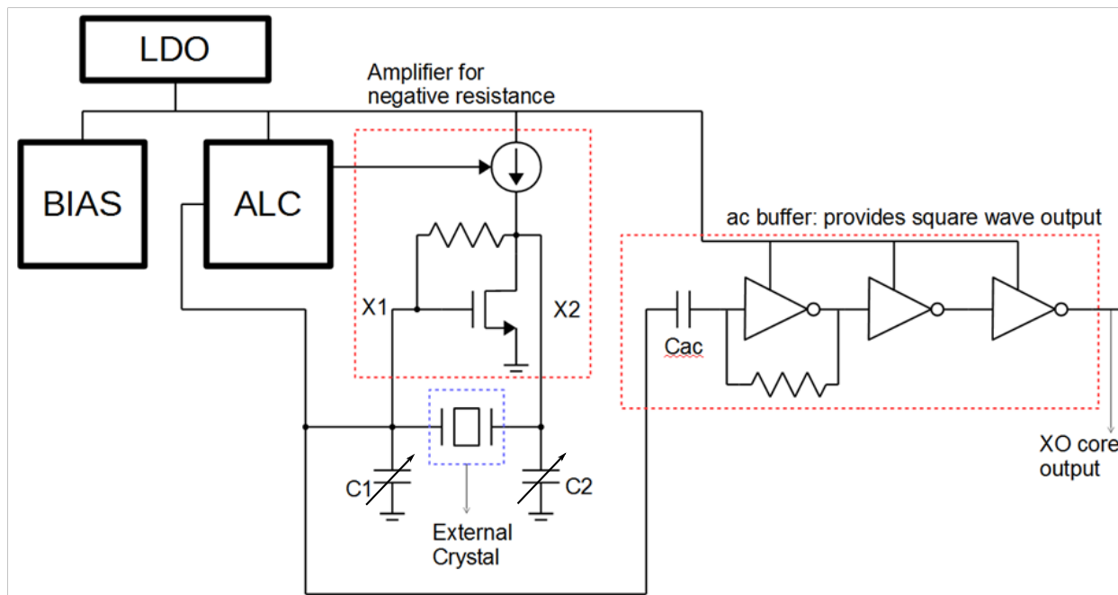
Figure 45-67. XO circuit diagram
