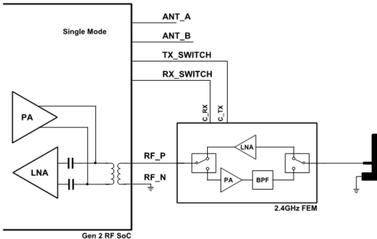
Figure 45-96. FEM Interface Single Antenna Configuration
