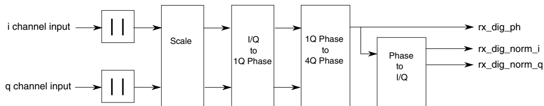
Normalizer Block Diagram
