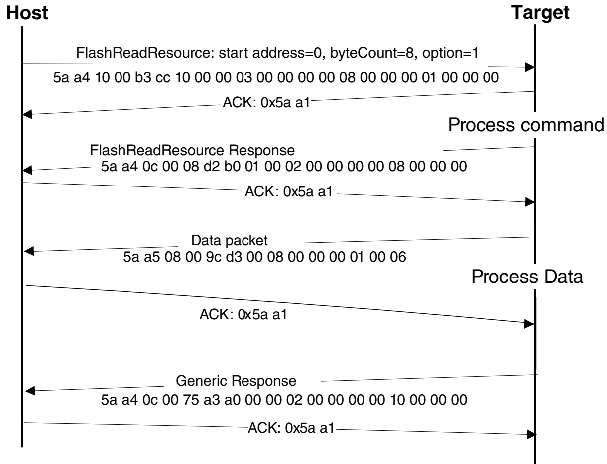
Figure 7-16. Protocol Sequence for FlashReadResource Command
