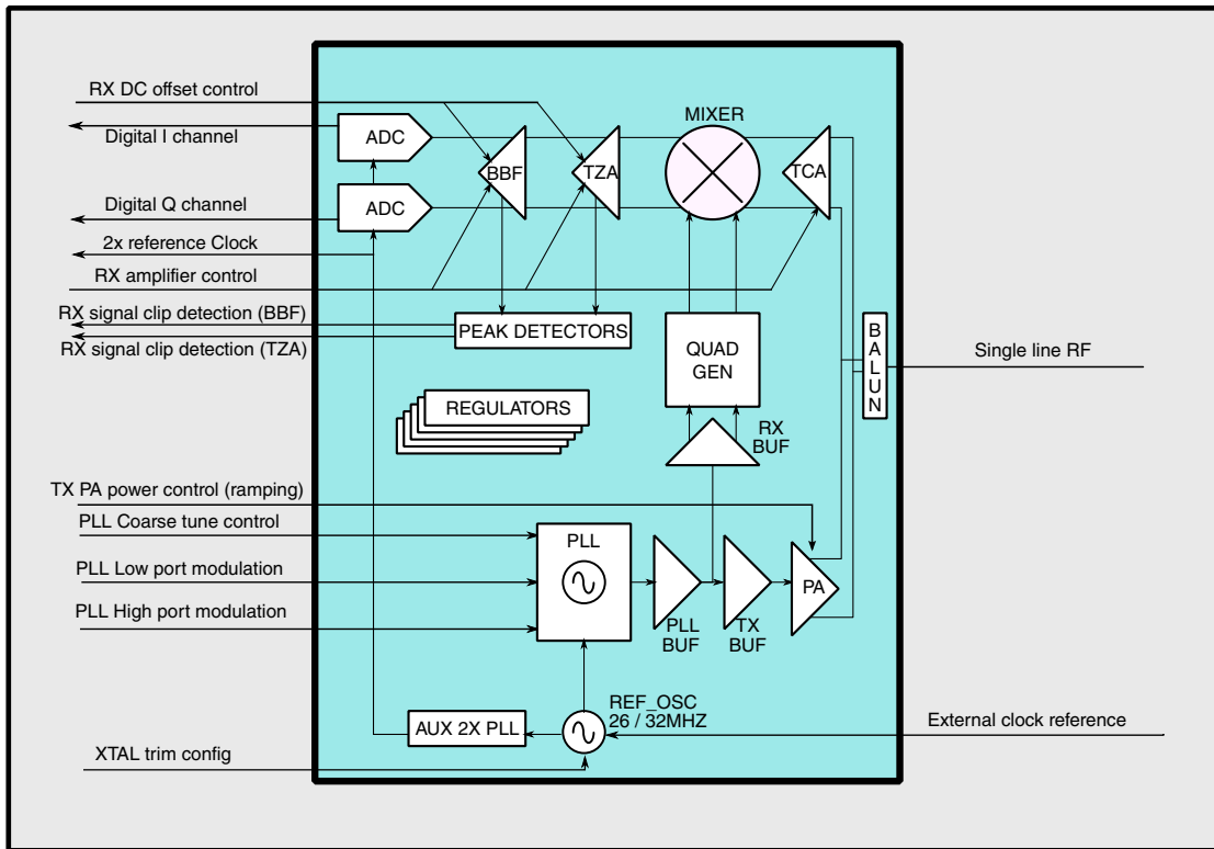
Figure 45-66. Analog Radio Block diagram
