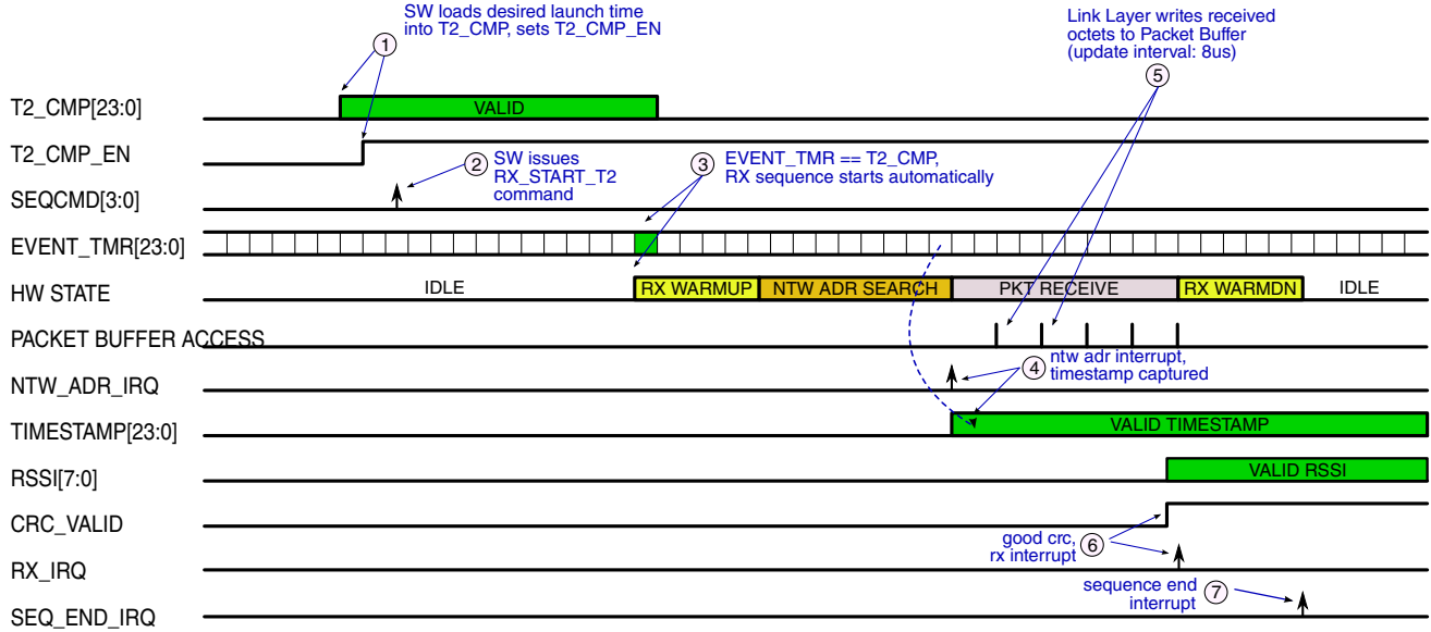
Figure 45-128. GENERIC FSK RX SEQUENCE: LAUNCH VIA T2 TIMER, GOOD PACKET
