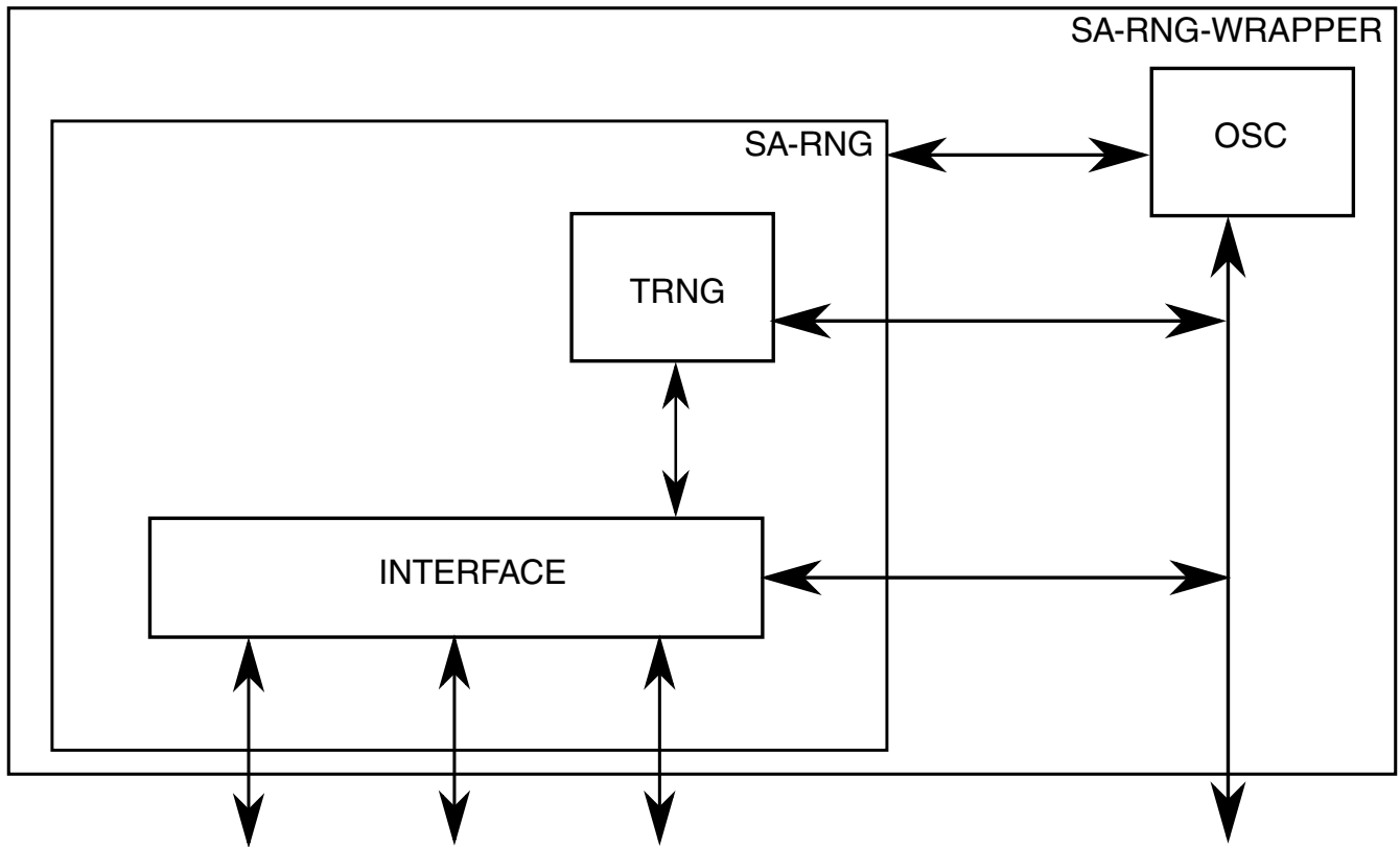
Figure 44-1. SA TRNG Block Diagram
