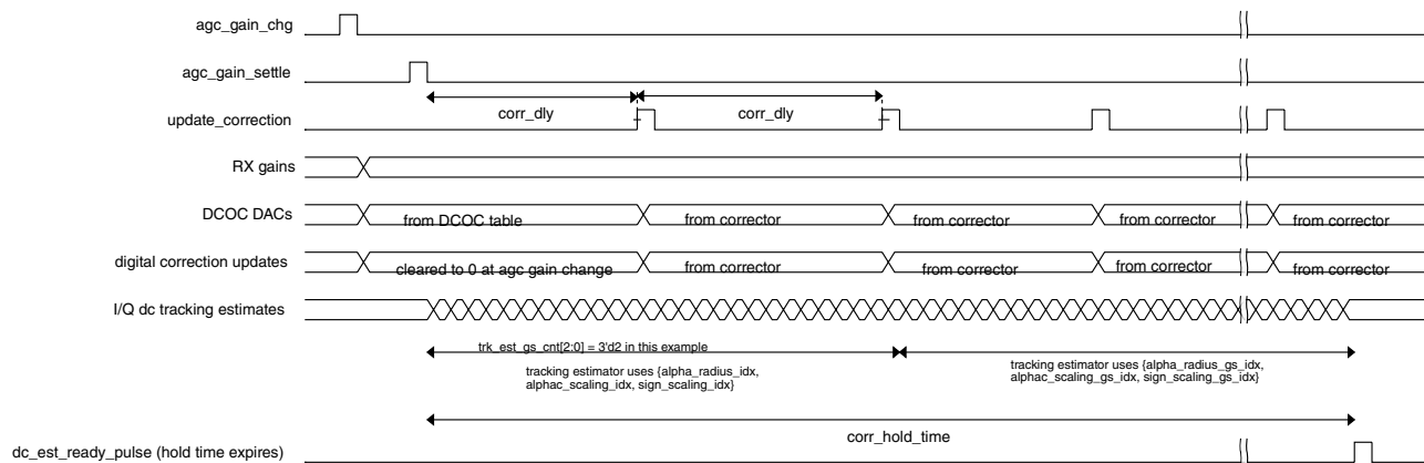
Figure 45-39. DC Offset Tracking Correction Timing
