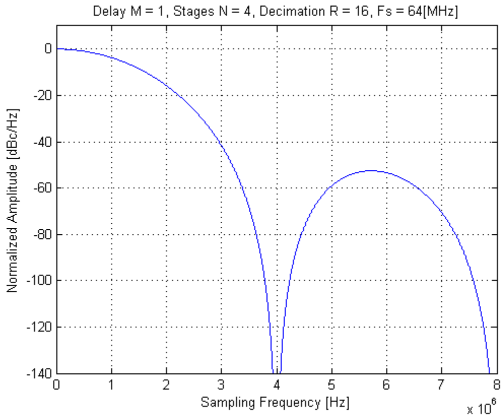
Figure 45-23. 4th order CIC (OSR=16) Decimation Filter Frequency Response
