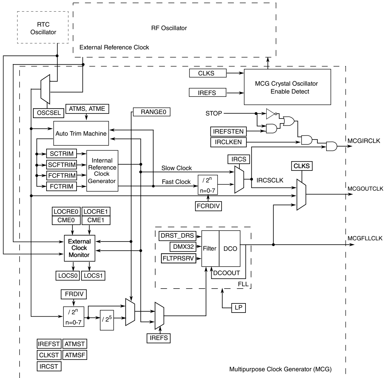
Figure 25-1. Multipurpose Clock Generator (MCG) block diagram
