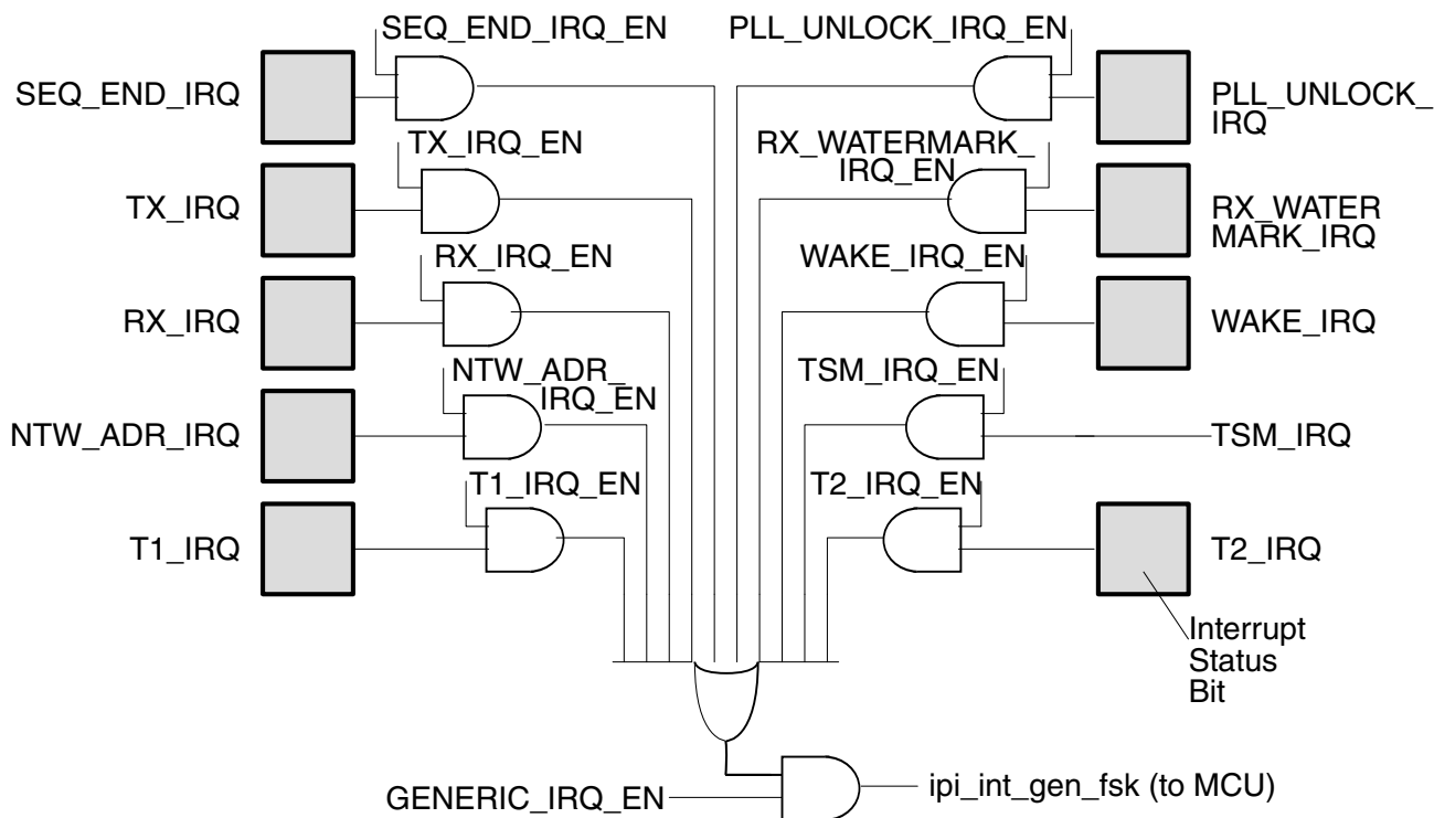
Figure 45-125. GENERIC_FSK Interrupt Architecture
