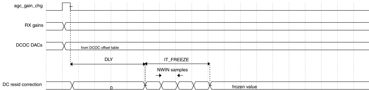
Figure 45-40. DC residual mode 1 timing
