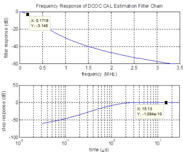
Figure 45-36. Magnitude and Step response of DC Offset Calibration Estimator
