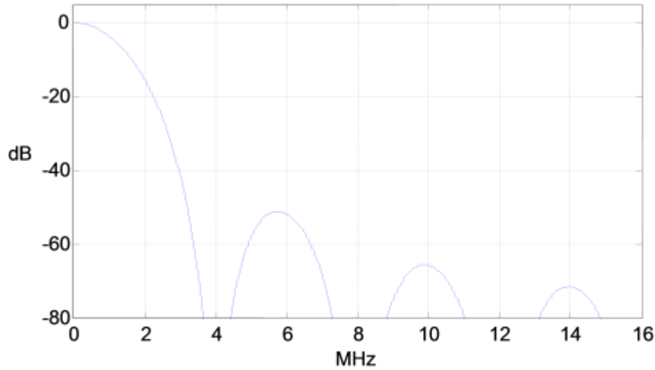
Figure 45-22. 4th order CIC (OSR=8) Decimation Filter Frequency Response
