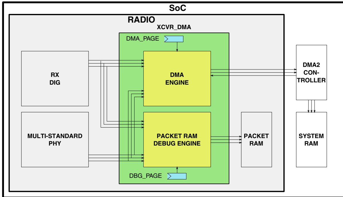
Figure 45-63. Transceiver DMA and Packet RAM Debug
