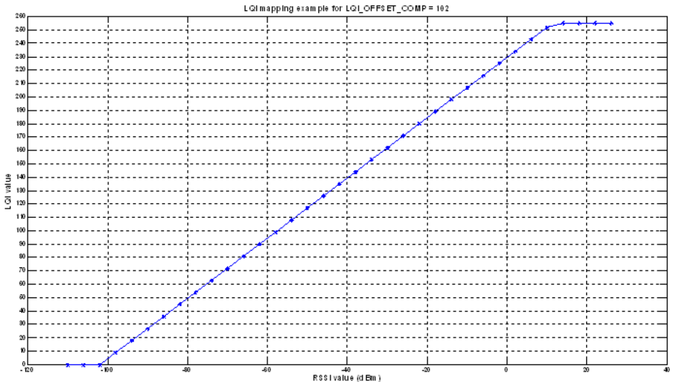
Figure 45-86. Plot of LQI vs. RSSI
