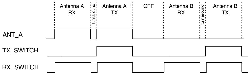
Figure 45-92. FAD Single Mode Timing
