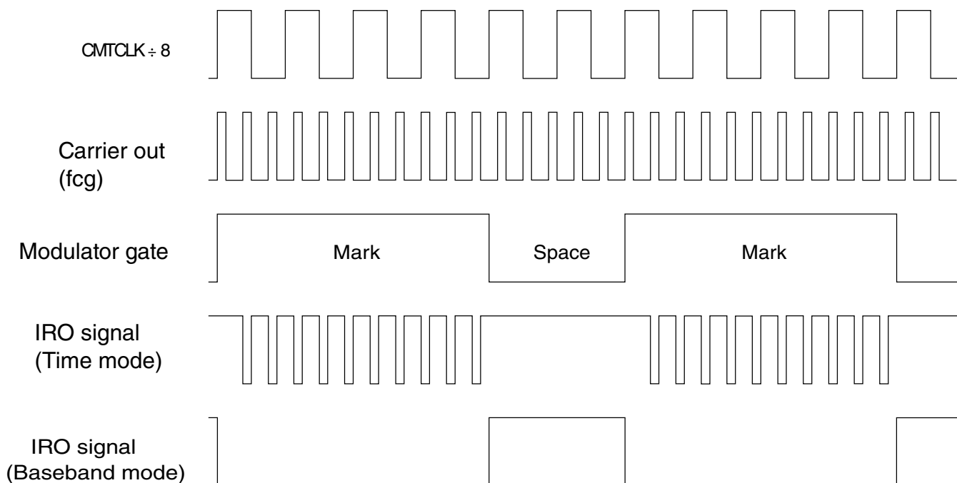
Figure 40-5. Example: CMT output in Time and Baseband modes with \text{OC}[\text{CMTPOL}] = 0
