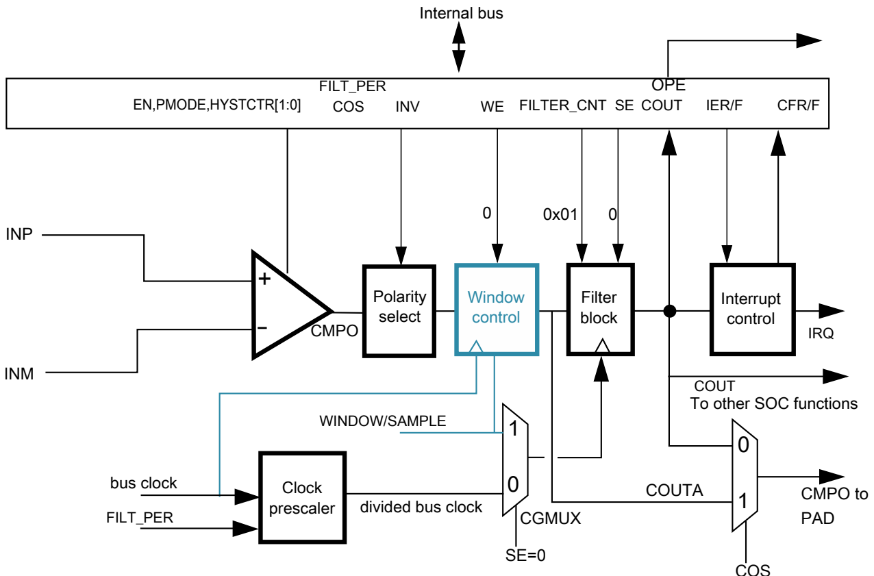
Figure 30-4. Sampled, Non-Filtered (# 3B): sampling interval internally derived
