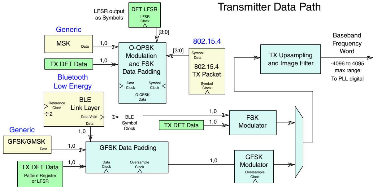
Figure 45-4. Transmitter Digital
