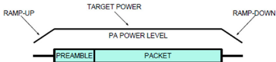
Figure 45-5. Power Amplifier Ramping
