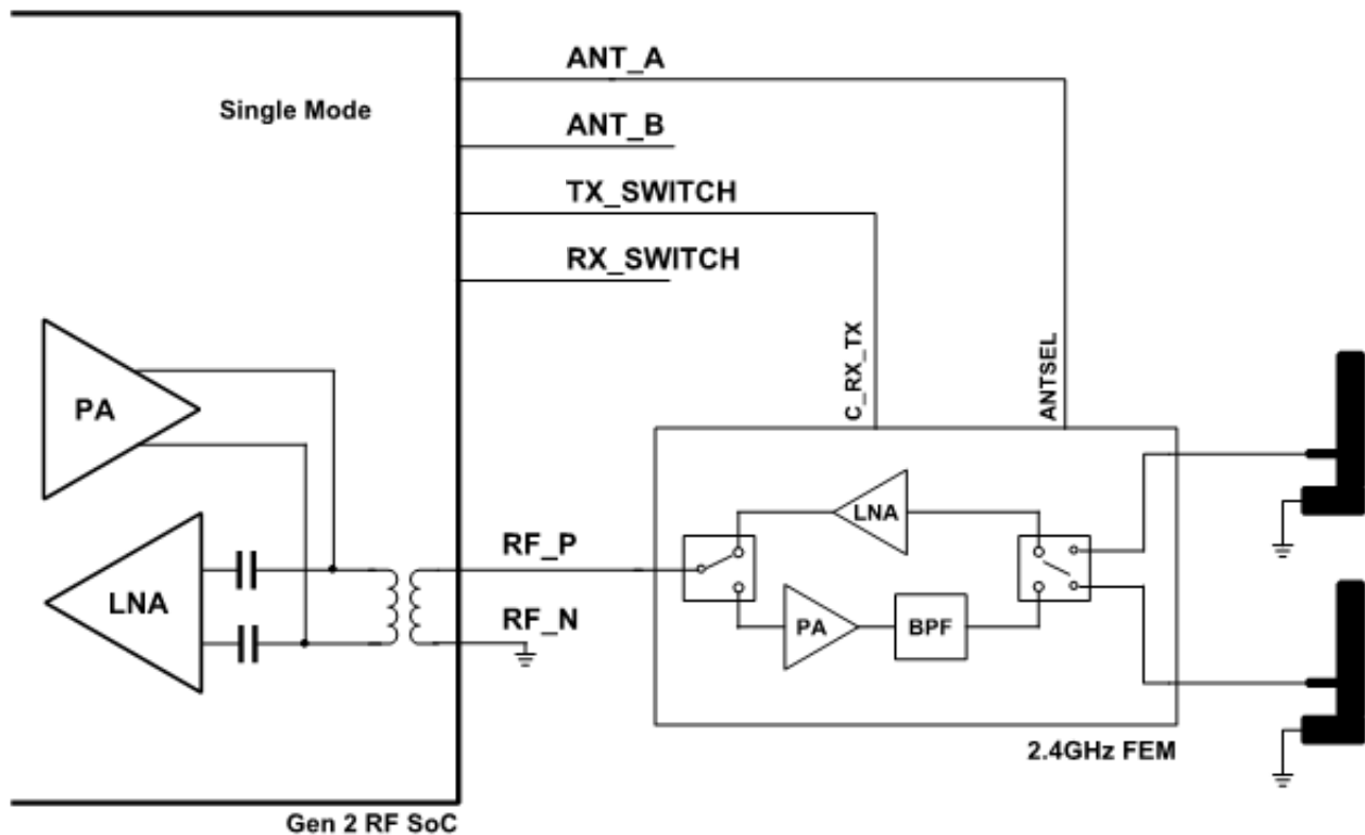
Figure 45-93. FEM Interface Single Mode
