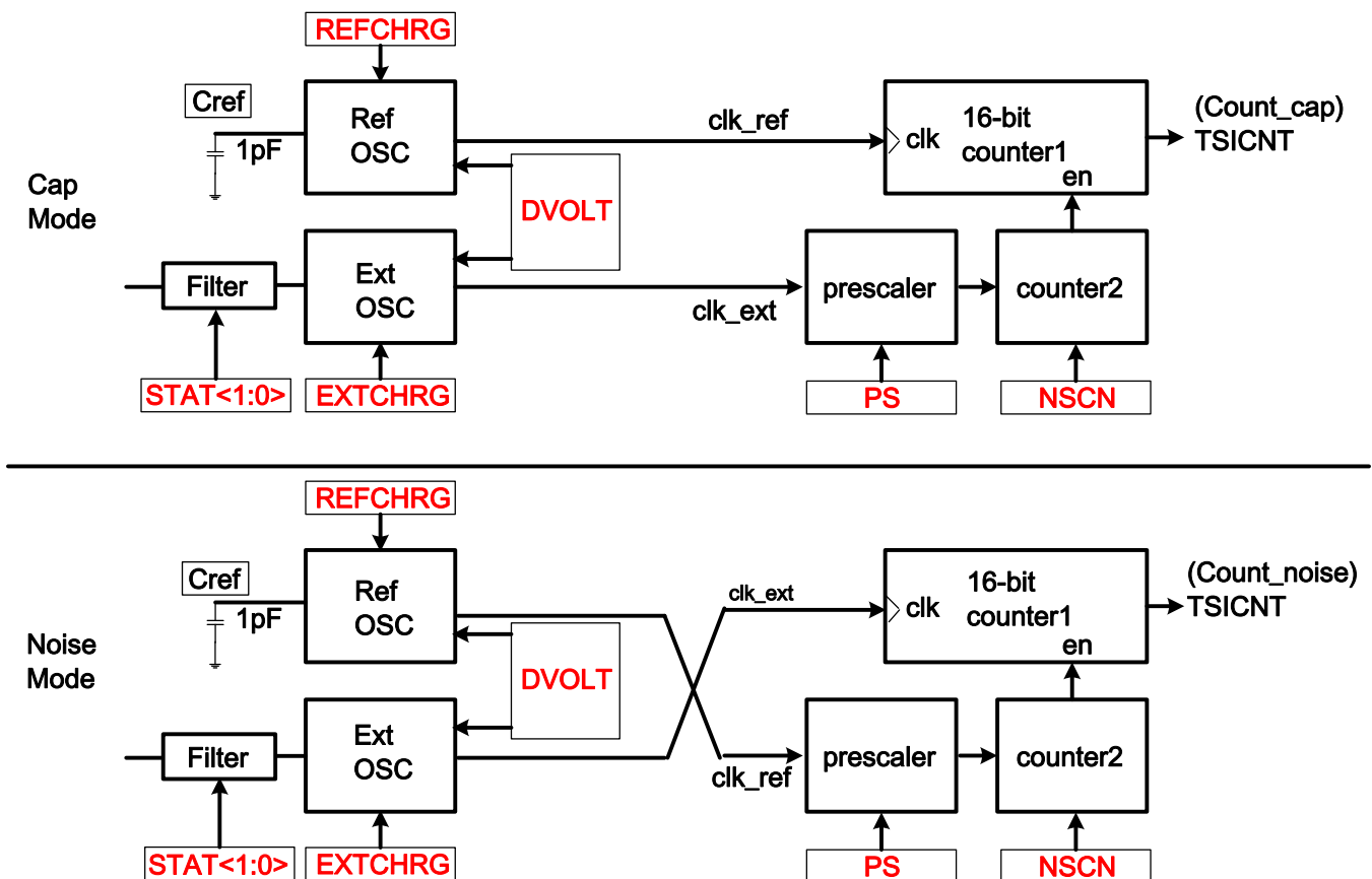
Figure 42-4. TSI noise detection mode block diagram
