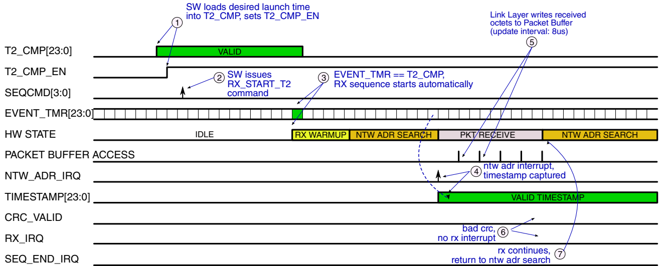
Figure 45-129. GENERIC FSK RX SEQUENCE: LAUNCH VIA T2 TIMER, BAD PACKET, RX RECYCLE
