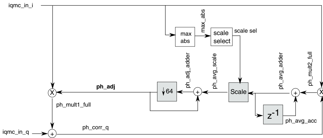
Figure 45-30. I/Q Phase Mismatch Calibration Block Diagram
