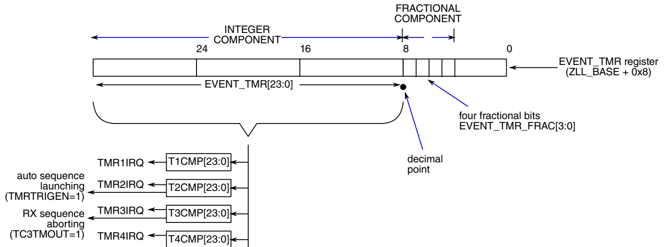
Figure 45-81. Event Timer Hardware Referencing
