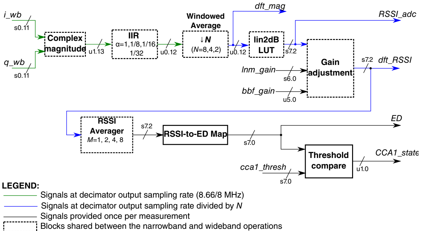
Figure 45-27. Block diagram instantiated for wideband mode
