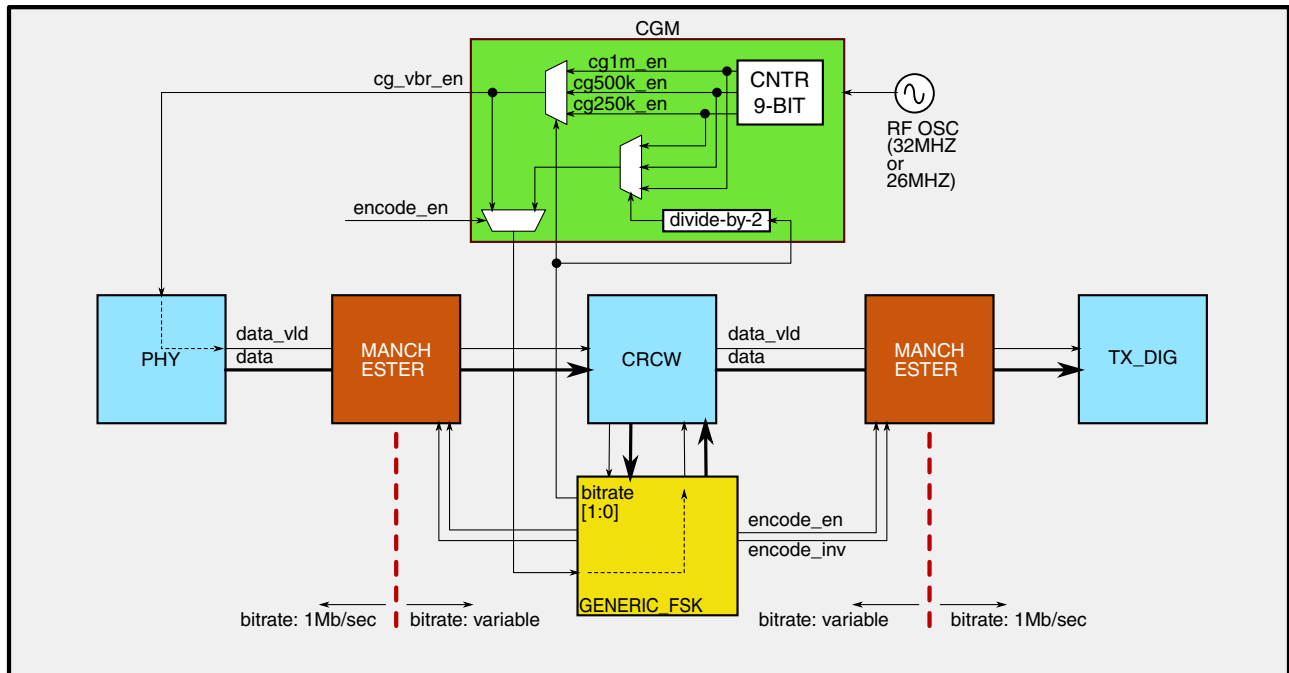
Figure 45-119. BITSTREAM PROCESSING WITH MANCHESTER ENCODING
