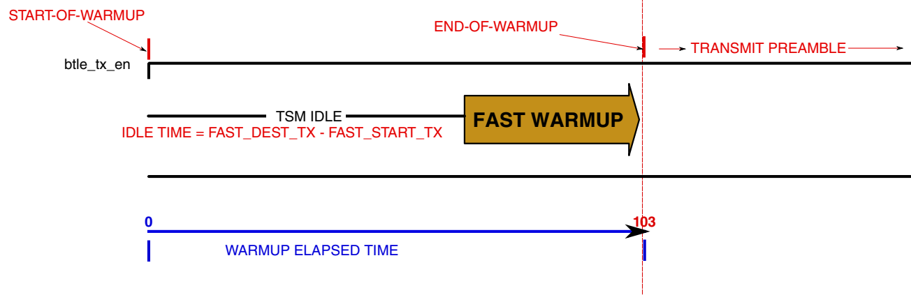
Figure 45-60. Nominal vs. Fast TX Warmups
