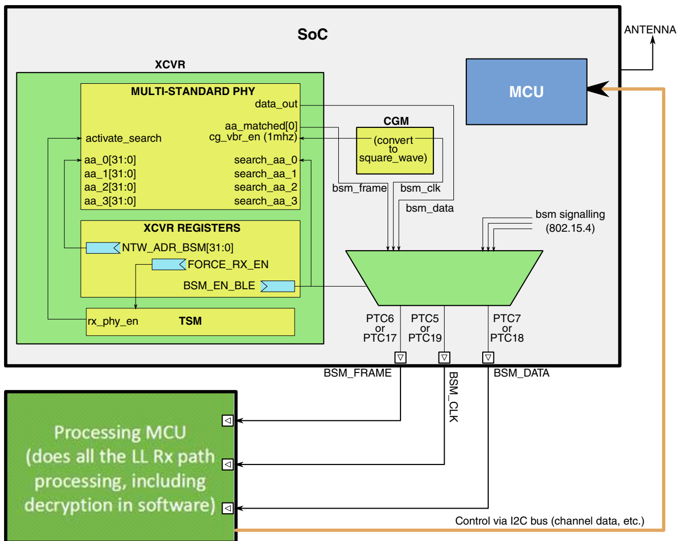
Figure 45-46. BSM Block Diagram
