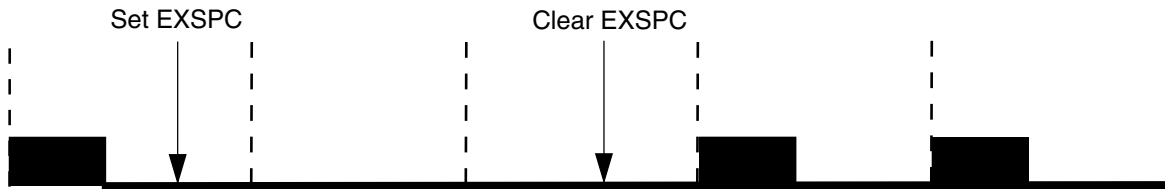
Figure 40-7. Extended space operation
