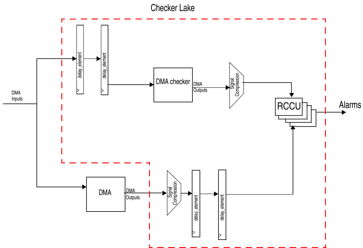
Figure 24-7. Lockstep block diagram
