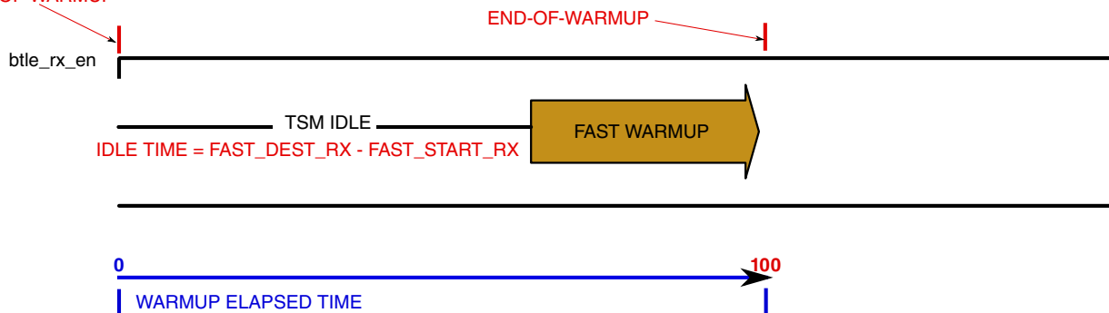
Figure 45-61. Nominal vs. Fast RX Warmups
