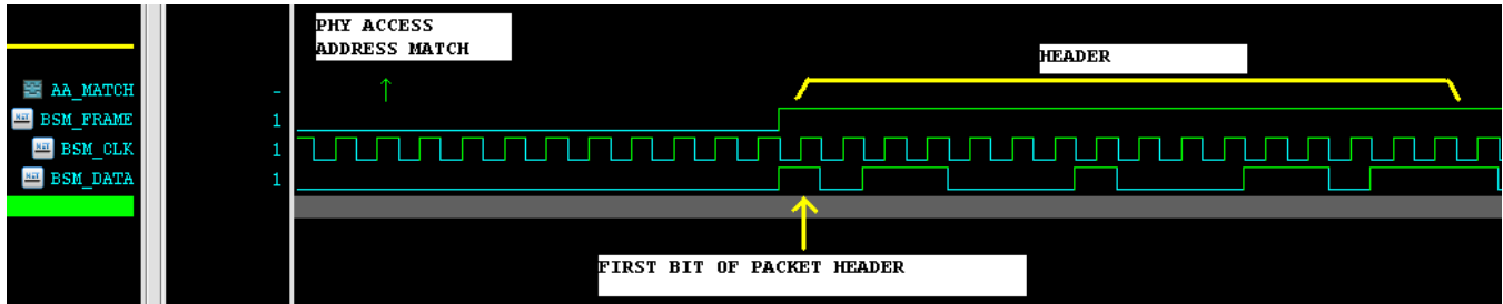
Figure 45-47. BSM Timing Diagram
