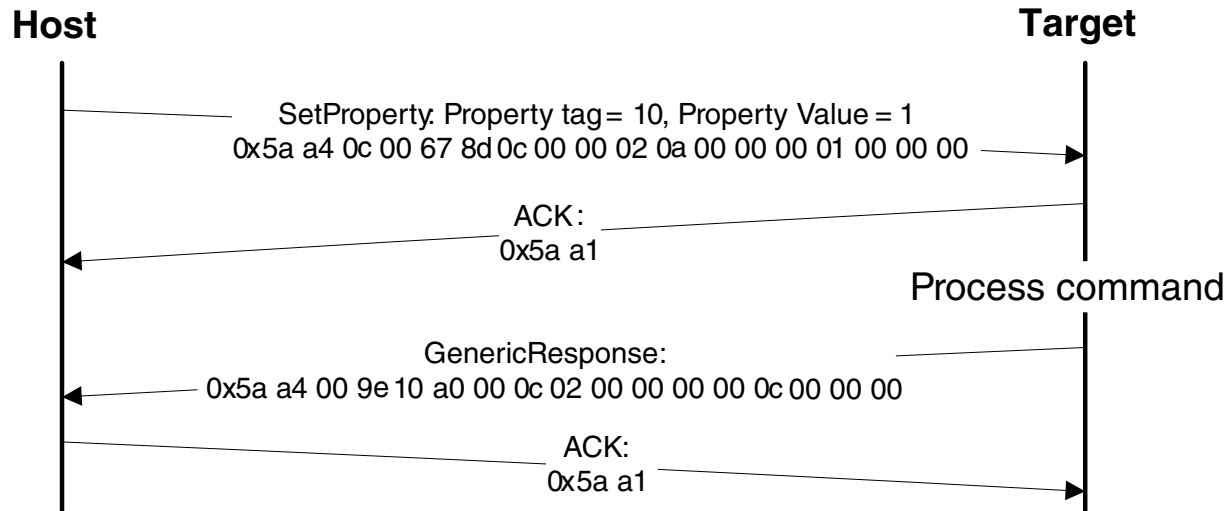
Figure 7-9. Protocol Sequence for SetProperty Command
