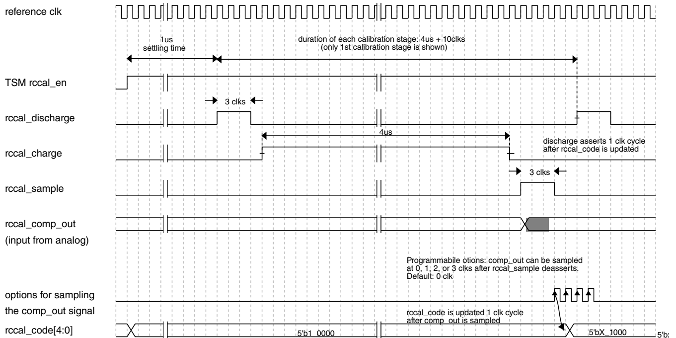
Figure 45-45. RX RCCAL timing
