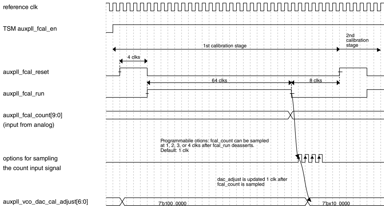
Figure 45-44. RX AuxPLL FCAL timing
