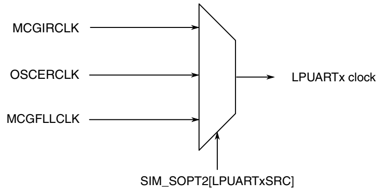
Figure 5-6. LPUART clock generation
