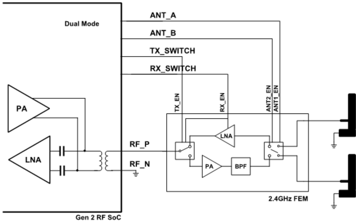
Figure 45-95. FEM Interface Dual Mode
