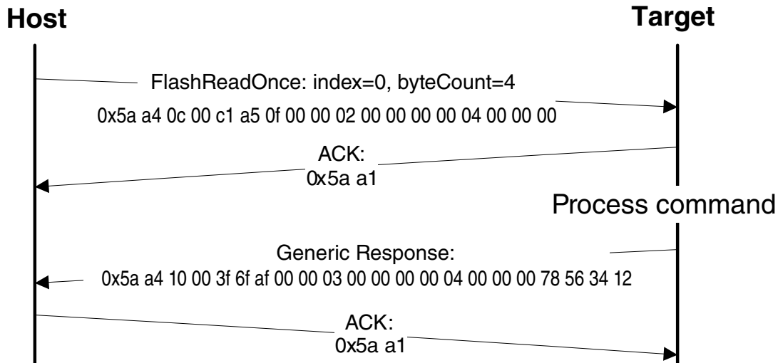
Figure 7-15. Protocol Sequence for FlashReadOnce Command
