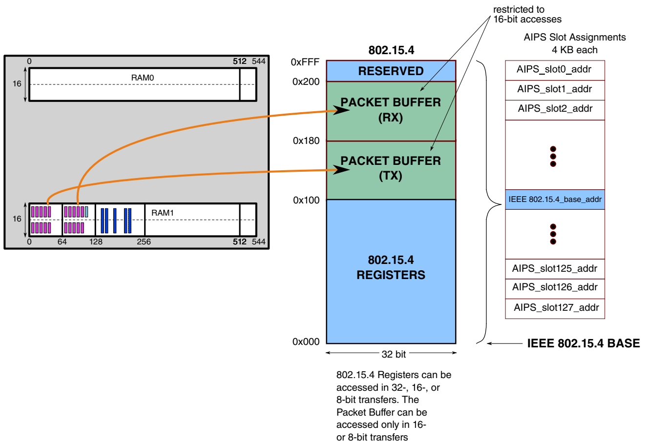
Figure 45-79. 802.15.4 MEMORY MAPPING
