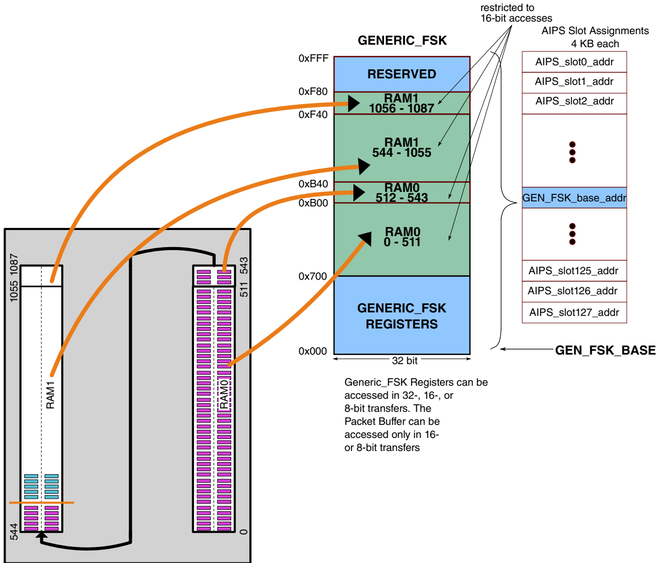
Figure 45-126. GENERIC_FSK MEMORY MAPPING
