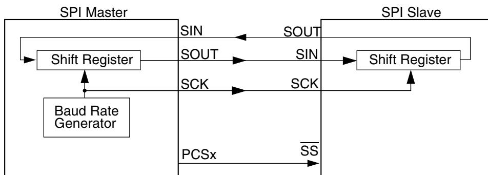
Figure 37-3. Serial protocol overview
