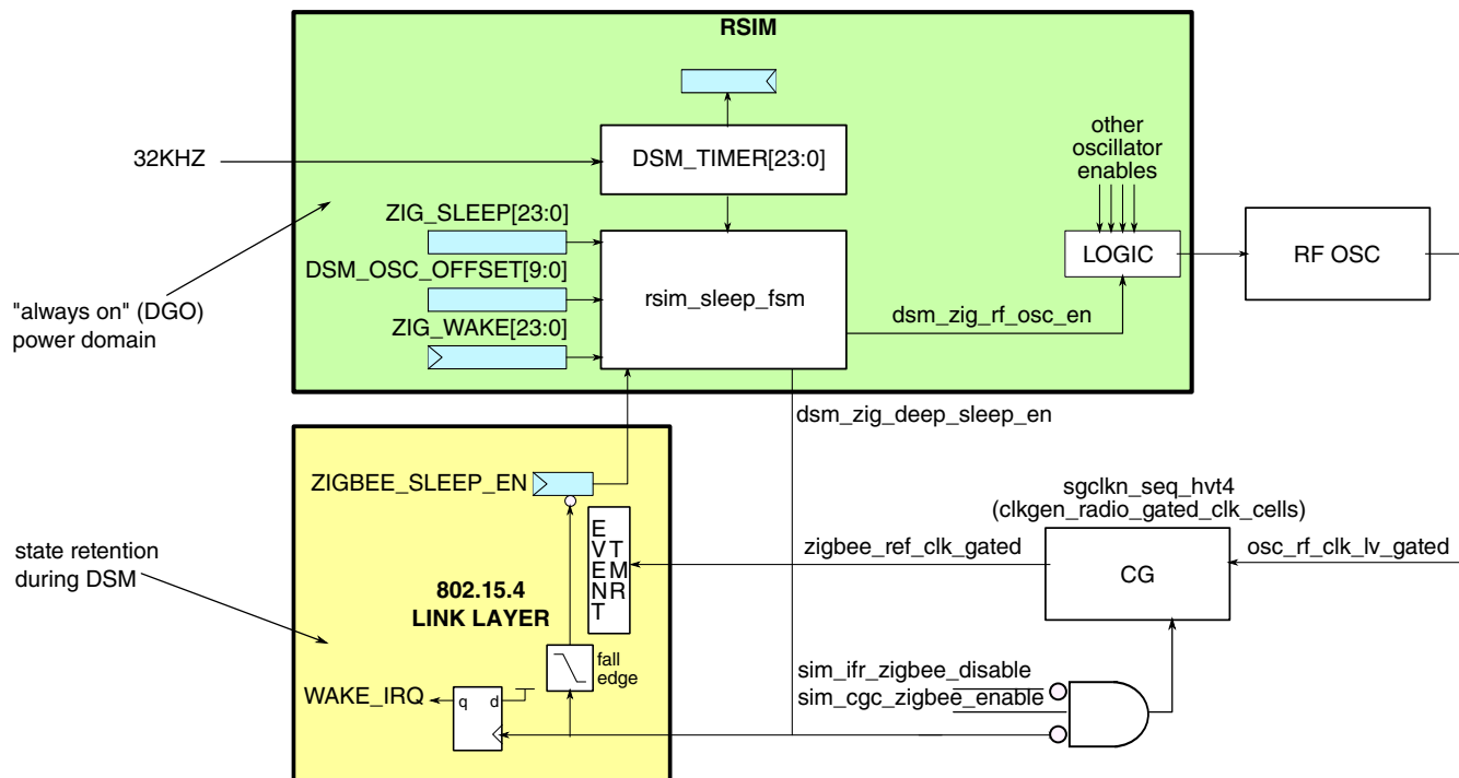
Figure 45-82. Deep Sleep Mode
