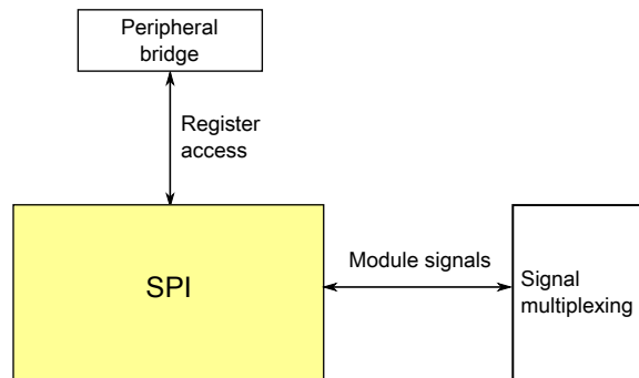
Figure 3-37. SPI configuration
