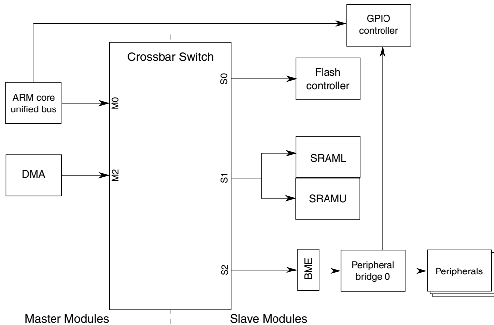
Figure 3-13. Crossbar-light switch integration
