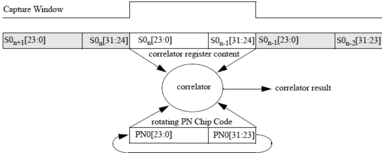
Figure 45-87. S0 Symbol Search
