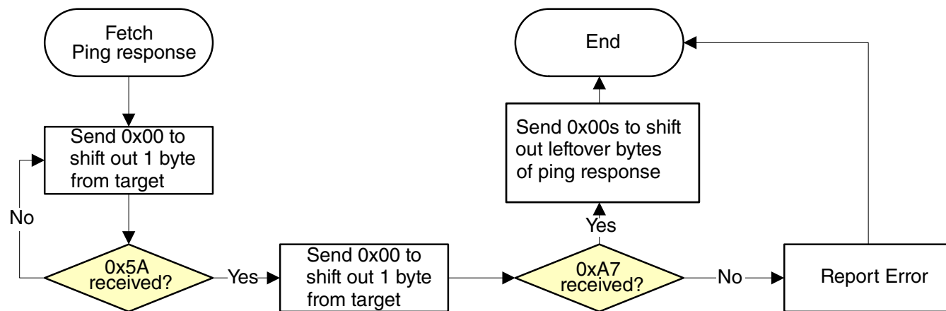
Figure 7-23. Host reads ping packet from target via SPI
