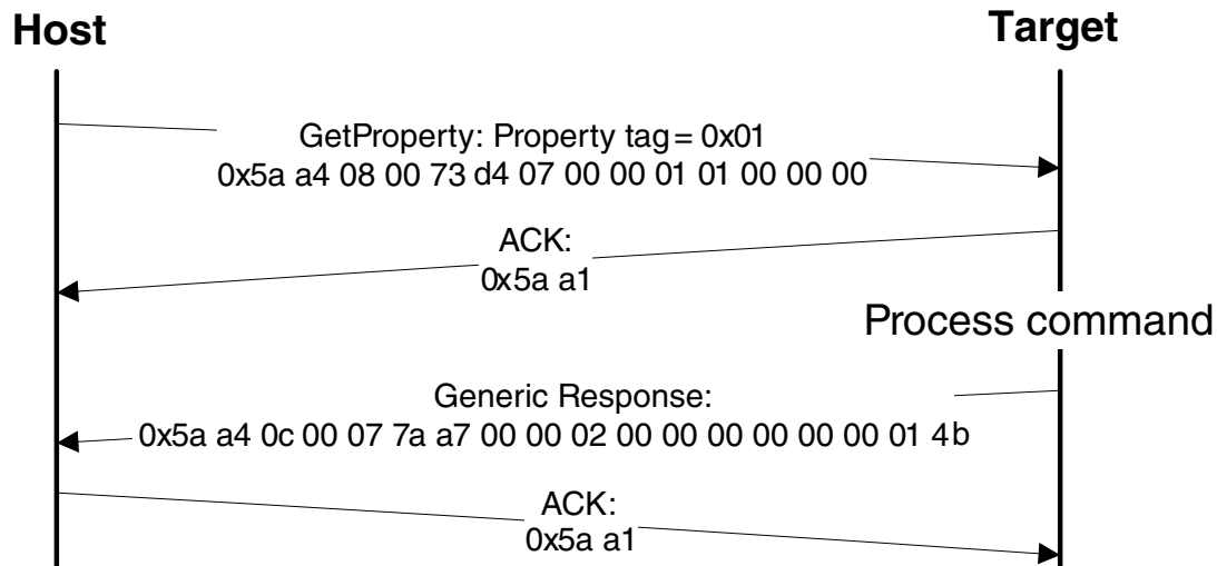
Figure 7-8. Protocol Sequence for GetProperty Command
