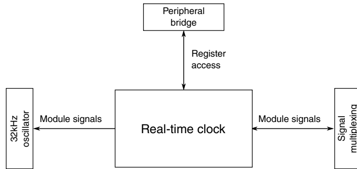
Figure 3-36. RTC configuration
