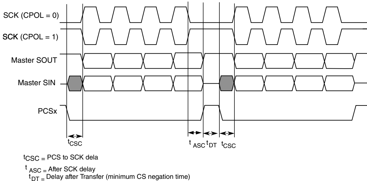
Figure 37-13. Example of non-continuous format (CPHA=1, CONT=0)
