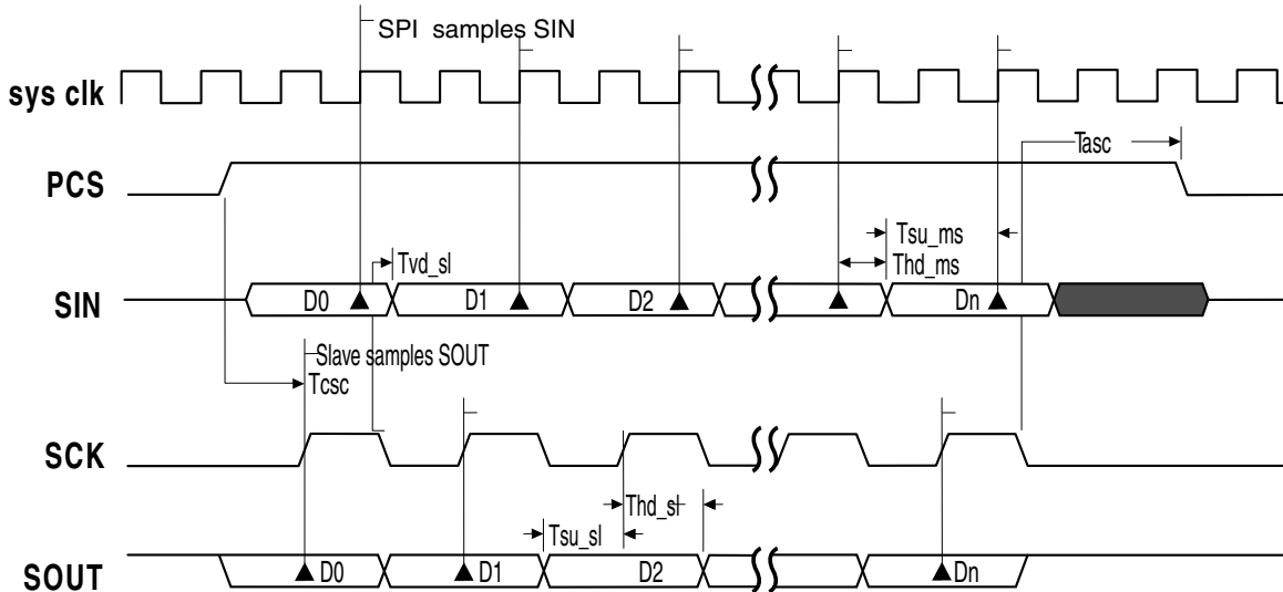
Figure 37-7. SPI Modified Transfer Format (MTFE=1, CPHA=0, f_{sck} = f_{sys}/4 )
