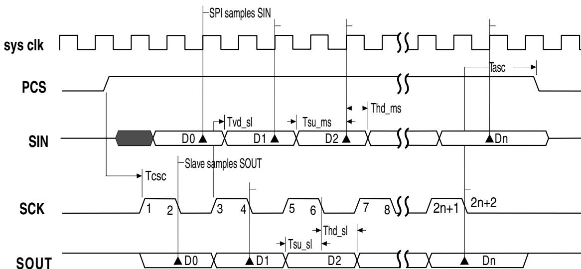
Figure 37-10. SPI Modified Transfer Format (MTFE=1, CPHA=1, f_{sck} = f_{sys}/2 )
