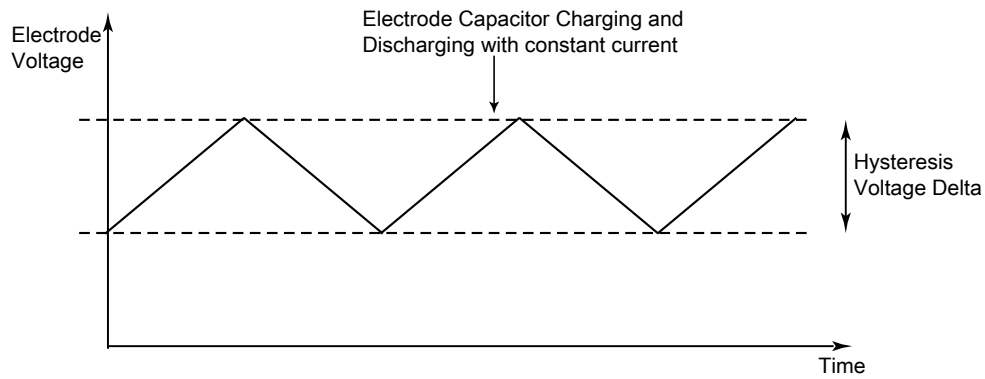
Figure 42-3. TSI electrode oscillator chart
