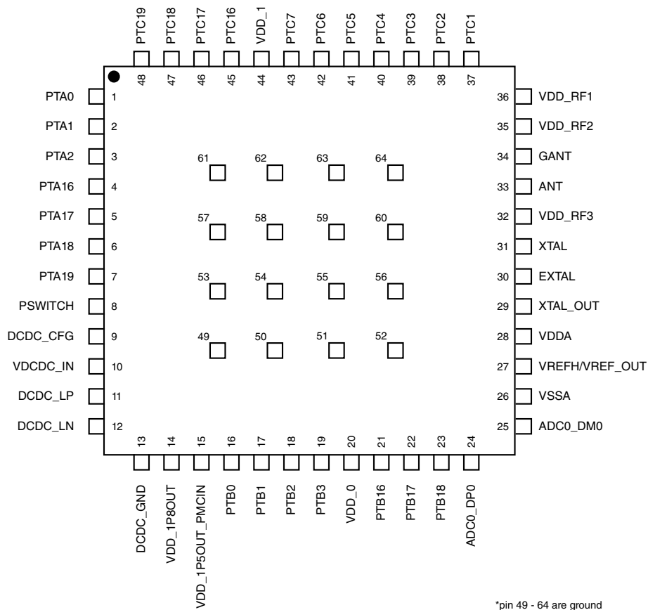
Figure 2-1. 48-pin Laminated QFN pinout diagram
