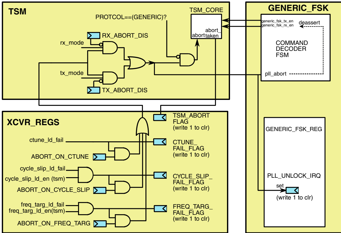
Figure 45-53. GENERIC_FSK PLL UNLOCK HANDLING
