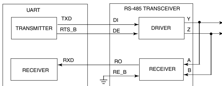
Figure 39-4. Transceiver driver enable using LPUART_RTS
