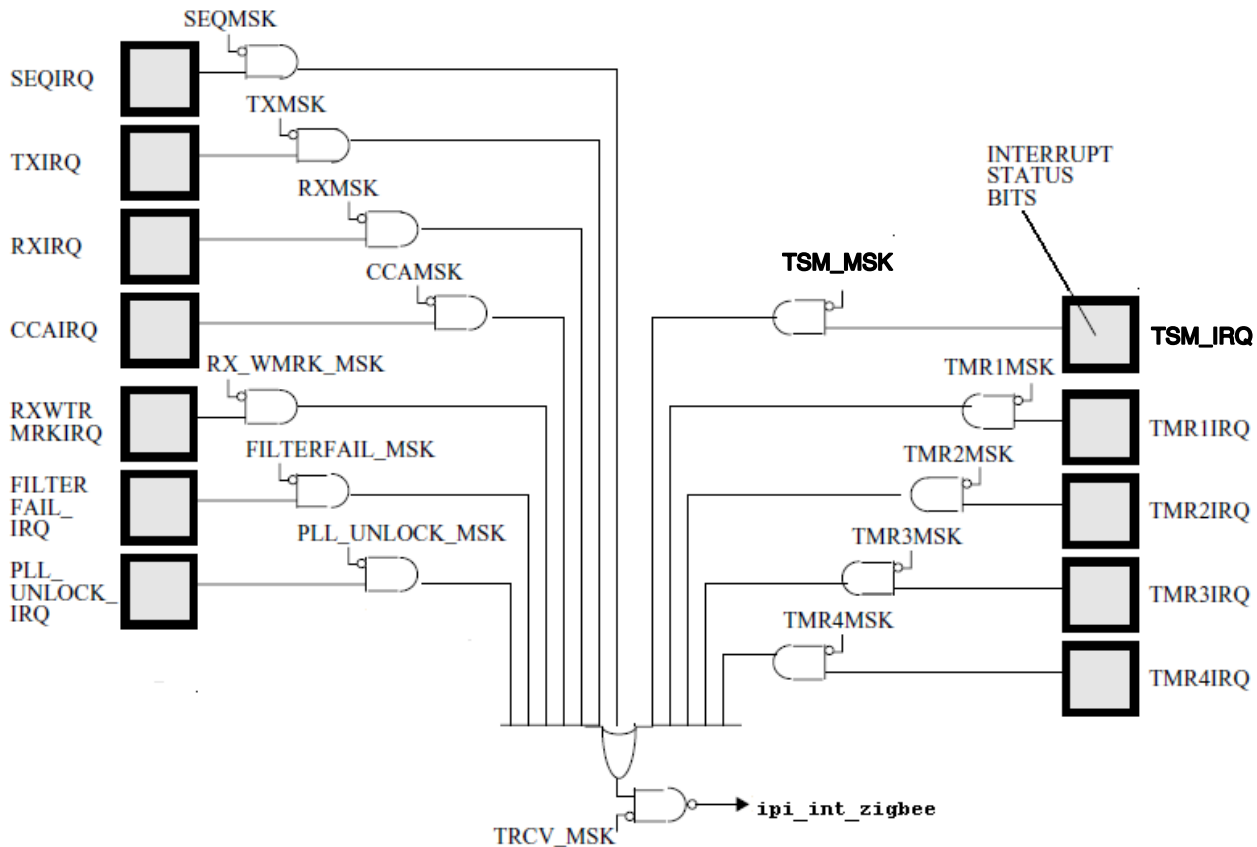
Figure 45-98. 802.15.4 Interrupt Architecture
