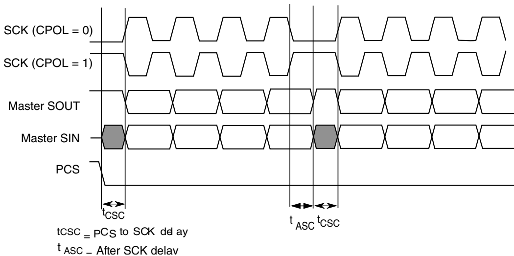
Figure 37-14. Example of continuous transfer (CPHA=1, CONT=1)
