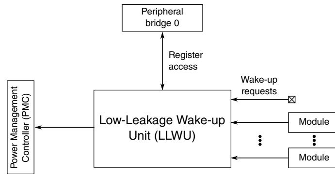
Figure 3-11. Low-Leakage Wake-up Unit configuration
