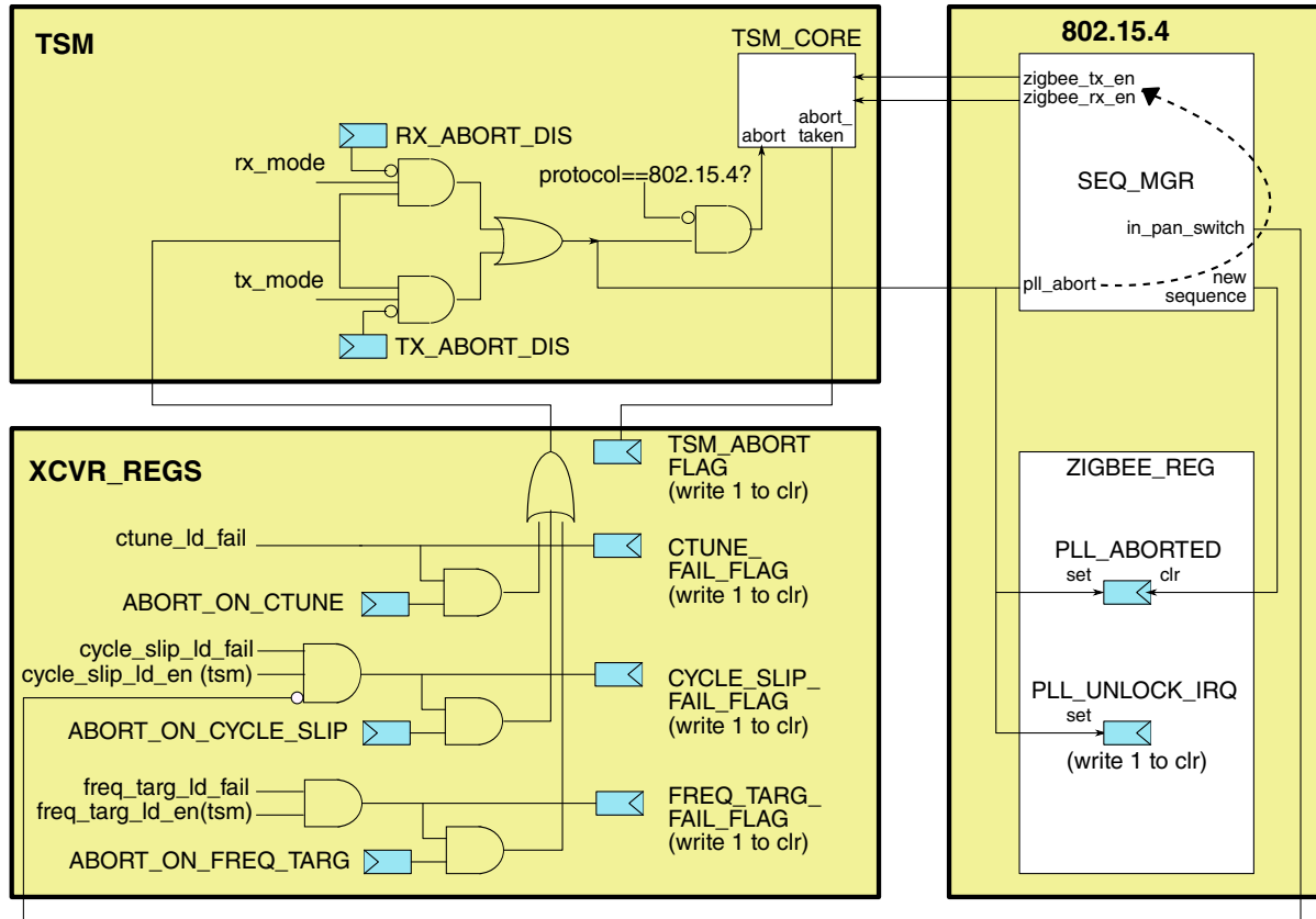
Figure 45-52. 802.15.4 PLL UNLOCK HANDLING
