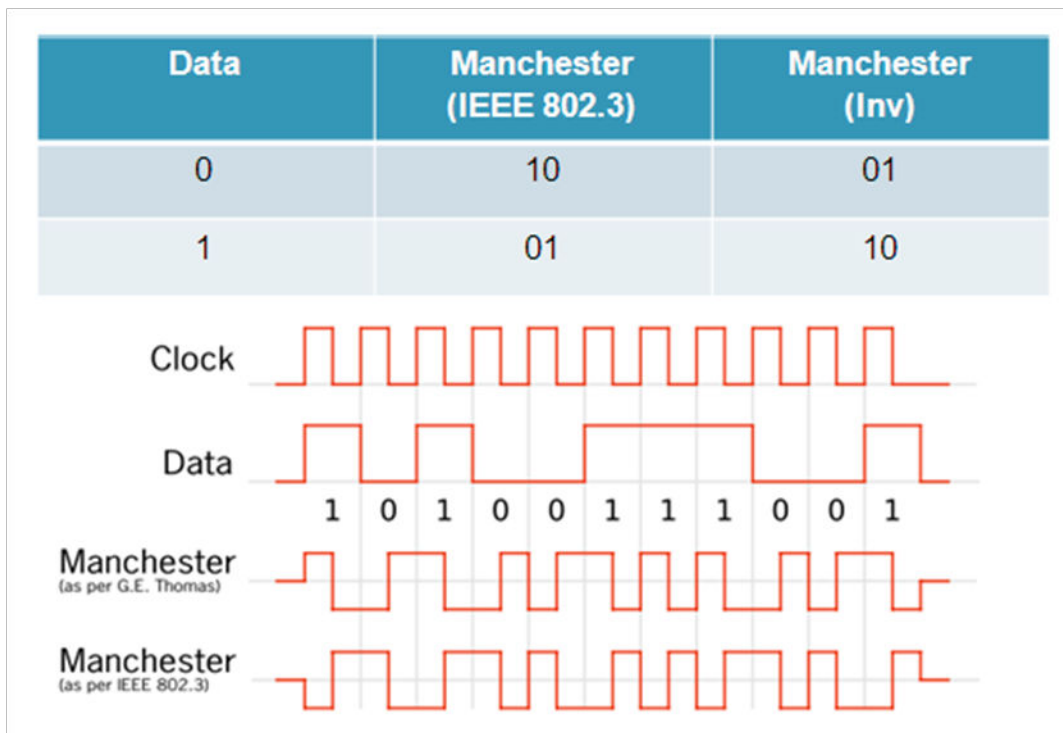
Figure 45-118. Manchester Encoding
