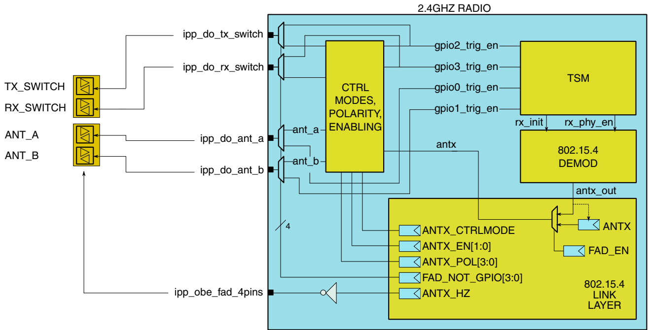
Figure 45-90. FAD Pin Interface
