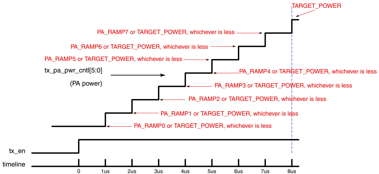
Figure 45-58. PA RAMP UP(8us)
