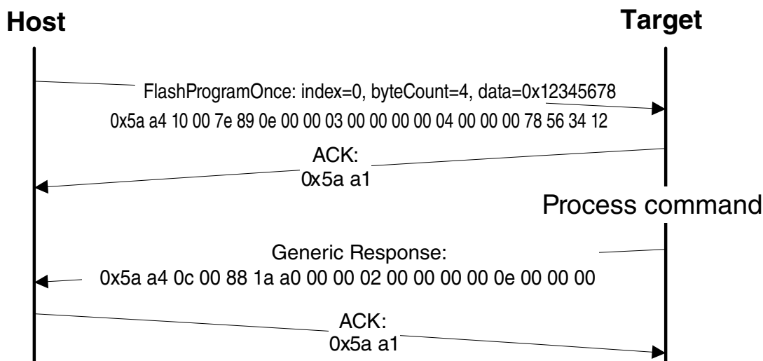
Figure 7-14. Protocol Sequence for FlashProgramOnce Command
