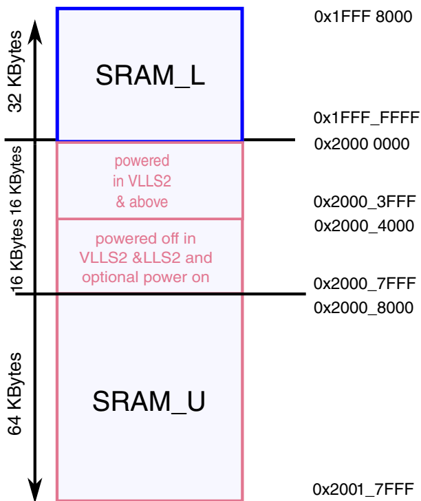
Figure 3-25. SRAM blocks memory map
