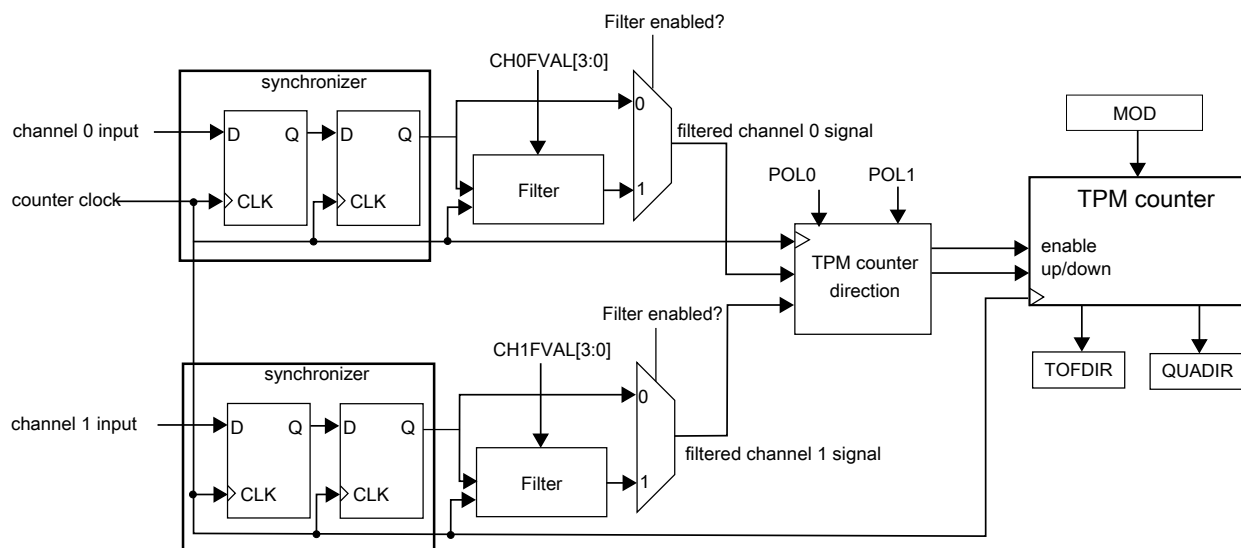
Figure 33-27. Quadrature Decoder block diagram
