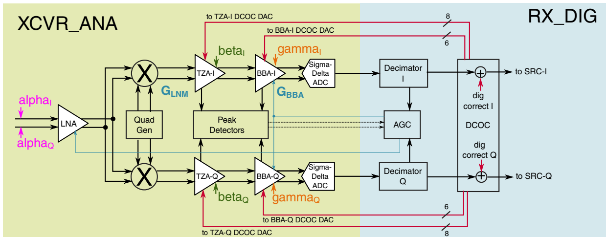
Figure 45-38. Receiver model showing three contributors of DC offset
