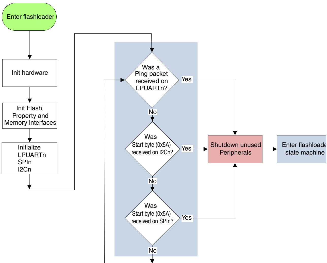
Figure 7-2. Kinetis Flashloader Start-up Flowchart
