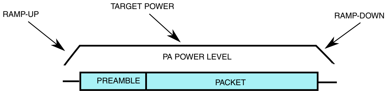
Figure 45-54. PA Target Power
