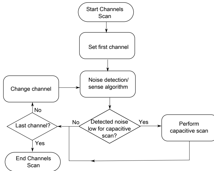
Figure 42-7. Detection of touch with noise sense and normal capacitive sense flow chart
