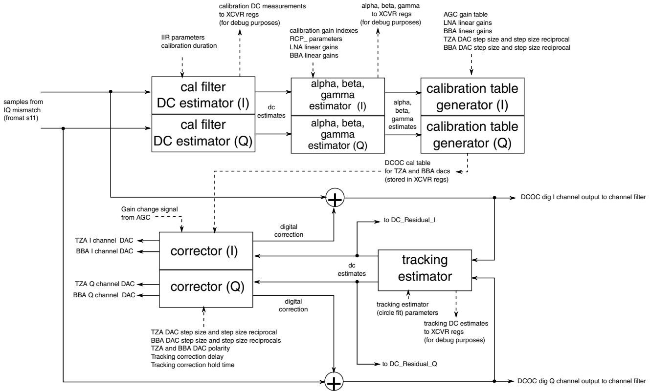
Figure 45-32. RX_DIG DCOC Block Diagram
