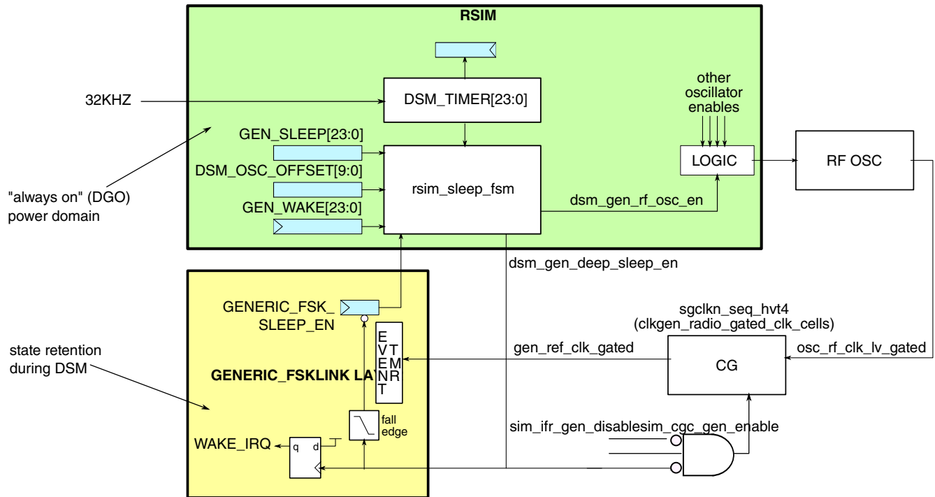
Figure 45-131. Deep Sleep Mode
