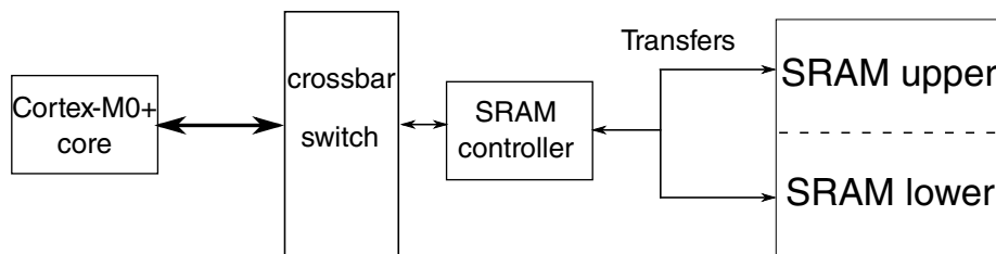
Figure 3-24. SRAM configuration
