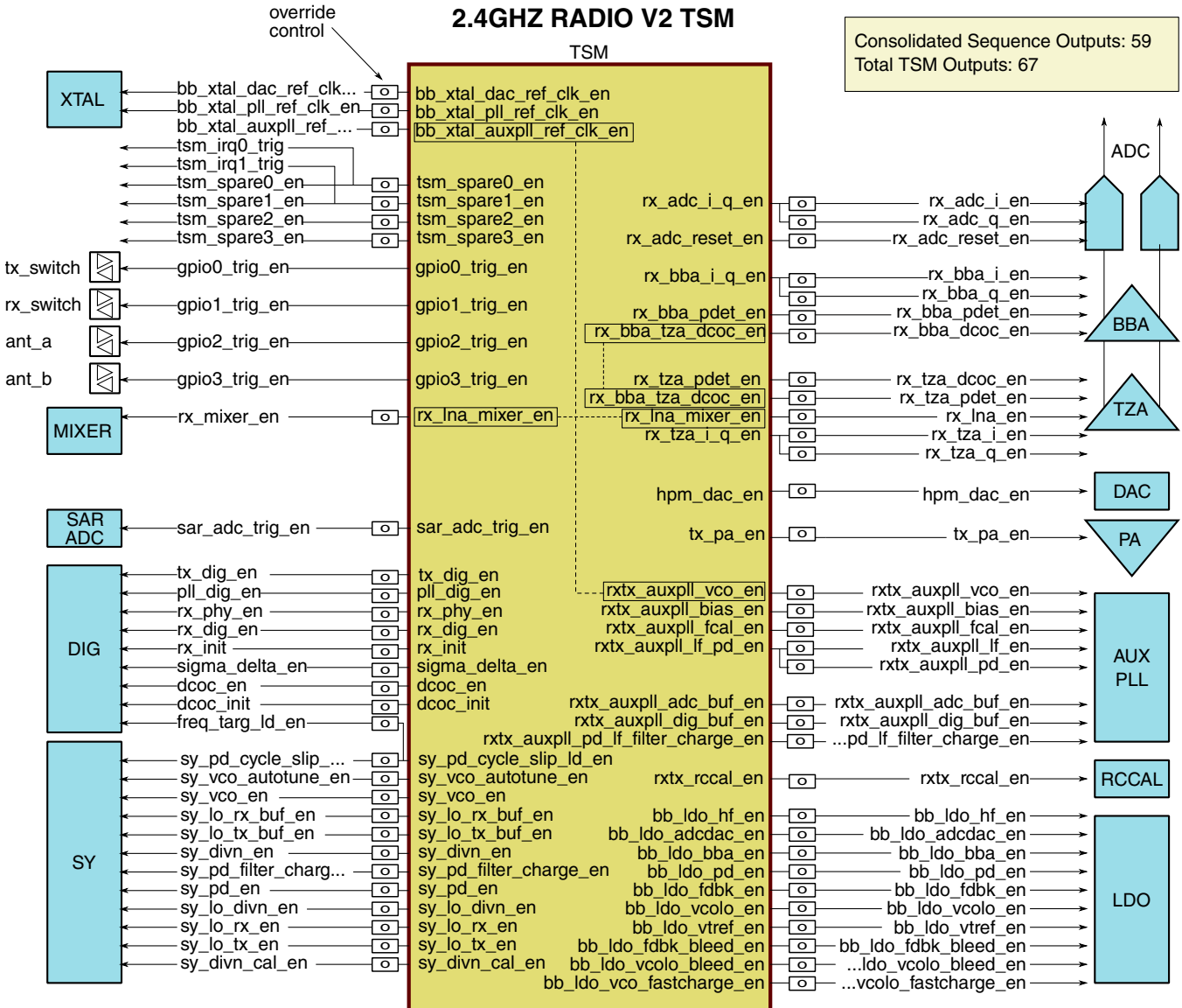
Figure 45-48. Block diagram
