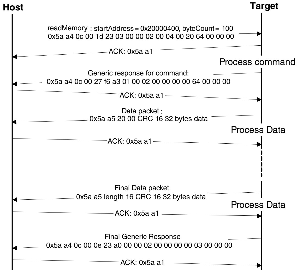
Figure 7-18. Command sequence for read memory
