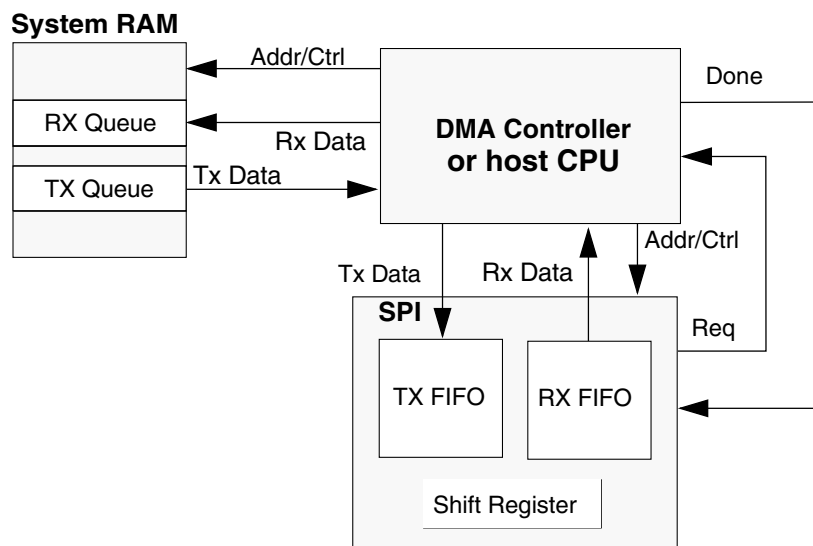
Figure 37-2. SPI with queues and DMA
