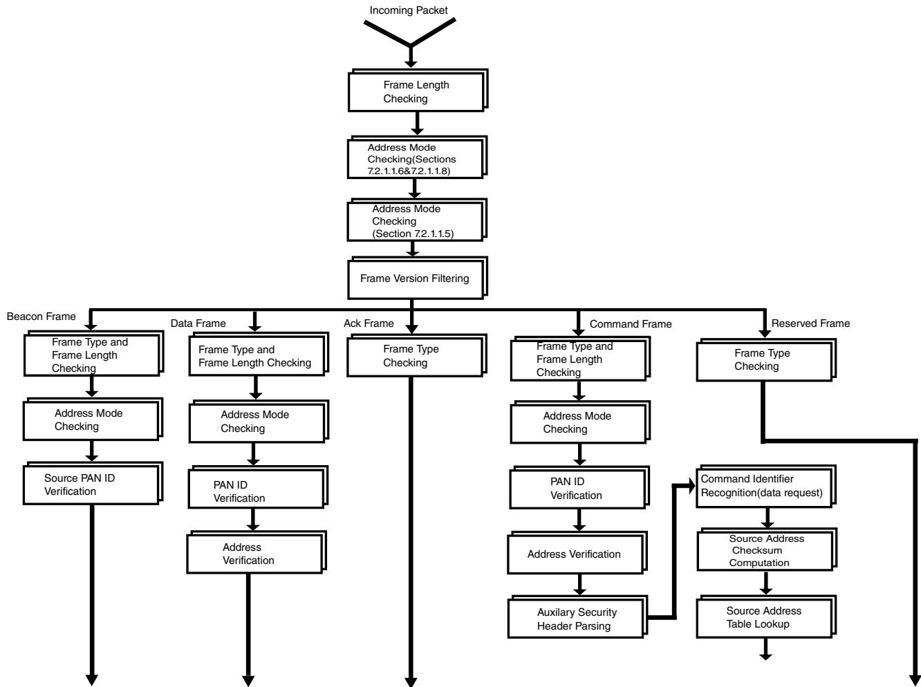
Figure 45-74. Packet Filtering Flow Diagram
