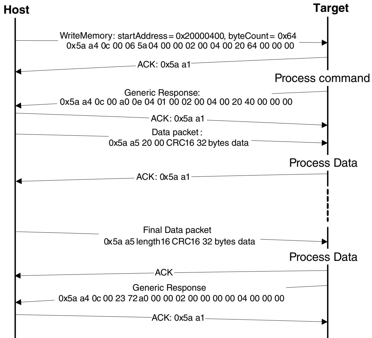
Figure 7-17. Protocol Sequence for WriteMemory Command
