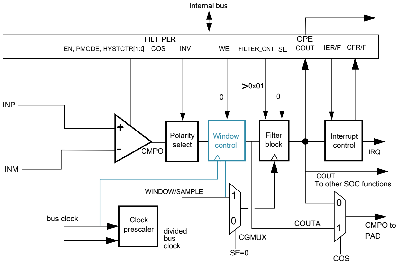
Figure 30-5. Sampled, Filtered (# 4B): sampling point internally derived
