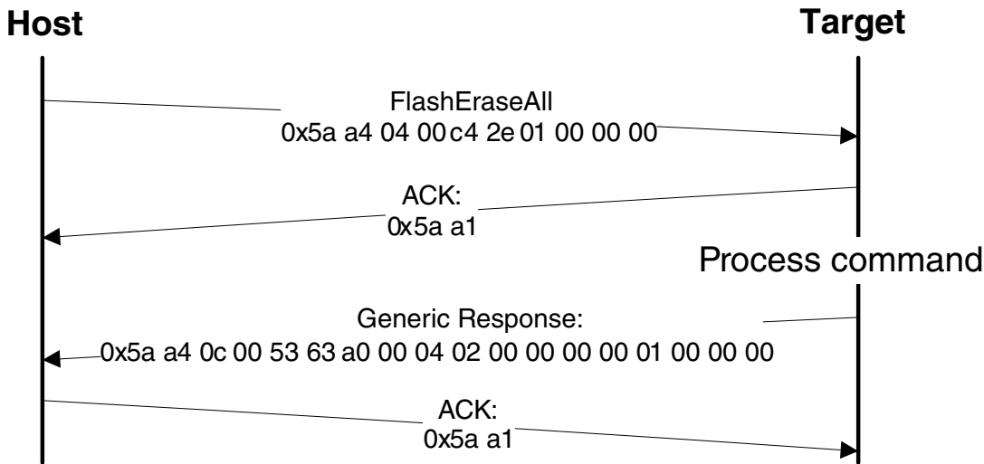
Figure 7-10. Protocol Sequence for FlashEraseAll Command
