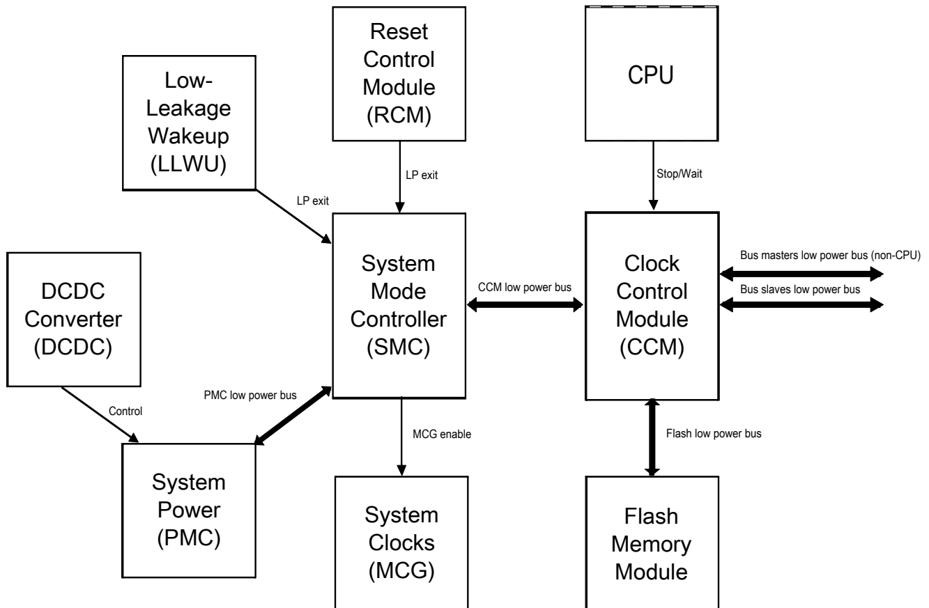
Figure 13-2. Low-power system components and connections
