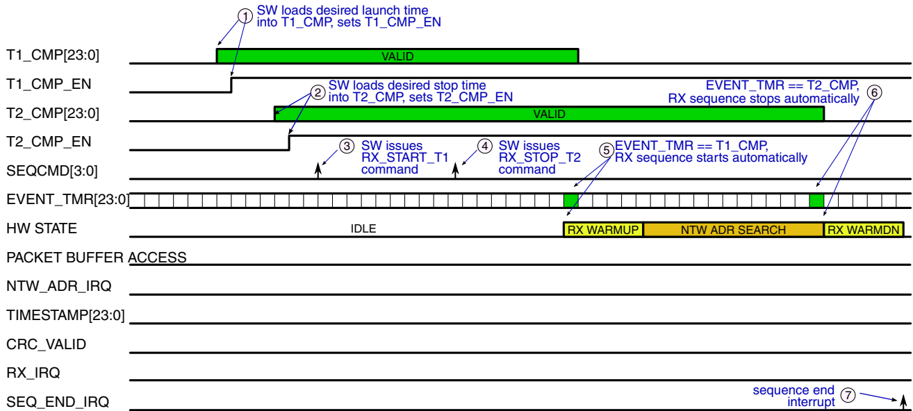
Figure 45-130. GENERIC FSK RX SEQUENCE: SLAVE CHANNEL SEARCH, LAUNCH VIA T1, STOP VIA T2
