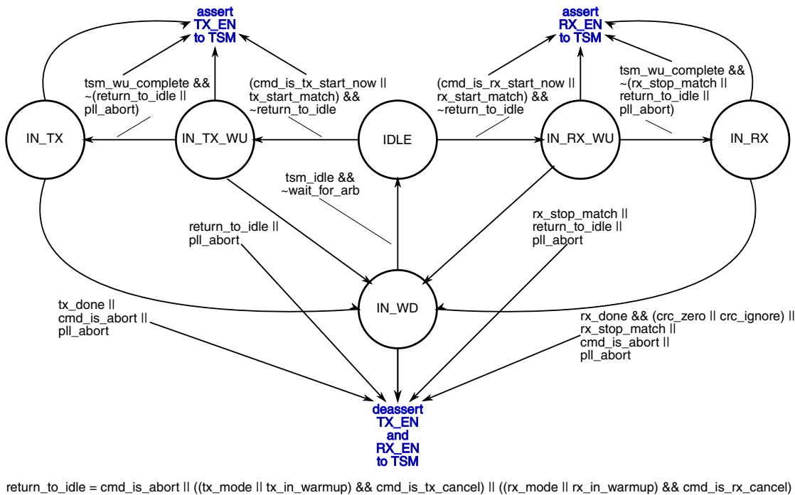
Figure 45-123. GENERIC COMMAND DECODER FSM
