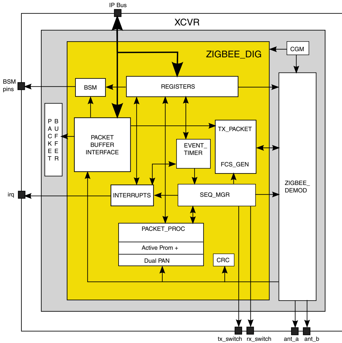
Figure 45-68. 802.15.4 Link Layer Controller Block Diagram
