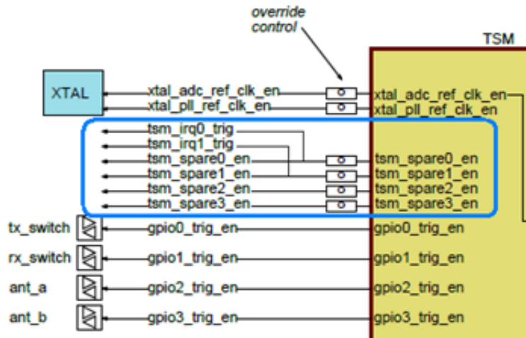
Figure 45-62. TSM Interrupt Re-use Scheme
