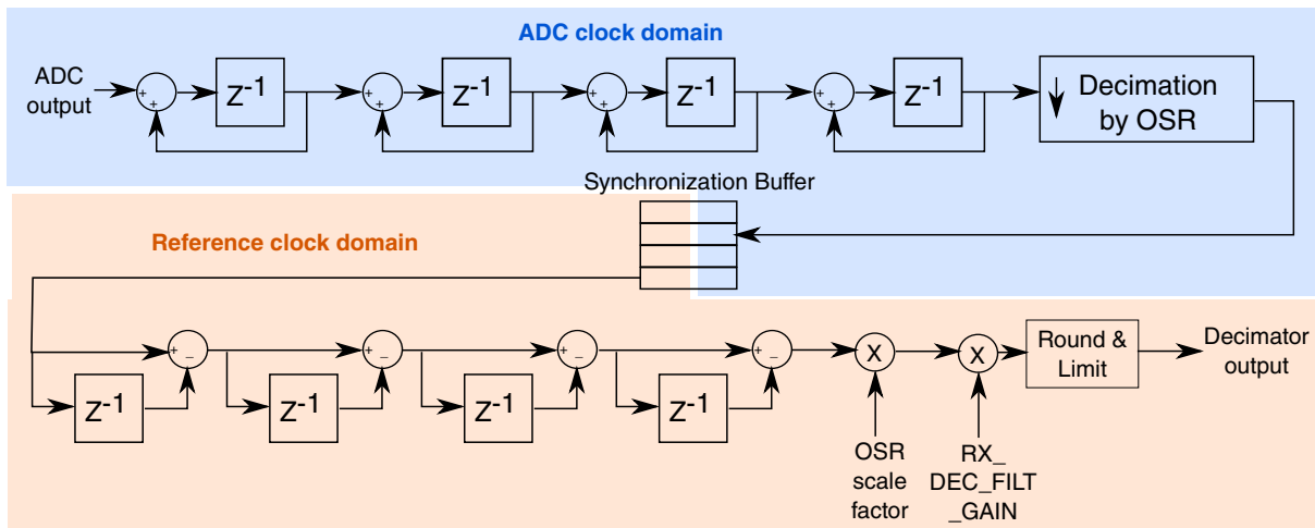
Figure 45-21. Decimation Filter Block Diagram
