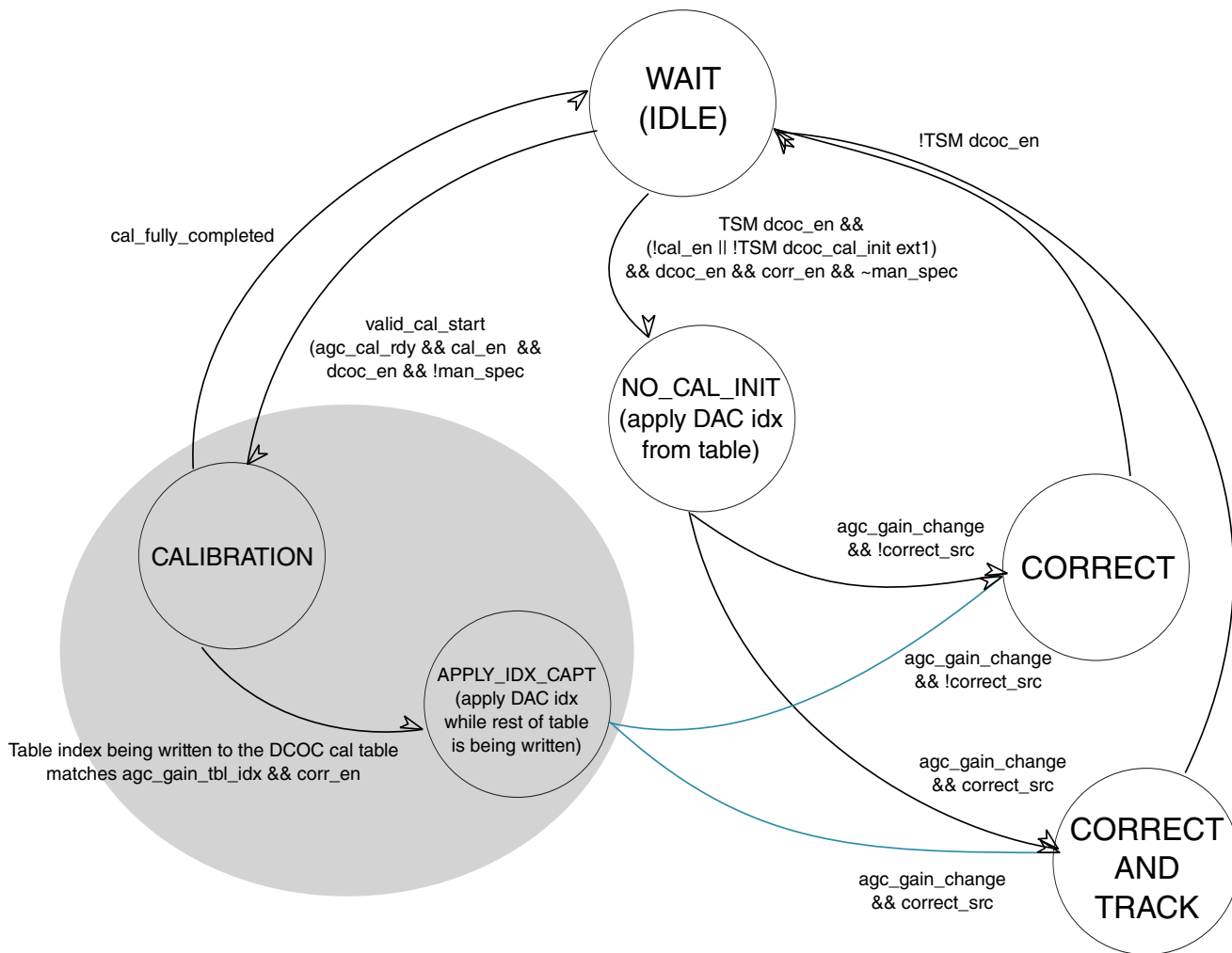
Figure 45-33. DCOC State Diagram
