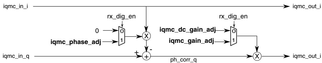
Figure 45-31. I/Q Mismatch Correction Block Diagram
