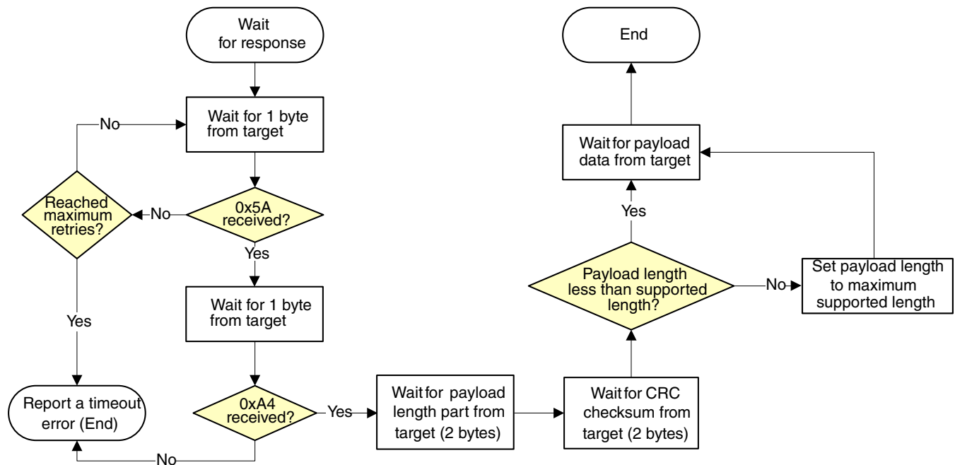
Figure 7-28. Host reads a command response from target via LPUART
