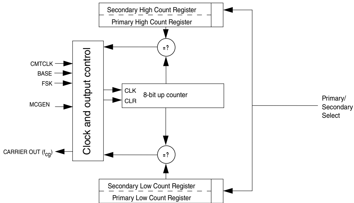
Figure 40-3. Carrier generator block diagram
