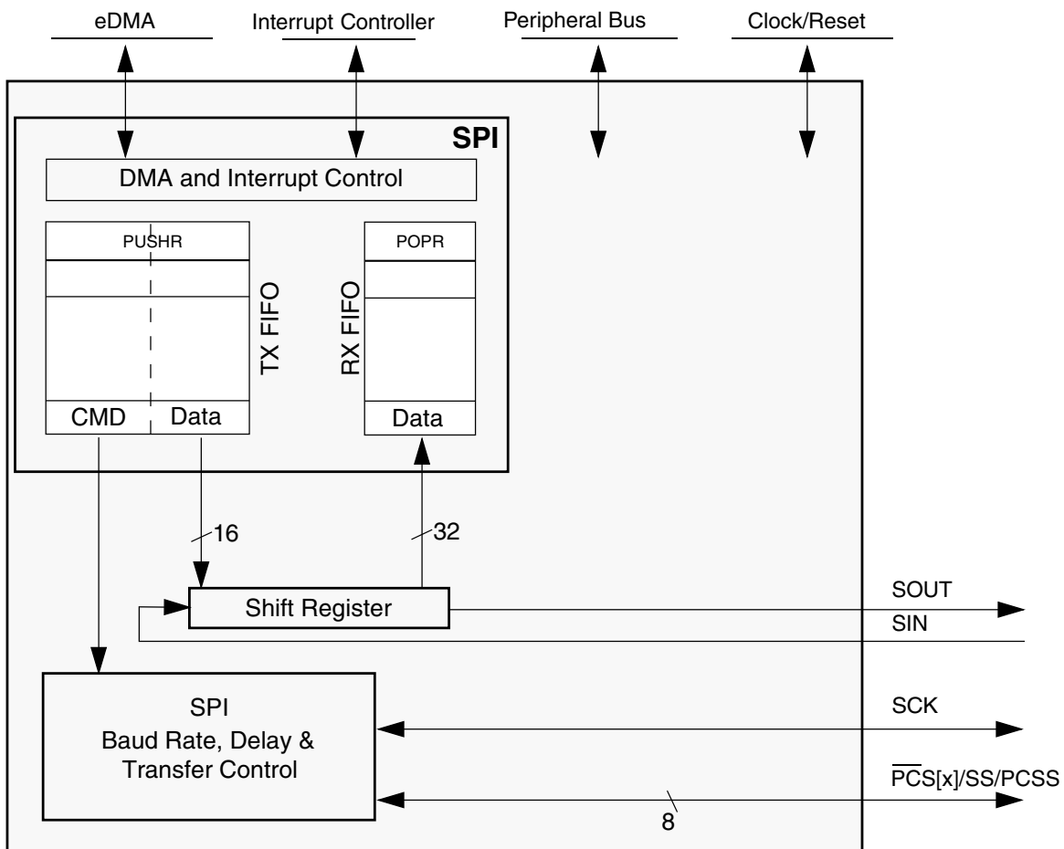
Figure 37-1. SPI Block Diagram
