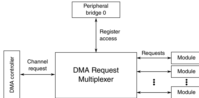
Figure 3-15. DMA request multiplexer configuration
