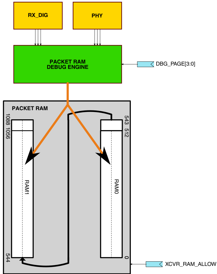
Figure 45-64. Packet RAM Debug Mode Block Diagram
