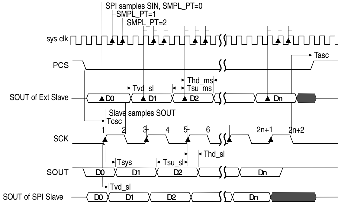
Figure 37-7. SPI Modified Transfer Format (MTFE=1, CPHA=0, f_{sck} = f_{sys}/4 )
