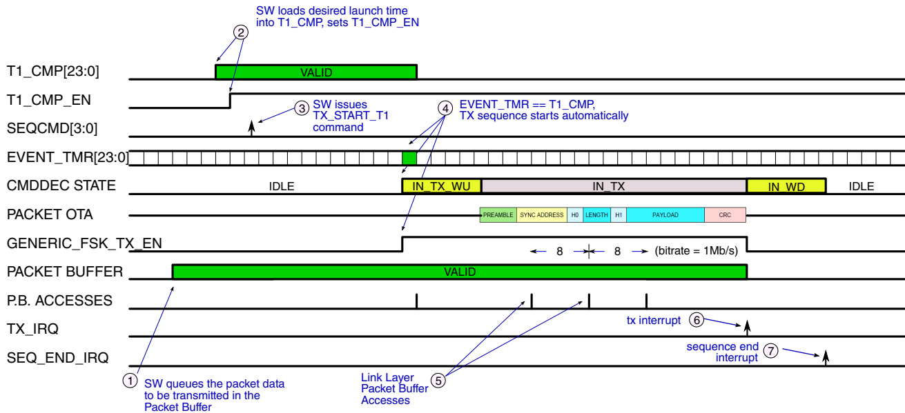
Figure 45-127. GENERIC FSK TX SEQUENCE: LAUNCH VIA T1 TIMER
