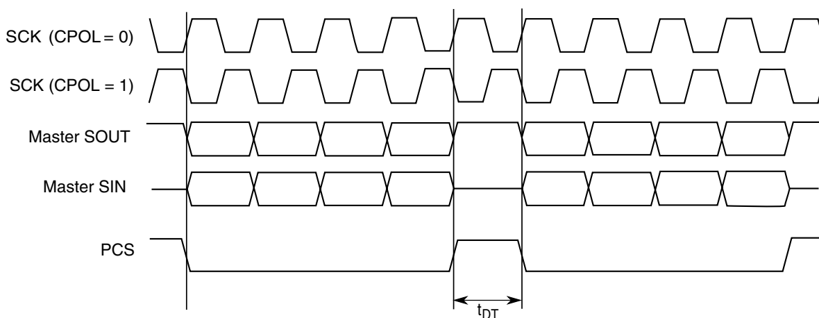
Figure 37-15. Continuous SCK Timing Diagram (CONT=0)
