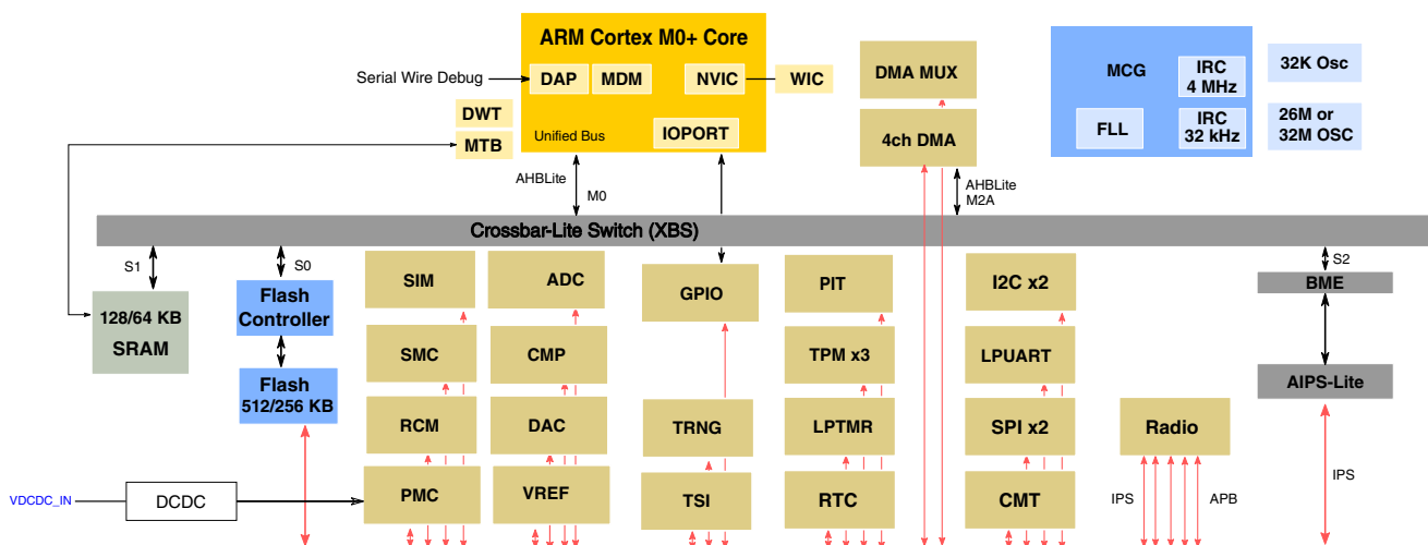
Figure 1-1. KW41Z Detailed Block Diagram
