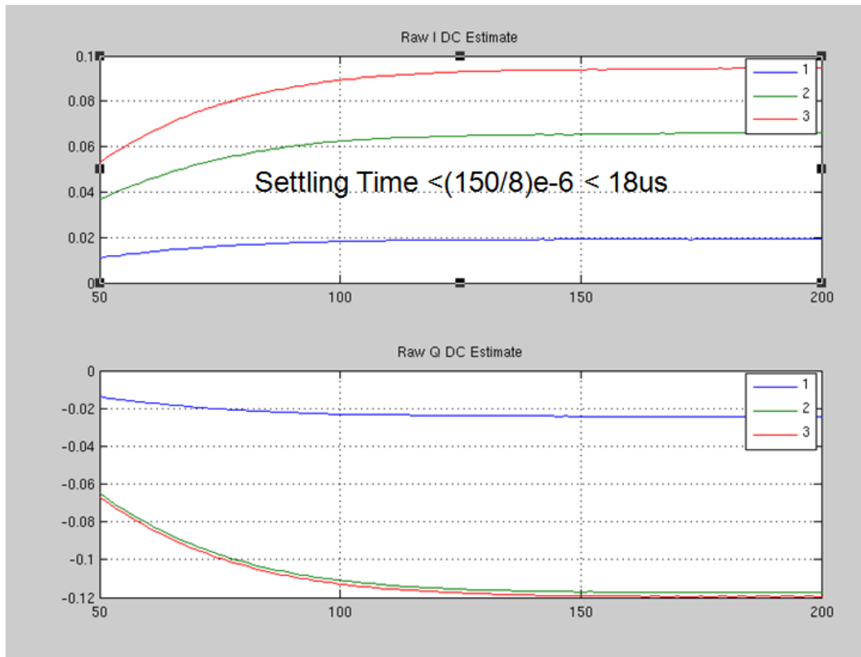
Figure 45-37. 3-step {I,Q} DC estimation during calibration
