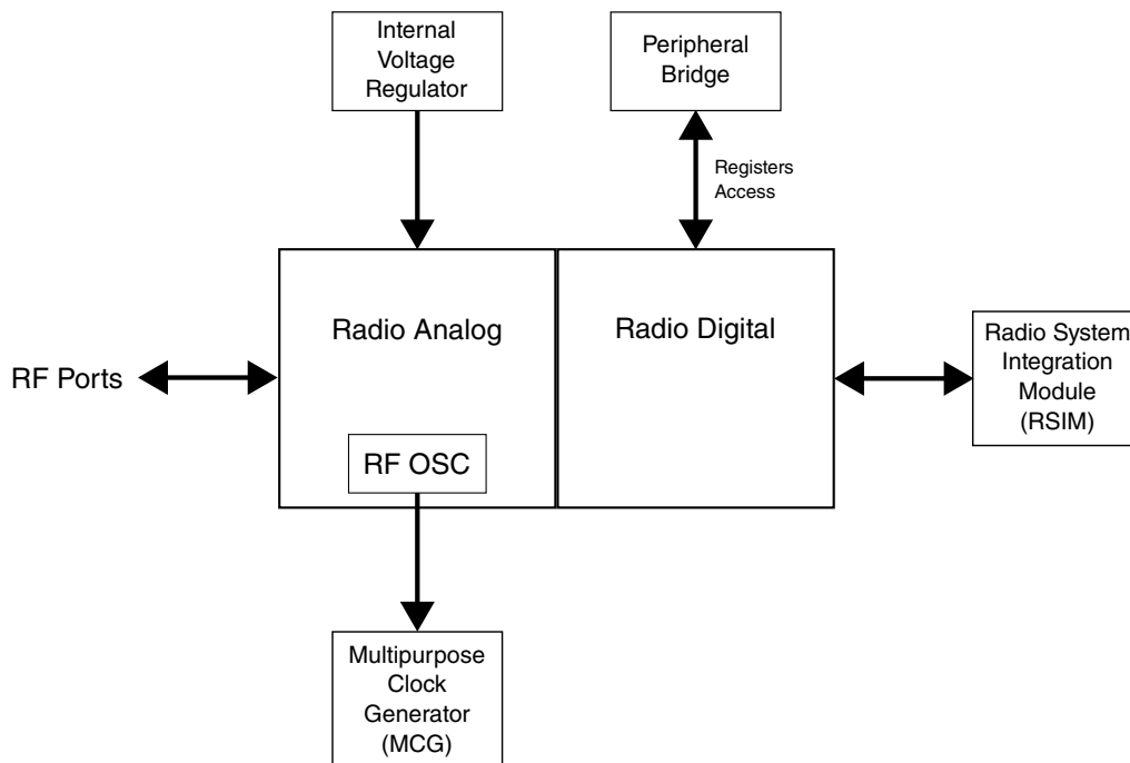
Figure 3-32. Radio configuration
