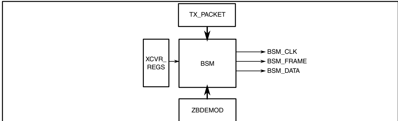
Figure 45-99. Block diagram
