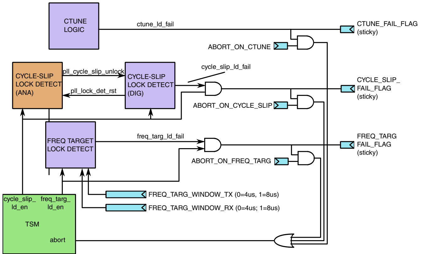
Figure 45-51. PLL UNLOCK MONITORING AND ABORT LOGIC
