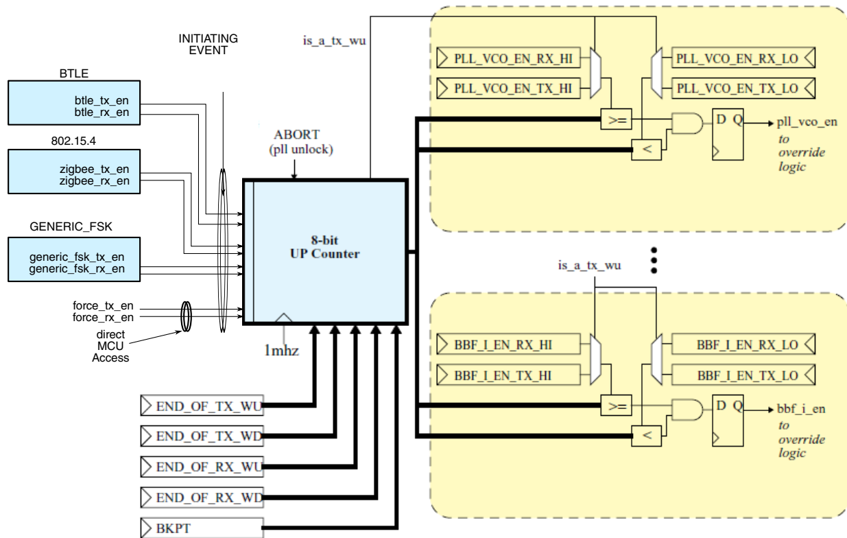
Figure 45-50. 2.4GHZ RADIO TSM BLOCK DIAGRAM
