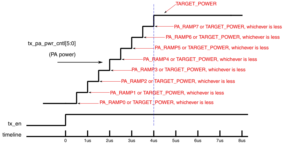
Figure 45-57. PA RAMP UP(4us)
