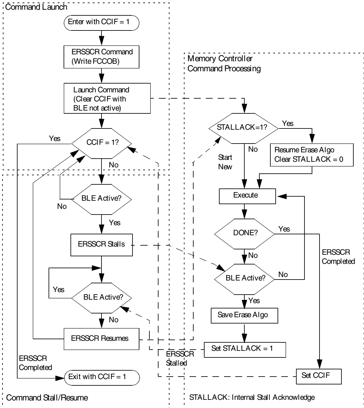
Figure 28-7. BLE Active Impact on Erase Flash Sector Operation
