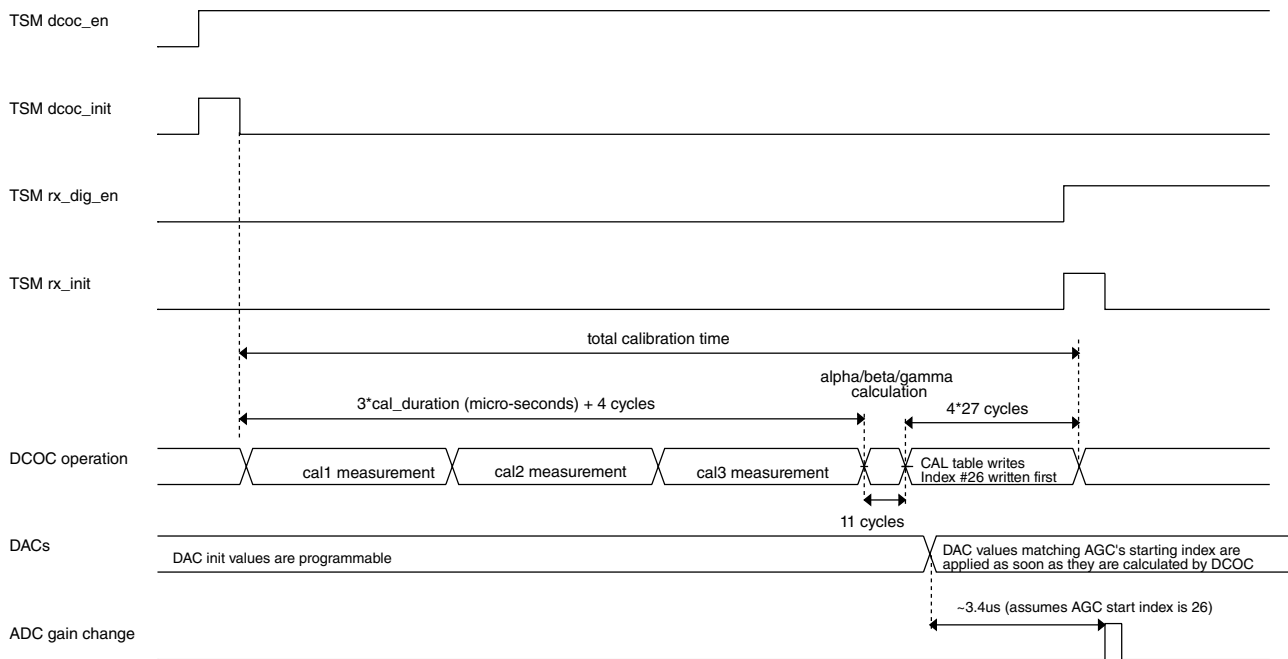
Figure 45-34. DCOC Calibration Timing Diagram
