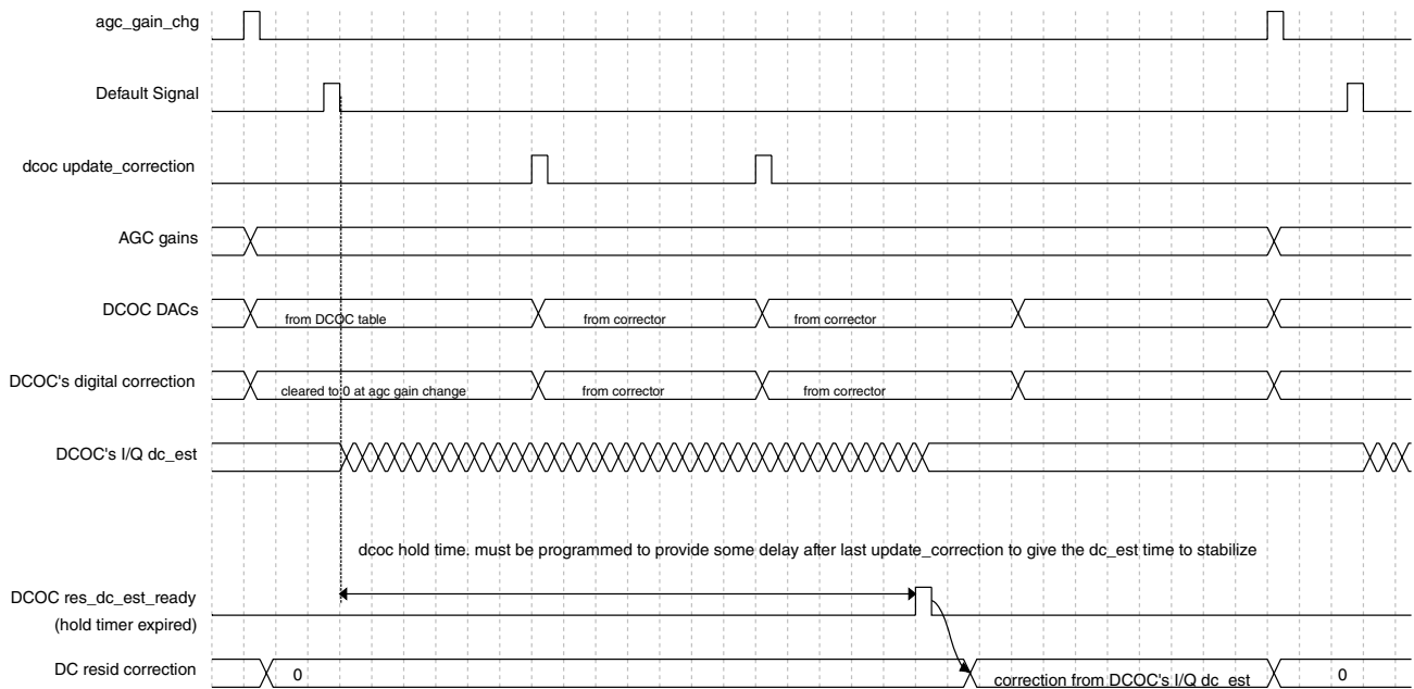
Figure 45-42. DC residual mode 3 timing
