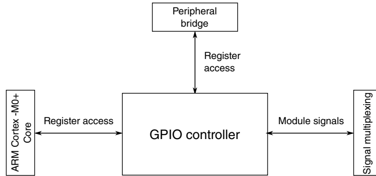
Figure 3-40. GPIO configuration
