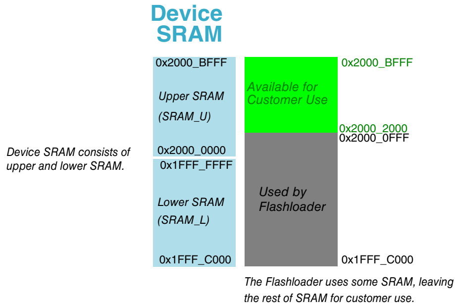
Figure 7-1. Kinetis Flashloader RAM Memory Map
