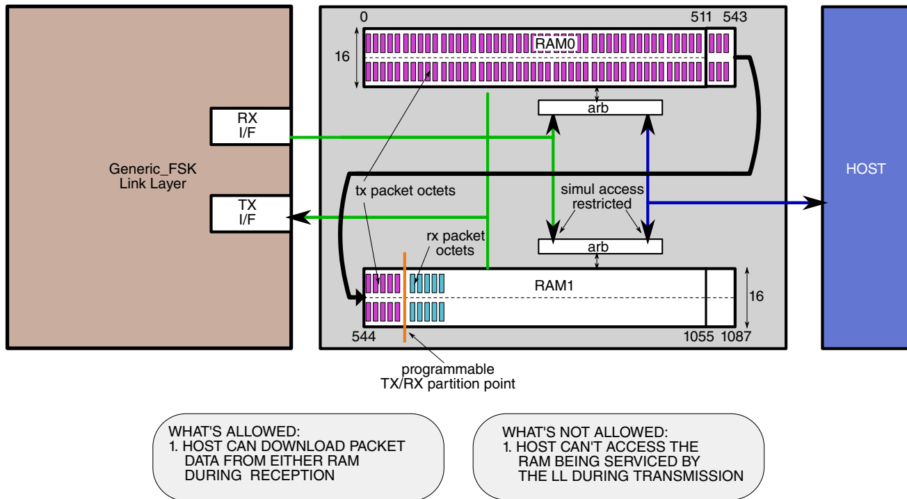
Figure 45-122. RAM ALLOCATIONS FOR GENERIC_FSK
