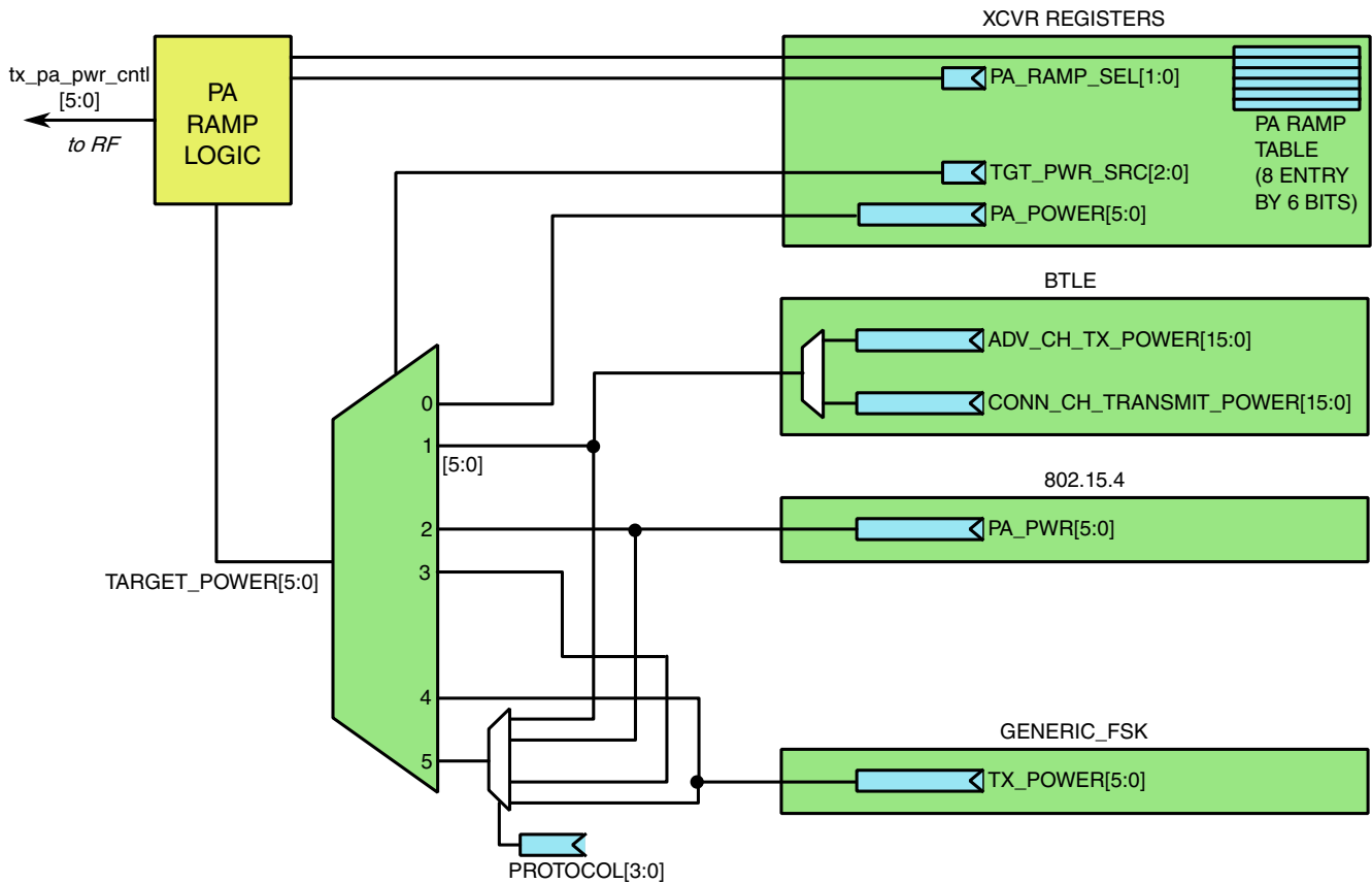
Figure 45-55. PA Target Power Selection
