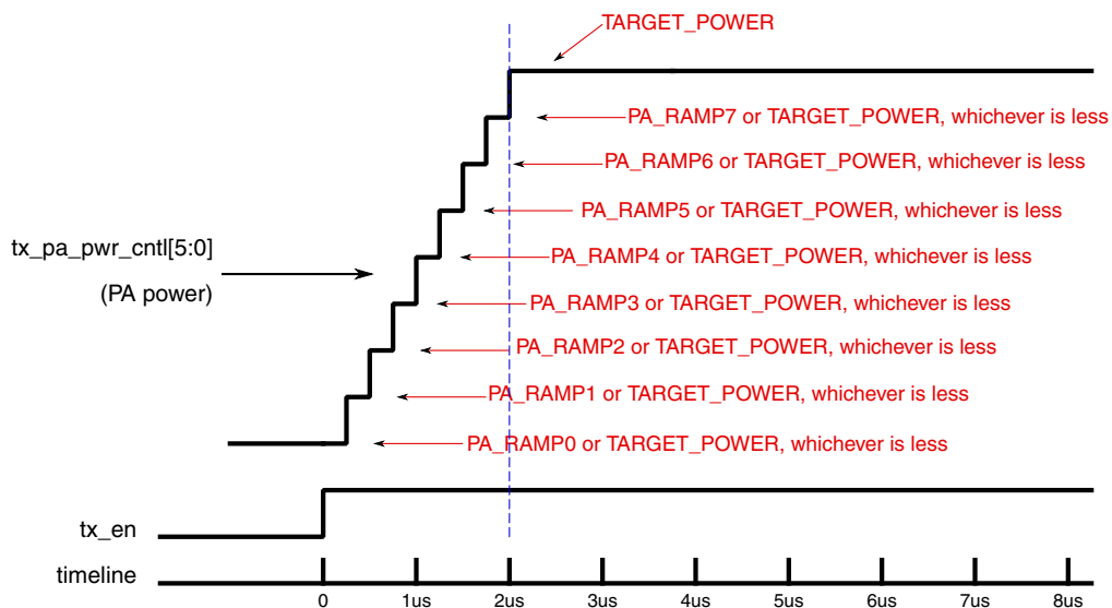
Figure 45-56. PA RAMP UP(2us)
