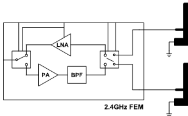
Figure 45-91. FEM Block Diagram
