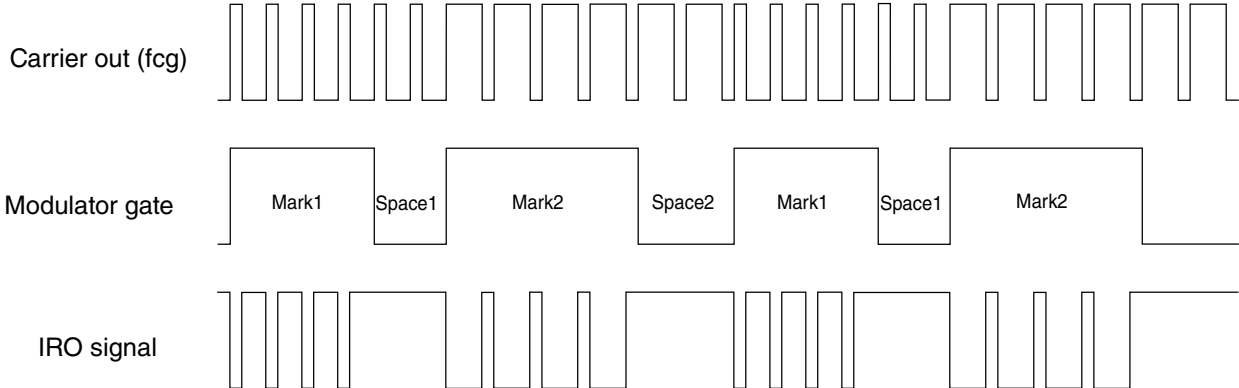
Figure 40-6. Example: CMT output in FSK mode
