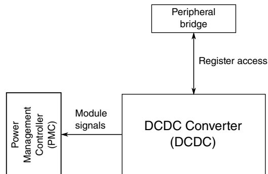
Figure 3-7. DCDC configuration
