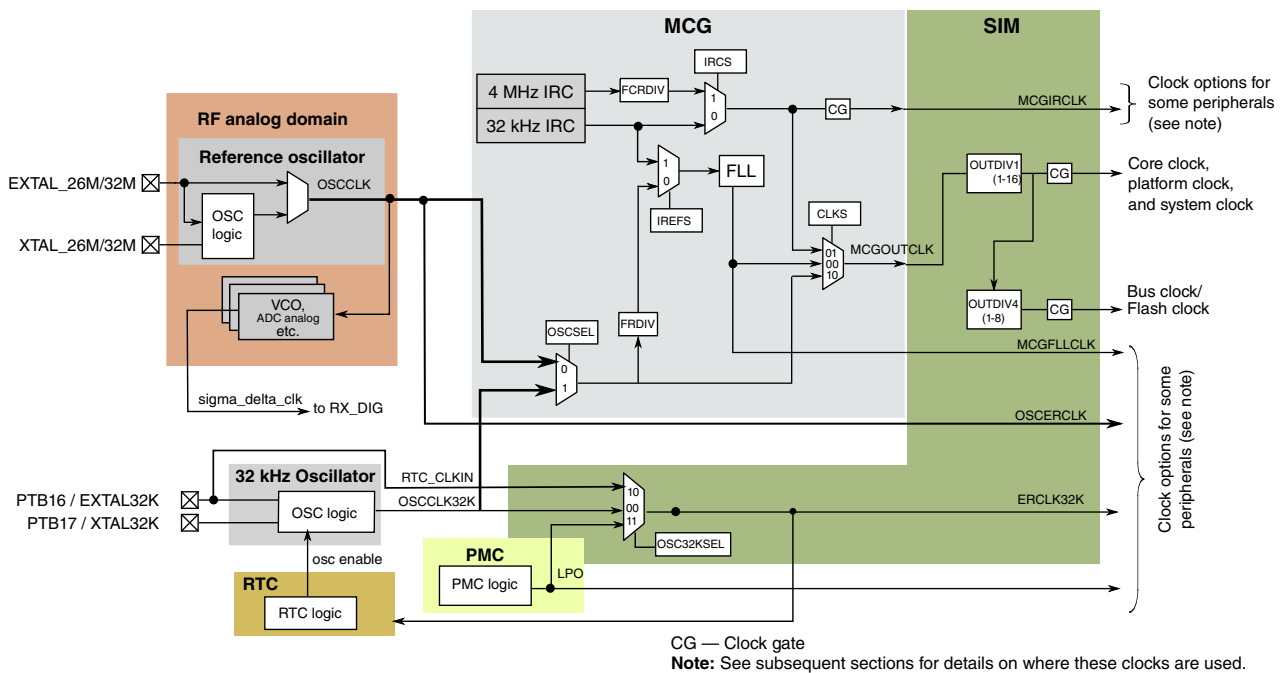
Figure 5-1. Clocking diagram
