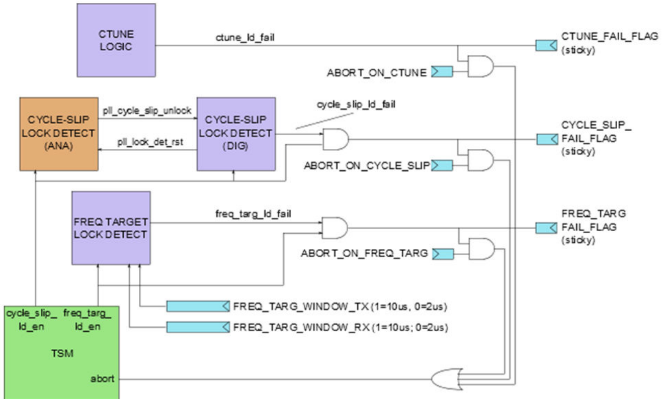
Figure 45-16. PLL Lock Detect Block Diagram
