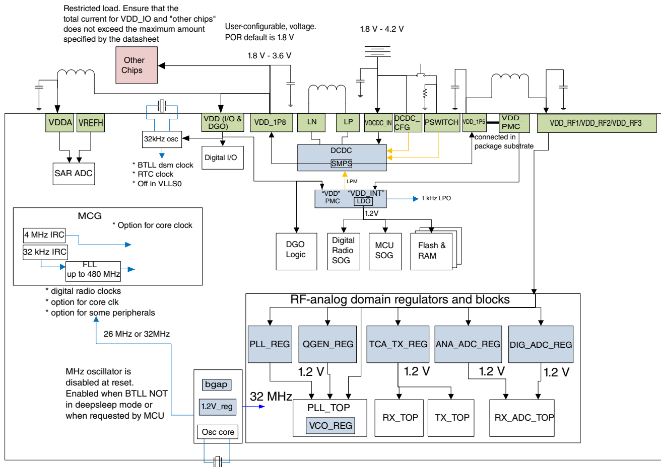
Figure 3-8. Buck Power Tree
