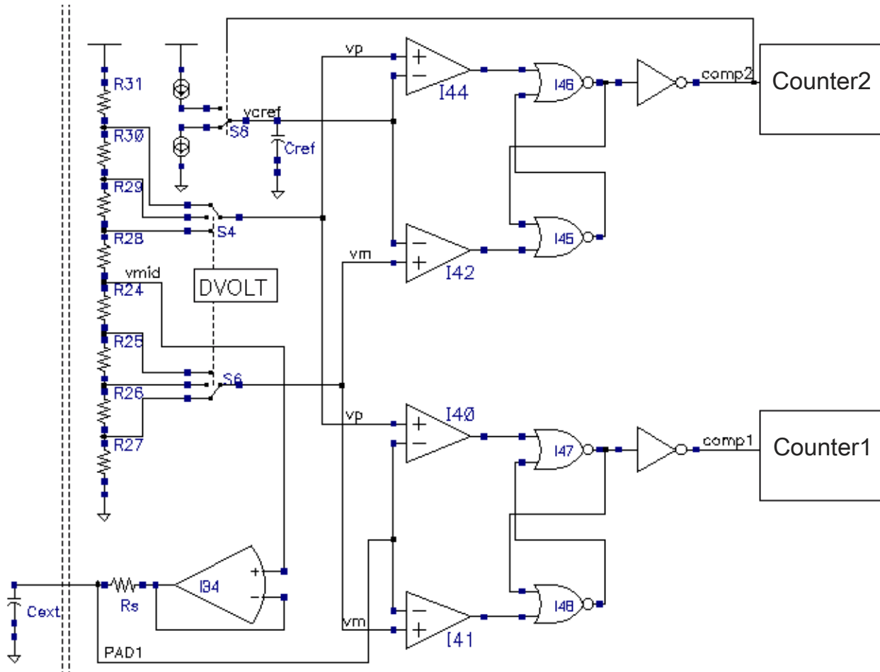
Figure 42-5. TSI circuit in noise detection mode
