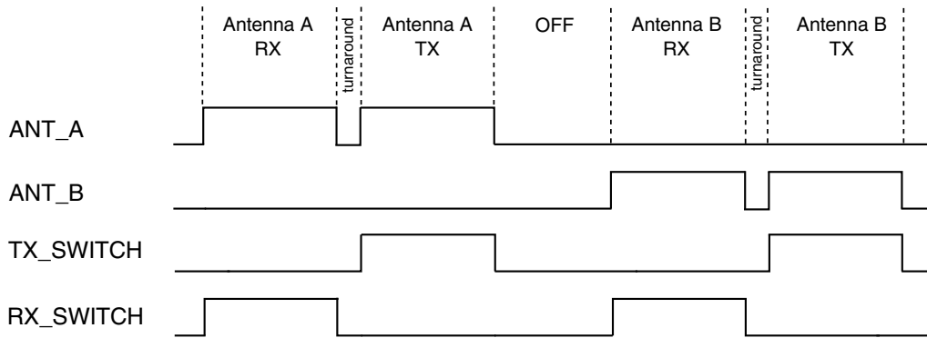
Figure 45-94. FAD Dual Mode Timing
