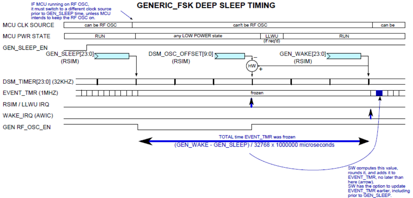
Figure 45-132. GENERIC FSK Deep Sleep Mode Timing
