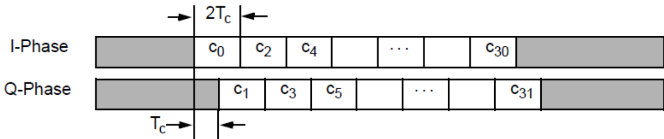
Figure 70—O-QPSK chip offsets
