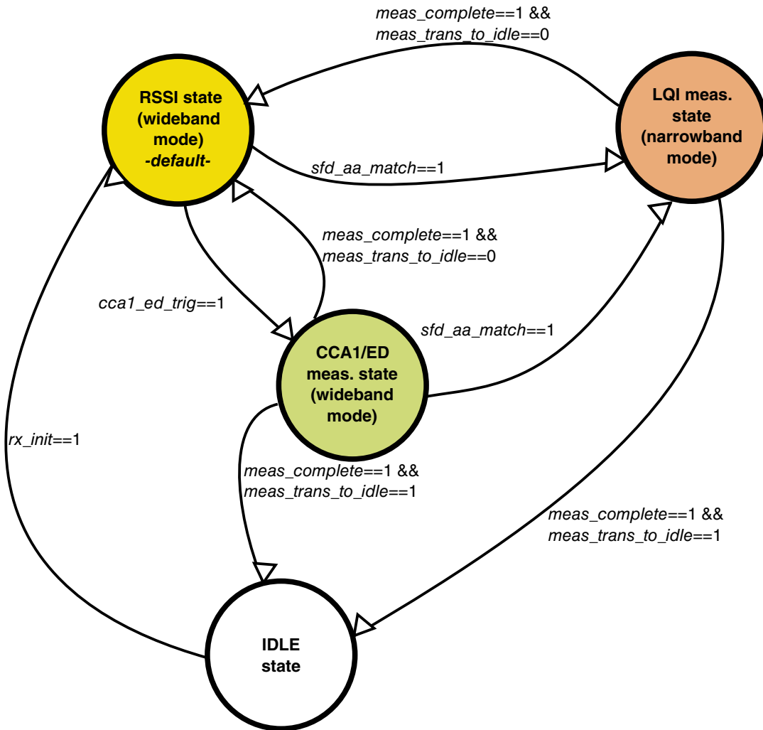
Figure 45-26. Module state machine
