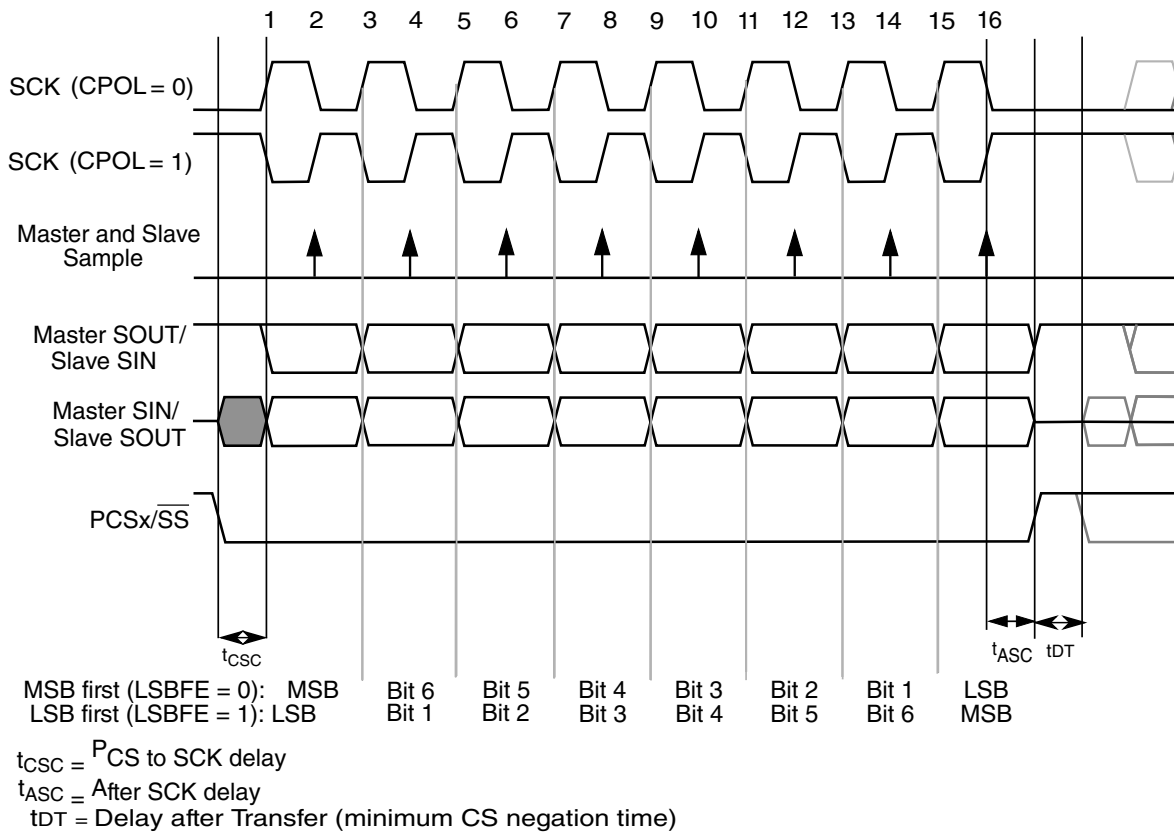
Figure 37-6. Module transfer timing diagram (MTFE=0, CPHA=1, FMSZ=8)
