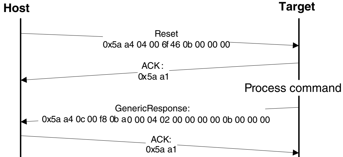
Figure 7-19. Protocol Sequence for Reset Command
