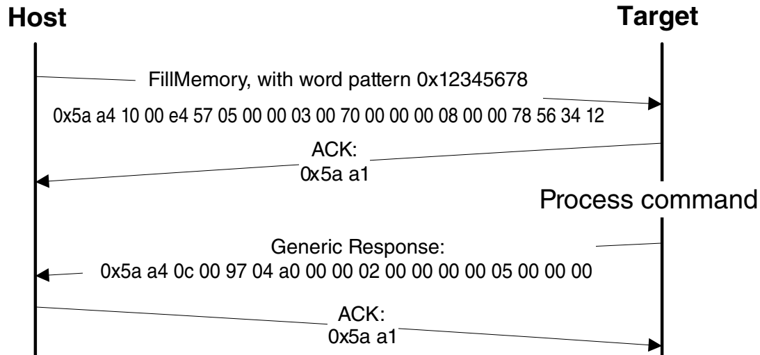
Figure 7-13. Protocol Sequence for FillMemory Command
