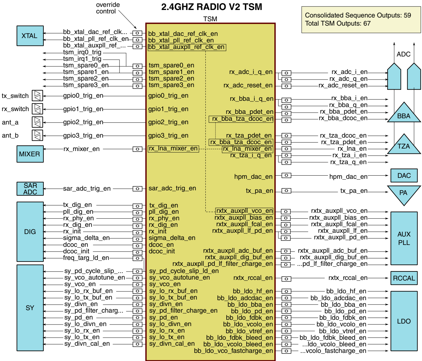
Figure 45-49. 2.4GHZ RADIO TSM
