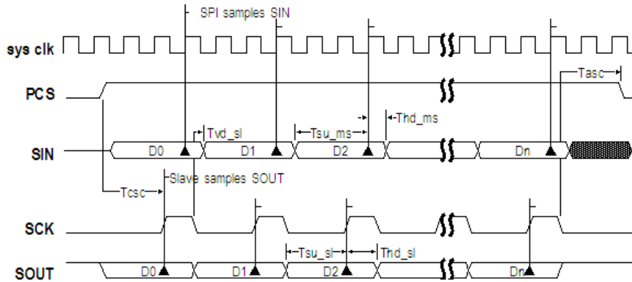
Figure 37-9. SPI Modified Transfer Format (MTFE=1, CPHA=0, f_{sck} = f_{sys}/3 )
