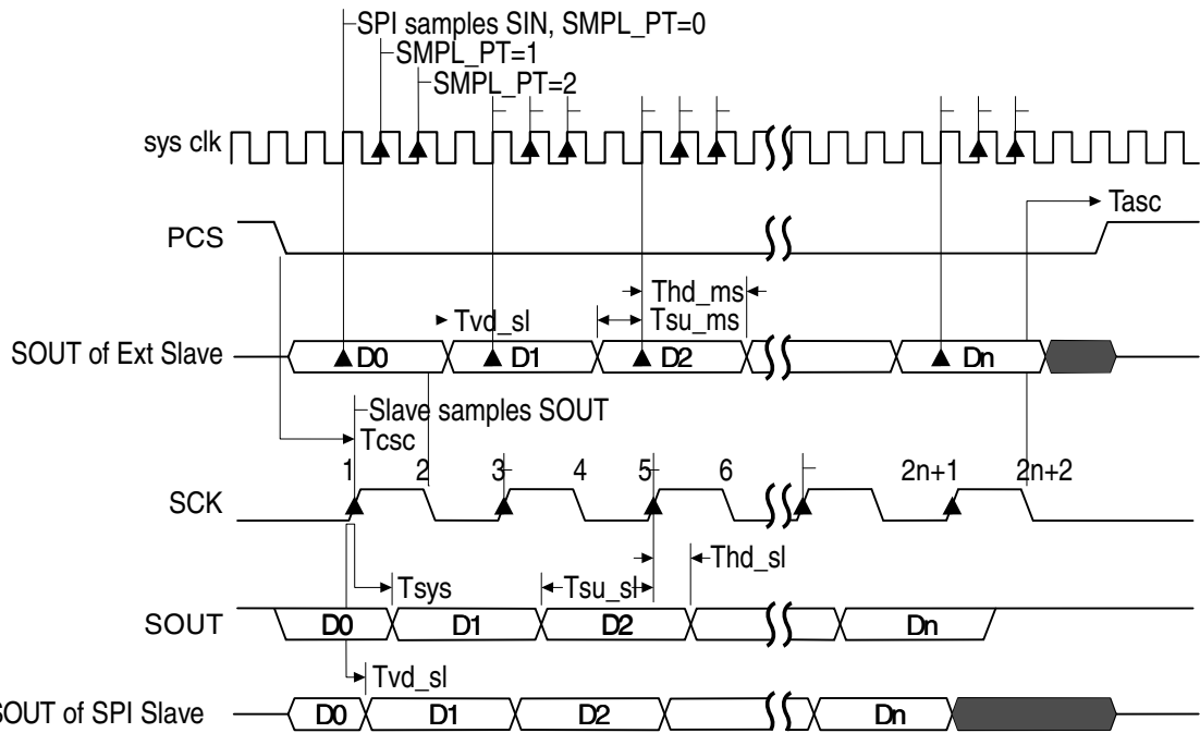
Figure 37-12. SPI Modified Transfer Format (MTFE=1, CPHA=1, f_{sck} = f_{sys}/4 )
