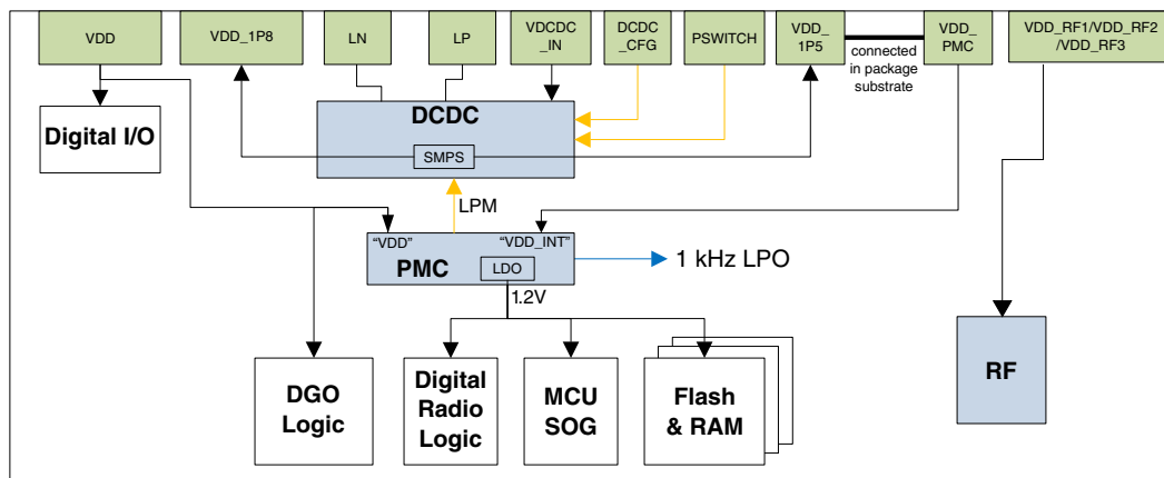
Figure 15-1. DCDC block Diagram
