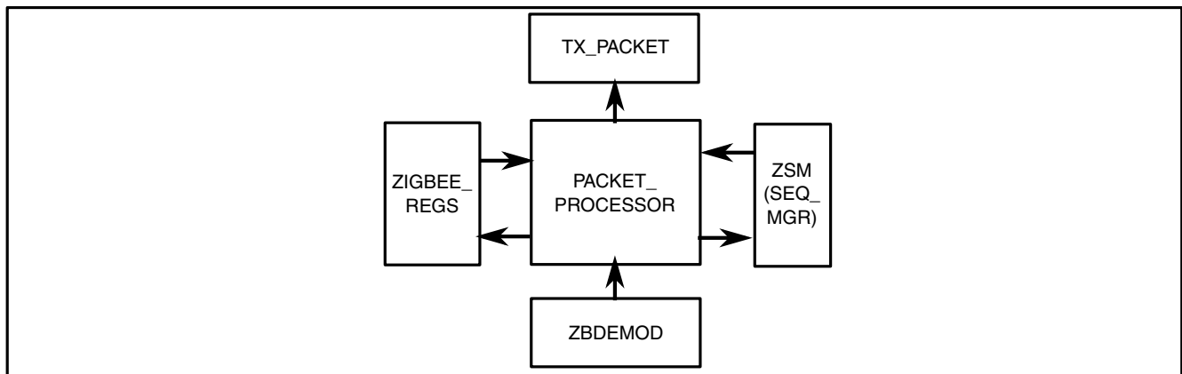
Figure 45-69. Block diagram
