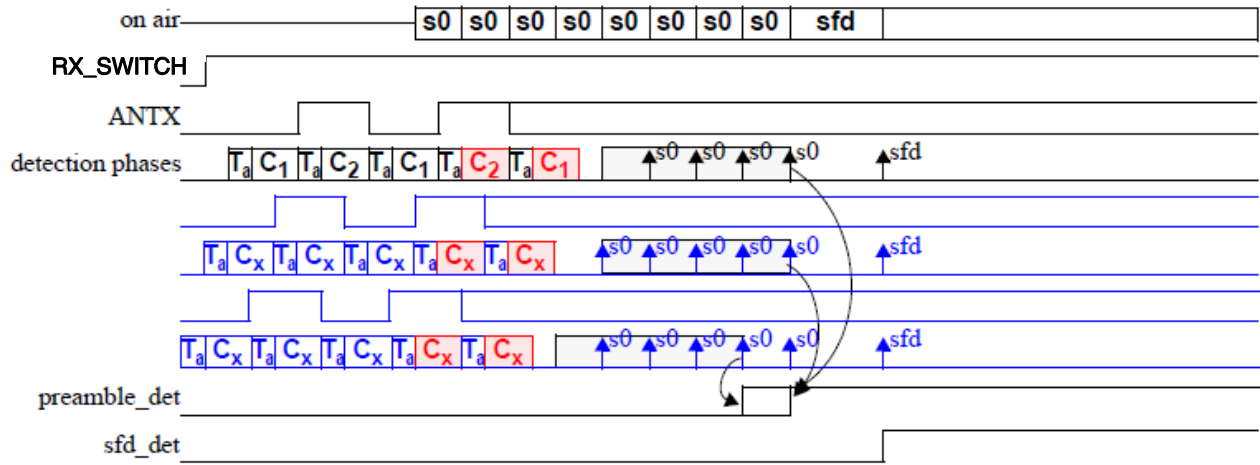
Figure 45-88. FAD Switching
