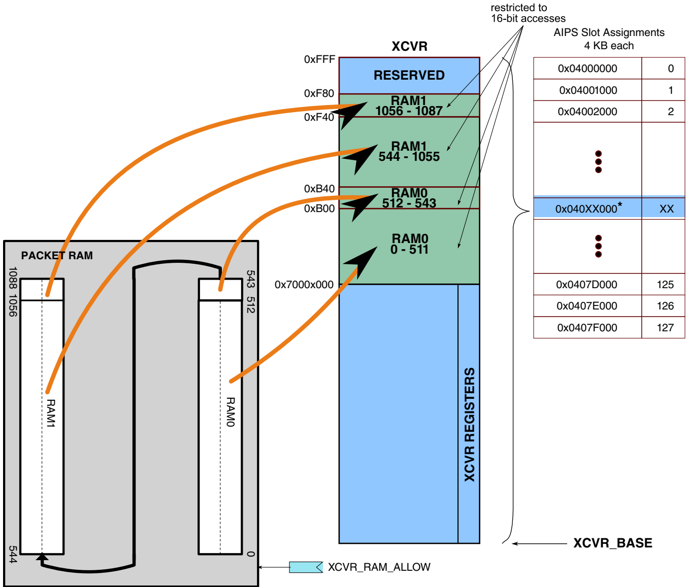
Figure 45-65. Packet RAM Memory Mapping in XCVR Space
