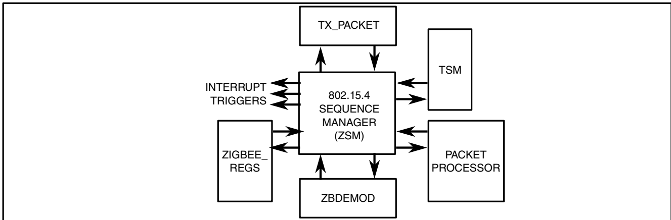
Figure 45-78. Block diagram
