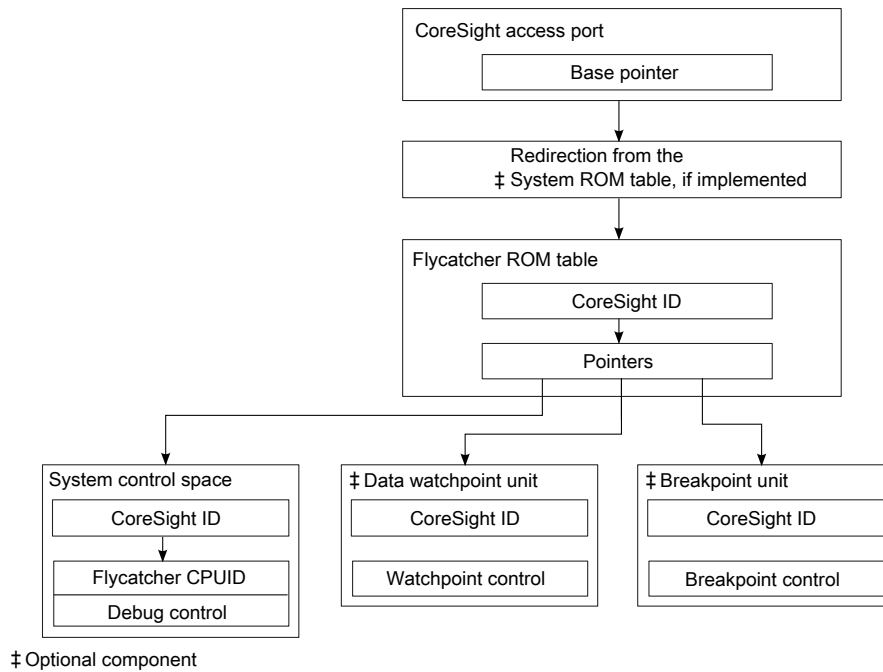
Figure 20-3. CoreSight discovery process
