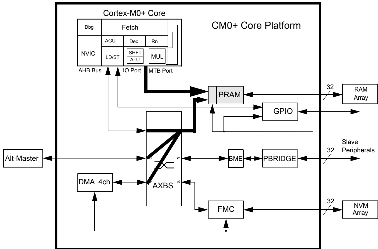
Figure 20-1. Generic Cortex-M0+ core platform block diagram
