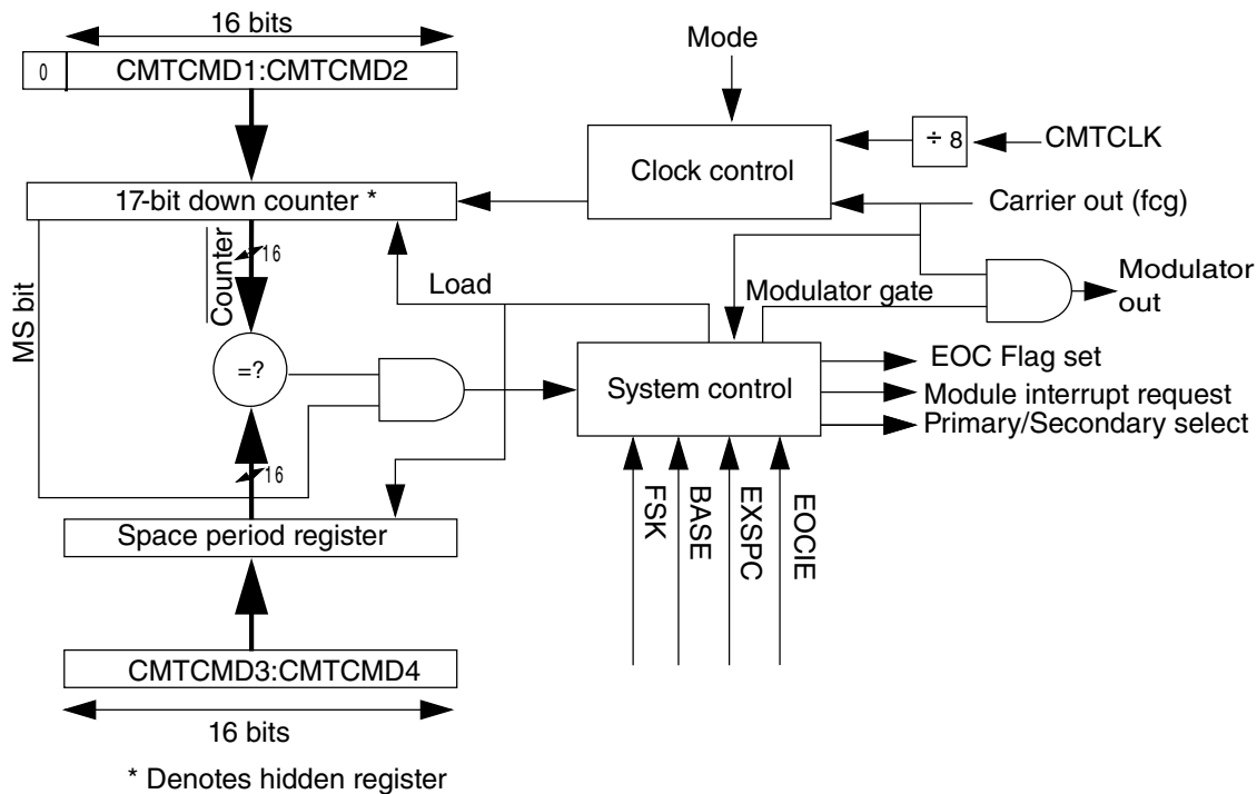
Figure 40-4. Modulator block diagram
