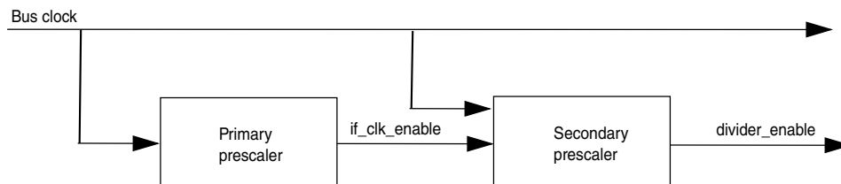
Figure 40-2. Clock divider block diagram
