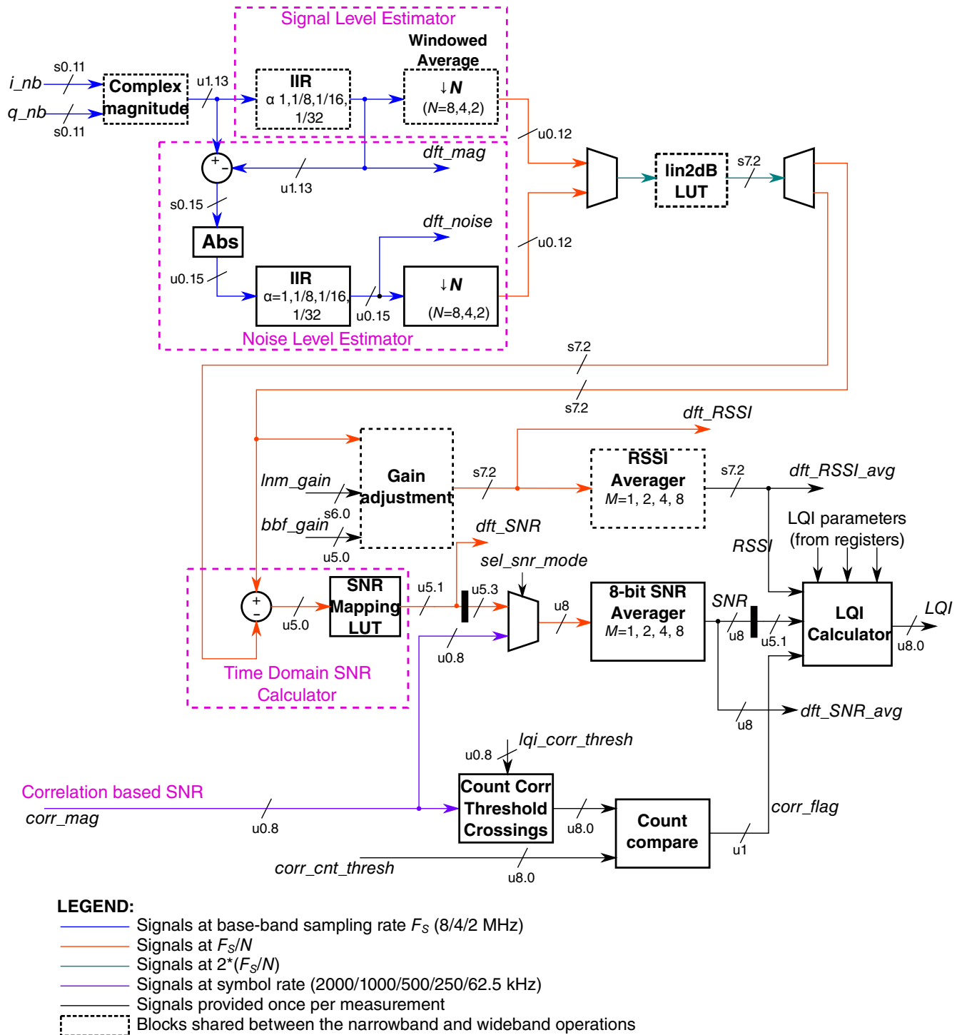
Figure 45-28. Block diagram instantiated for narrowband mode
