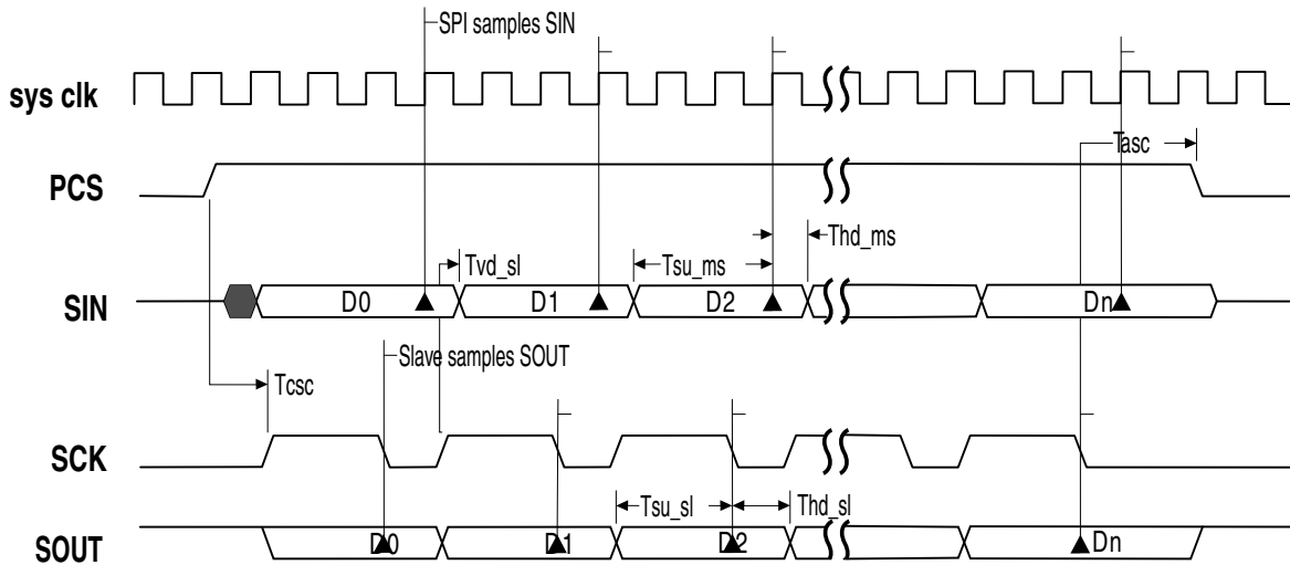
Figure 37-11. SPI Modified Transfer Format (MTFE=1, CPHA=1, f_{sck} = f_{sys}/3 )
