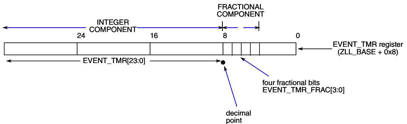
Figure 45-80. Event Timer Integer and Fractional Components
