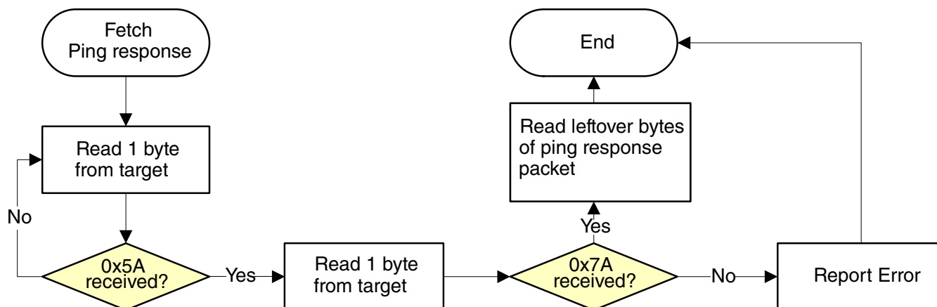
Figure 7-20. Host reads ping response from target via I2C
