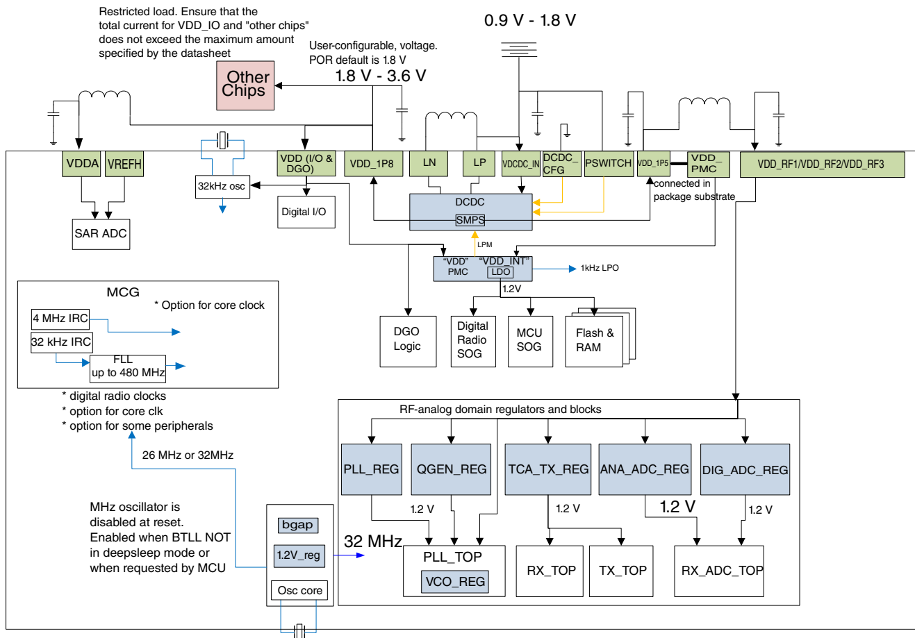
Figure 3-9. Boost Power Tree
