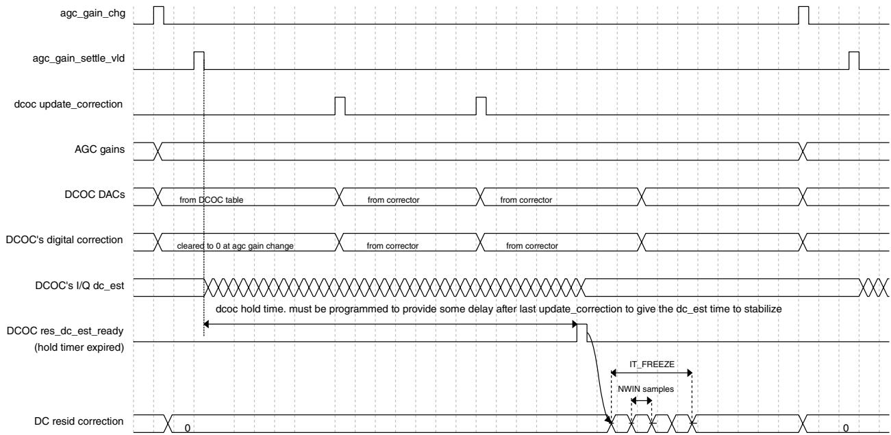
Figure 45-41. DC residual mode 2 timing
