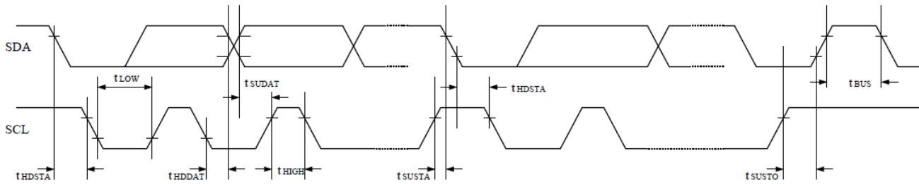
Figure 11. I2C Timing
