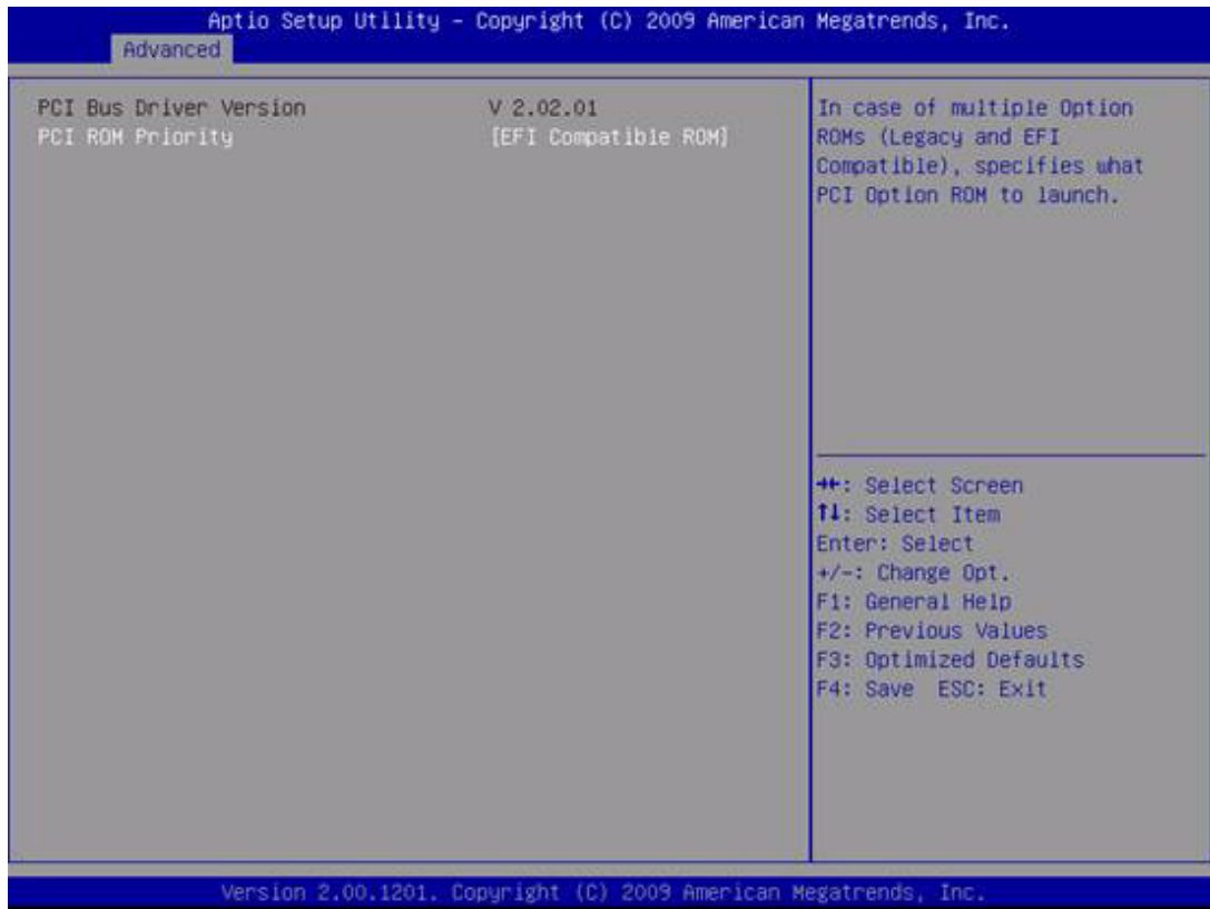
Figure 3.4 PCI Configuration
