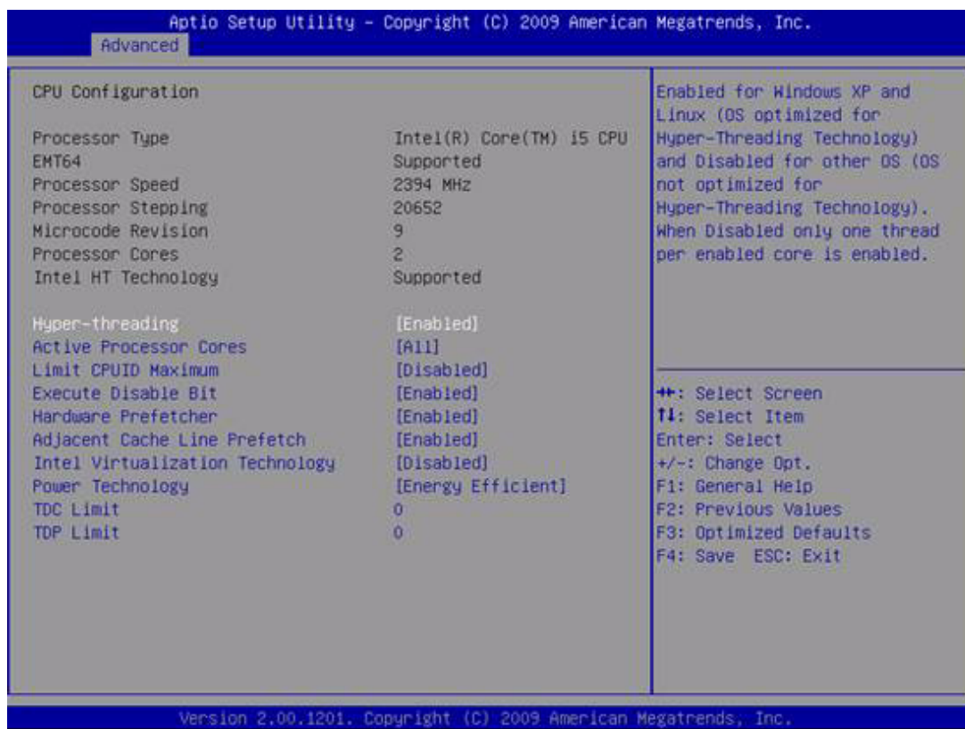
Figure 3.6 CPU Configuration
