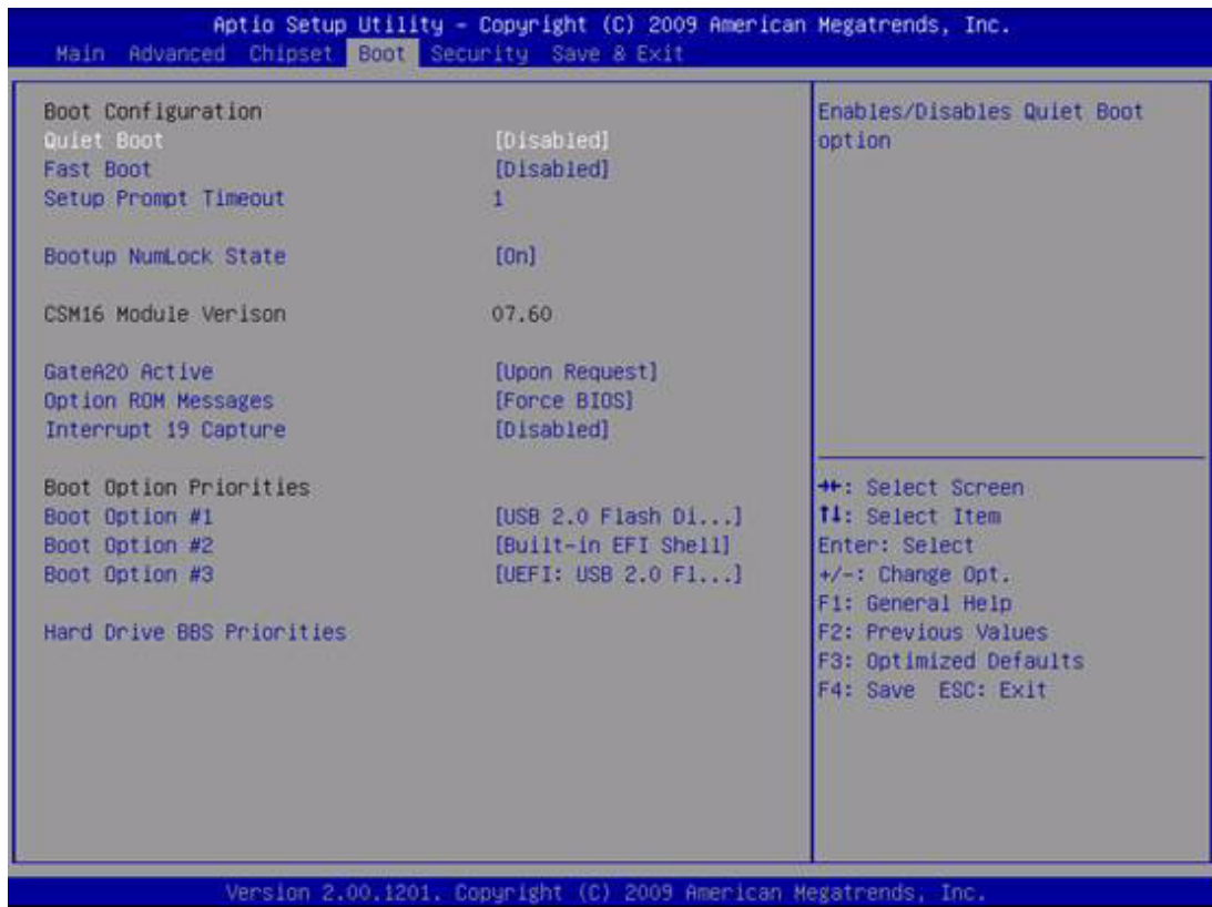
Figure 3.17 Boot Configuration
