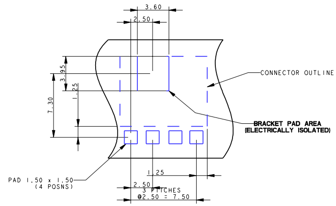
BOARD LAYOUT
