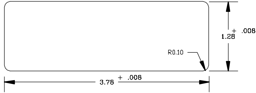
PANEL CUT-OUT
