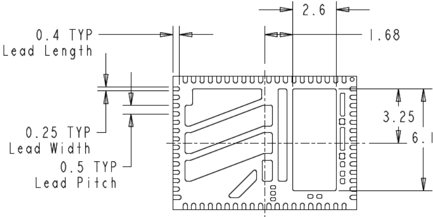
Figure 13: EN6360QA Package Dimensions (Bottom View)
