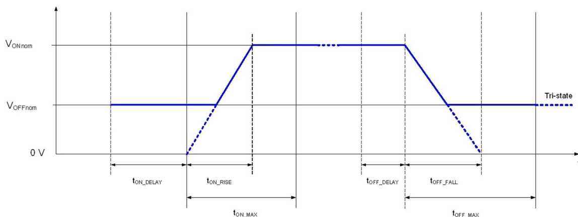
Figure 7: Power Sequencing With Non-Zero Off Voltage
