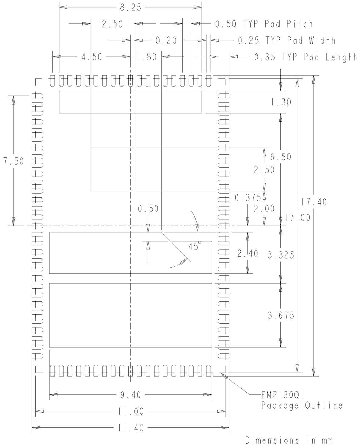
Figure 20: Recommended PCB Footprint
