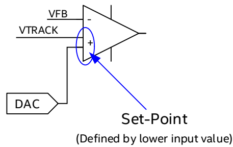
Figure 9: VTRACK Circuitry
