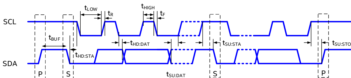
Figure 14: PMBus Timing Diagram
