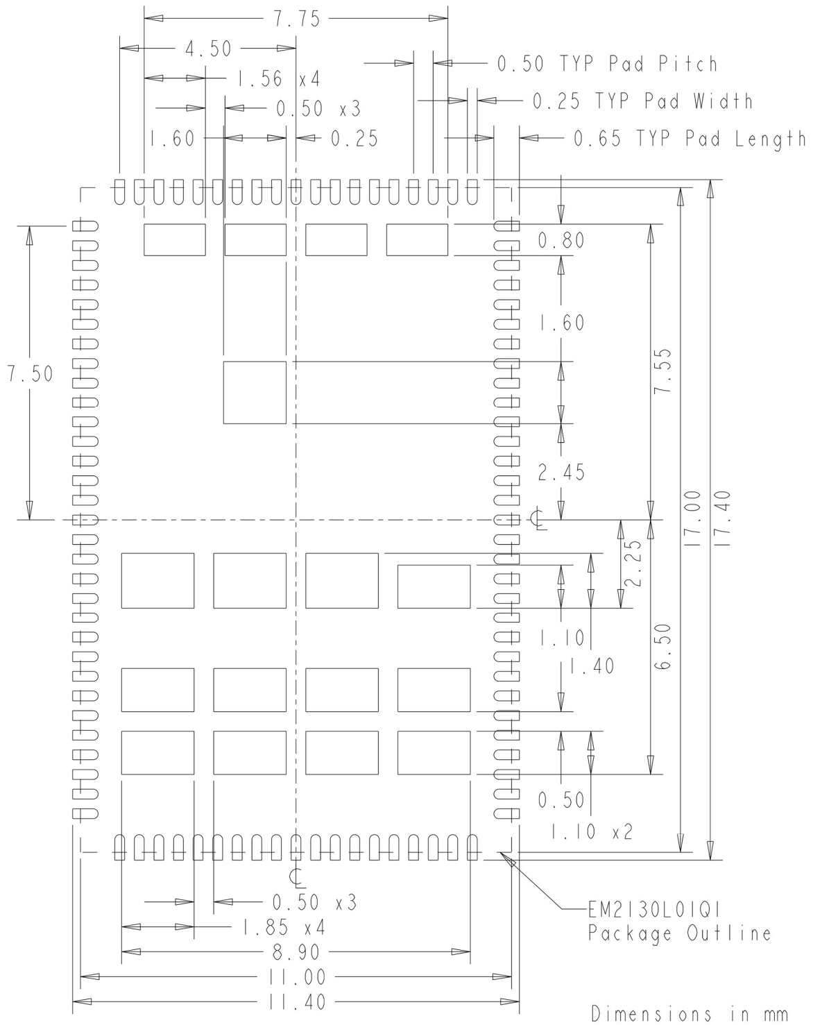
Figure 21: Recommended Solder Stencil Aperture
