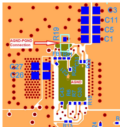
Figure 18: Backside Decoupling
