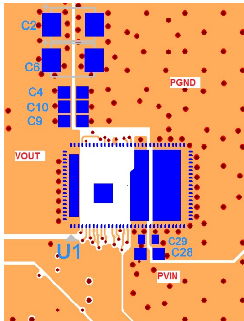
Figure 16: Top Layer Layout With Critical Components Only
