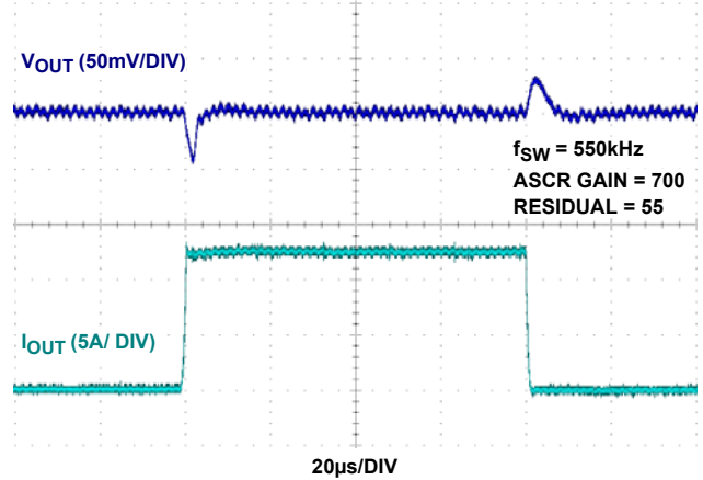
FIGURE 10. 1V TRANSIENT RESPONSE
