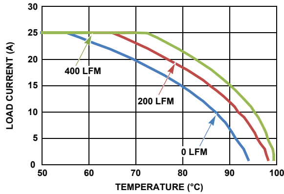
FIGURE 24. 12V_{\text{IN}} TO 5V_{\text{OUT}} , 727kHz
