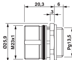
Dimensional drawing
