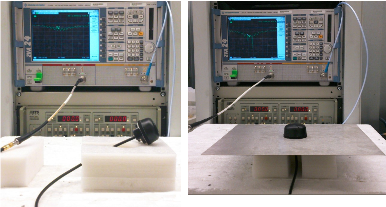
Figure 1. Return loss measurements.
