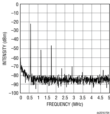
Figure 4. Conducted V OUT Noise Spectrum Using HP 4395A Spectrum Analyzer and 41800A Active Probe. V IN = 24V and V OUT = 12V at 3A
