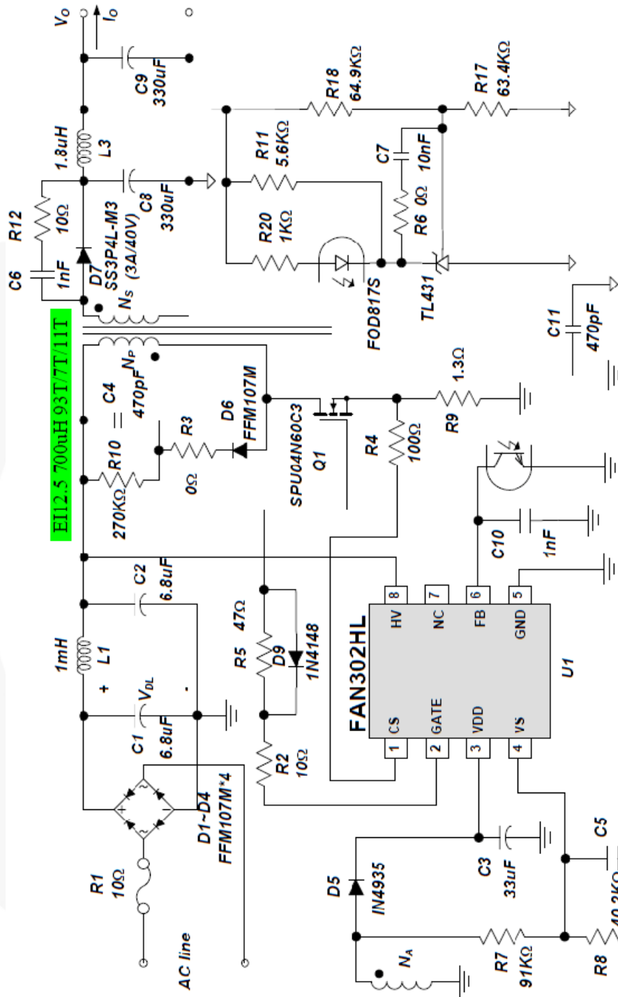
Figure 35. Circuit Schematic
