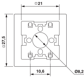
Dimensional drawing
