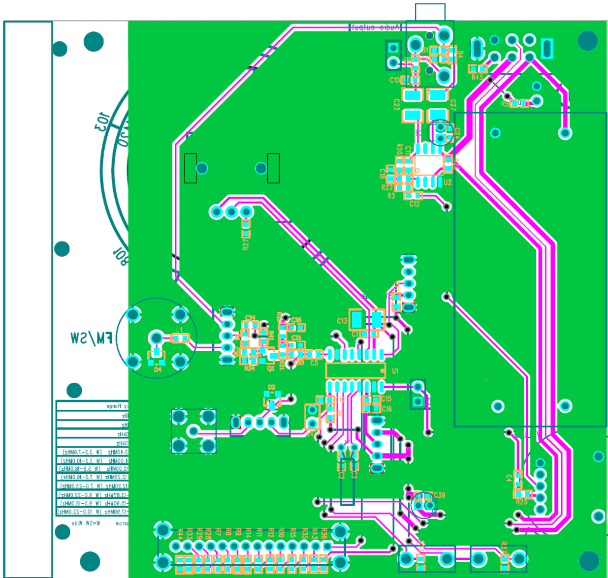
Figure 4. Si4825-DEMO Board Gerber Rev 1.1
