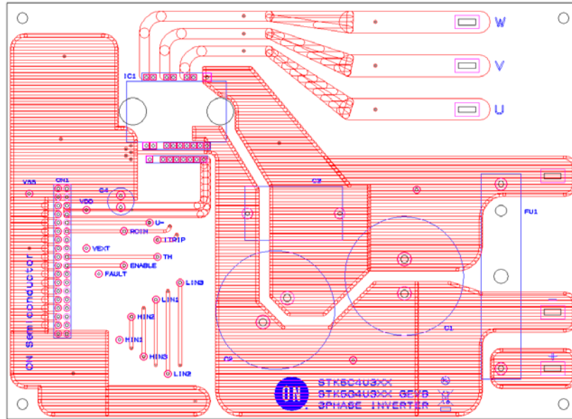
Figure 6. Layout – Surface
